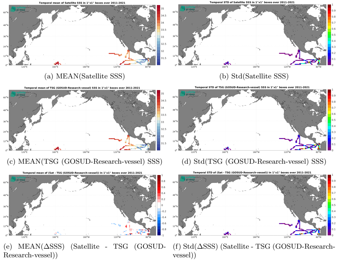
Figure 6: Temporal mean (left) and Std (right) of SSS from SMAP SSS L4 OI v2 - 7 Days (ESR) (top), TSG (GOSUD-Research-vessel) (middle), and of \Delta SSS (Satellite - TSG (GOSUD-Research-vessel)). Only match-up pairs are used to generate these maps.
