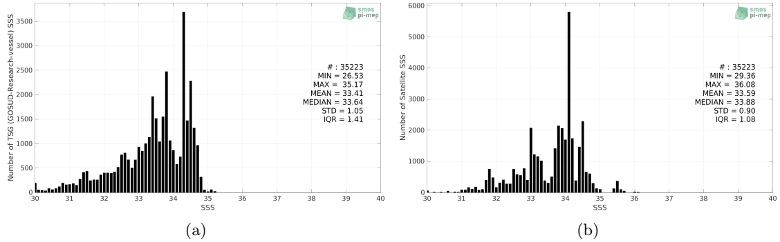
Figure 2: Histograms of SSS from TSG (GOSUD-Research-vessel) (a) and SMAP SSS L4 OI v2 - 7 Days (ESR) (b) considering all match-up pairs per bins of 0.1 over the North Pacific Ocean Pi-MEP region and for the full satellite product period.
