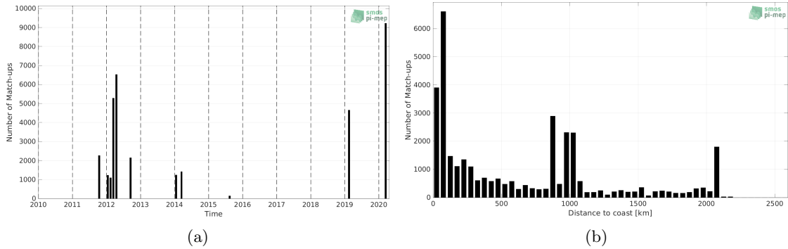
Figure 1: Number of match-ups between TSG (GOSUD-Research-vessel) and SMAP SSS L4 OI v2 - 7 Days (ESR) SSS as a function of time (a) and as function of the distance to coast (b) over the North Pacific Ocean Pi-MEP region and for the full satellite product period.
