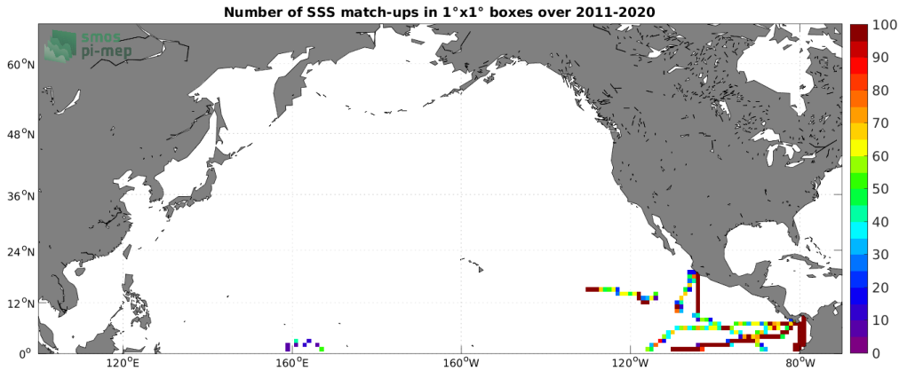
Figure 4: Number of SSS match-ups between TSG (GOSUD-Research-vessel) SSS and the SMAP SSS L4 OI v2 - 7 Days (ESR) SSS product for the North Pacific Ocean Pi-MEP region over 1^\circ \times 1^\circ boxes and for the full satellite product period.
