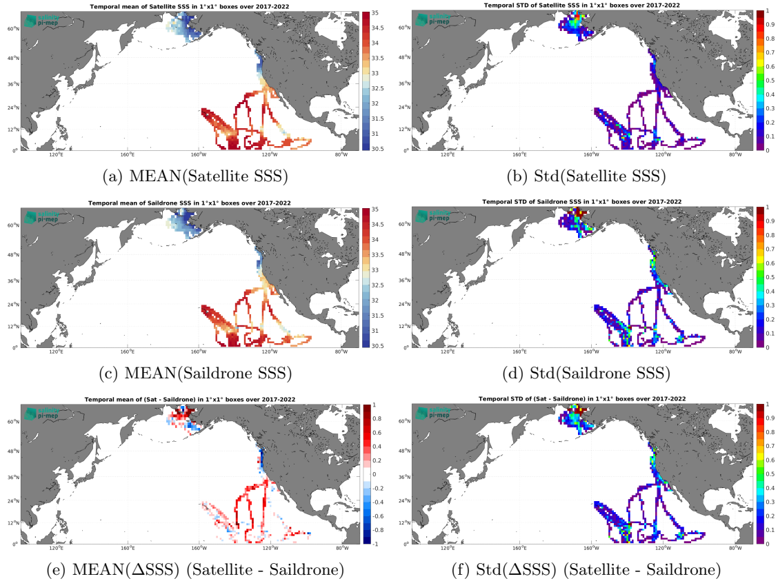
Figure 6: Temporal mean (left) and Std (right) of SSS from SMAP SSS L4 OI v2 - 7 Days (ESR) (top), Sairdrone (middle), and of \Delta\text{SSS} (Satellite - Sairdrone). Only match-up pairs are used to generate these maps.
