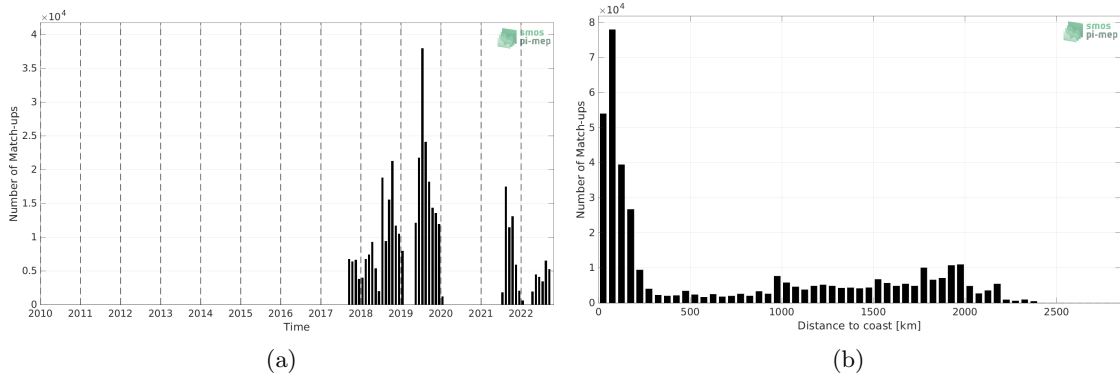
Figure 1: Number of match-ups between Saildrone and SMAP SSS L4 OI v2 - 7 Days (ESR) SSS as a function of time (a) and as function of the distance to coast (b) over the North Pacific Ocean Pi-MEP region and for the full satellite product period.
