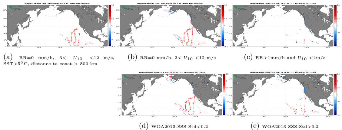
Figure 12: Temporal mean gridded over spatial boxes of size 1^\circ \times 1^\circ of \Delta SSS (SMAP SSS L4 OI v2 - 7 Days (ESR) - Sairdrone) for 5 different subdatasets corresponding to:RR=0 mm/h, 3 < U_{10} < 12 m/s, SST > 5^\circ C , distance to coast > 800 km (a), RR=0 mm/h, 3 < U_{10} < 12 m/s (b), RR >1 mm/h and U_{10} < 4 m/s (c), WOA2013 SSS Std <0.2 (d), WOA2013 SSS Std >0.2 (e).
