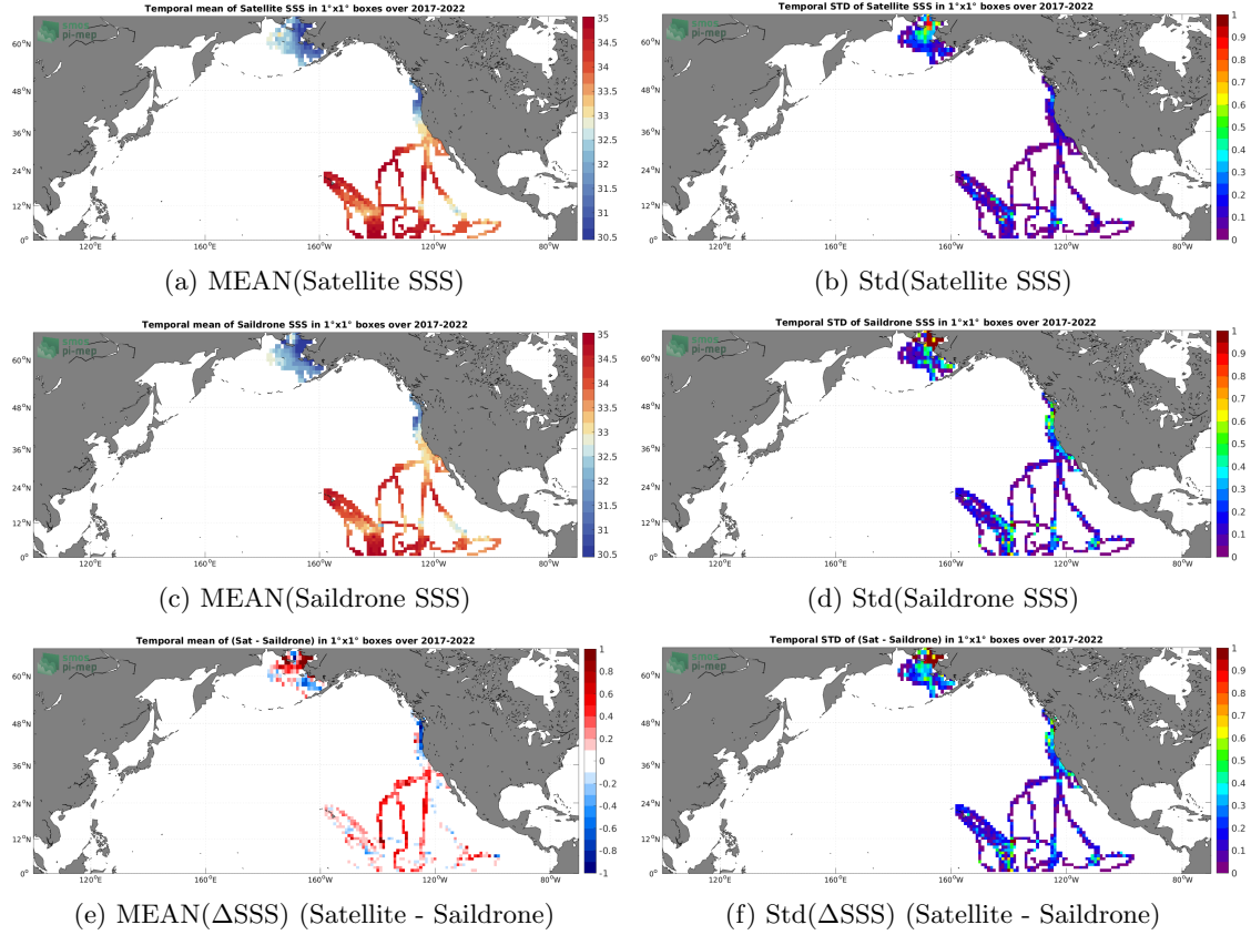
Figure 6: Temporal mean (left) and Std (right) of SSS from SMAP SSS L4 OI v2 - 7 Days (ESR) (top), Saildrone (middle), and of \Delta\text{SSS} (Satellite - Saildrone). Only match-up pairs are used to generate these maps.
