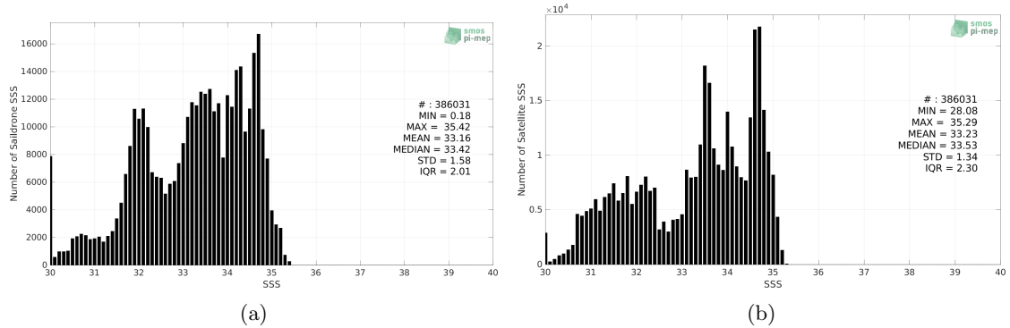
Figure 2: Histograms of SSS from Saildrone (a) and SMAP SSS L4 OI v2 - 7 Days (ESR) (b) considering all match-up pairs per bins of 0.1 over the North Pacific Ocean Pi-MEP region and for the full satellite product period.
