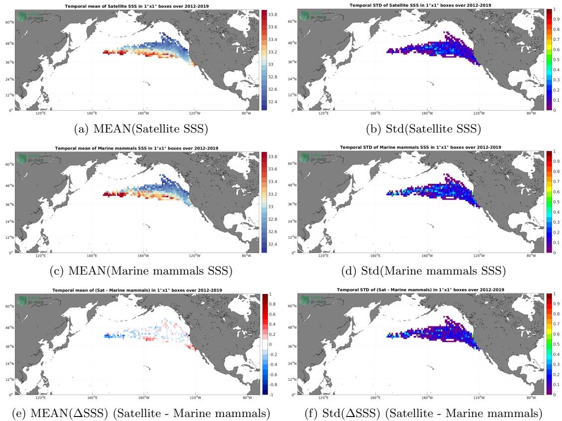
Figure 6: Temporal mean (left) and Std (right) of SSS from SMAP SSS L4 OI v2 - 7 Days (ESR) (top), Marine mammals (middle), and of \Delta SSS (Satellite - Marine mammals). Only match-up pairs are used to generate these maps.
