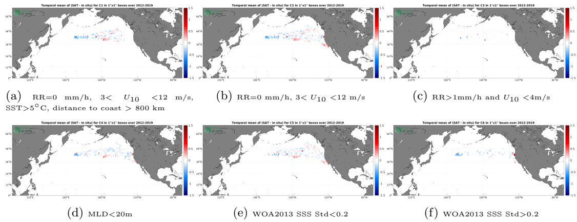
Figure 12: Temporal mean gridded over spatial boxes of size 1^\circ \times 1^\circ of \Delta SSS (SMAP SSS L4 OI v2 - 7 Days (ESR) - Marine mammals) for 6 different subdatasets corresponding to:RR=0 mm/h, 3 < U_{10} < 12 m/s, SST >5^\circ C, distance to coast > 800 km (a), RR=0 mm/h, 3 < U_{10} < 12 m/s (b), RR >1 mm/h and U_{10} < 4 m/s (c),MLD <20 m (d),WOA2013 SSS Std <0.2 (e),WOA2013 SSS Std >0.2 (f).
