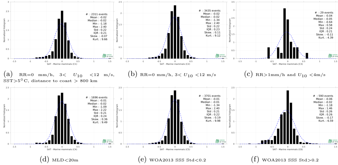
Figure 13: Normalized histogram of \Delta\text{SSS} (SMAP SSS L4 OI v2 - 7 Days (ESR) - Marine mammals) for 6 different subdatasets corresponding to: RR=0 mm/h, 3 < U_{10} < 12 m/s, SST>5°C, distance to coast > 800 km (a), RR=0 mm/h, 3 < U_{10} < 12 m/s (b), RR>1mm/h and U_{10} < 4 m/s (c), MLD<20m (d), WOA2013 SSS Std<0.2 (e), WOA2013 SSS Std>0.2 (f).
