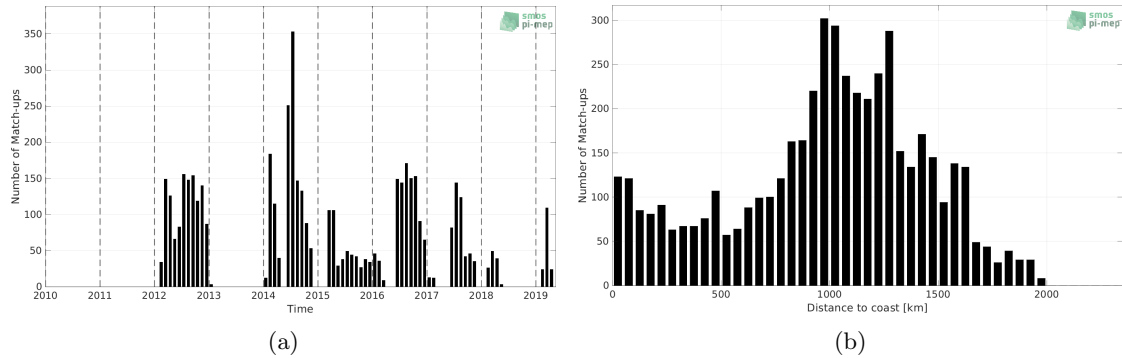
Figure 1: Number of match-ups between Marine mammals and SMAP SSS L4 OI v2 - 7 Days (ESR) SSS as a function of time (a) and as function of the distance to coast (b) over the North Pacific Ocean Pi-MEP region and for the full satellite product period.
