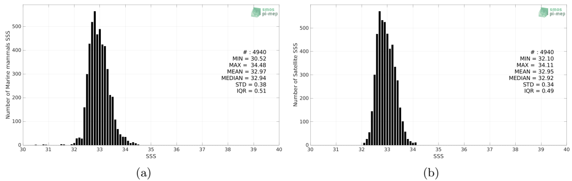
Figure 2: Histograms of SSS from Marine mammals (a) and SMAP SSS L4 OI v2 - 7 Days (ESR) (b) considering all match-up pairs per bins of 0.1 over the North Pacific Ocean Pi-MEP region and for the full satellite product period.
