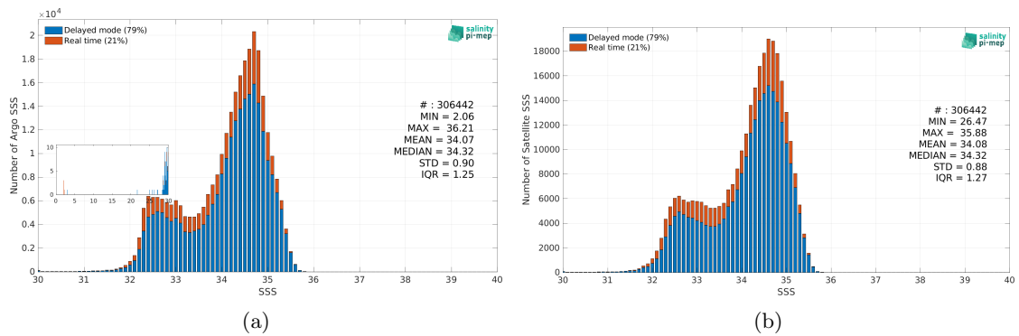
Figure 2: Histograms of SSS from Argo (a) and SMAP SSS L4 OI v2 - 7 Days (ESR) (b) considering all match-up pairs per bins of 0.1 over the North Pacific Ocean Pi-MEP region and for the full satellite product period.
