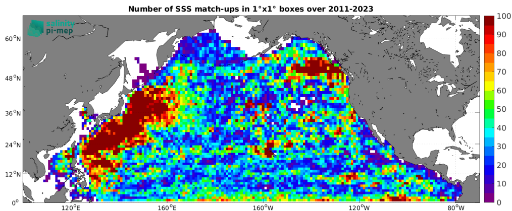
Figure 4: Number of SSS match-ups between Argo SSS and the SMAP SSS L4 OI v2 - 7 Days (ESR) SSS product for the North Pacific Ocean Pi-MEP region over 1^\circ \times 1^\circ boxes and for the full satellite product period.
