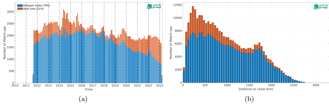
Figure 1: Number of match-ups between Argo and SMAP SSS L4 OI v2 - 7 Days (ESR) SSS as a function of time (a) and as function of the distance to coast (b) over the North Pacific Ocean Pi-MEP region and for the full satellite product period.
