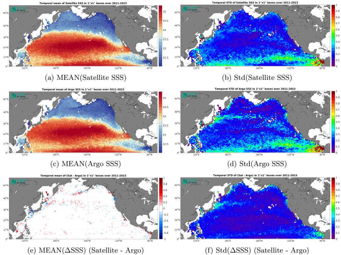
Figure 6: Temporal mean (left) and Std (right) of SSS from SMAP SSS L4 OI v2 - 7 Days (ESR) (top), Argo (middle), and of \Delta SSS (Satellite - Argo). Only match-up pairs are used to generate these maps.
