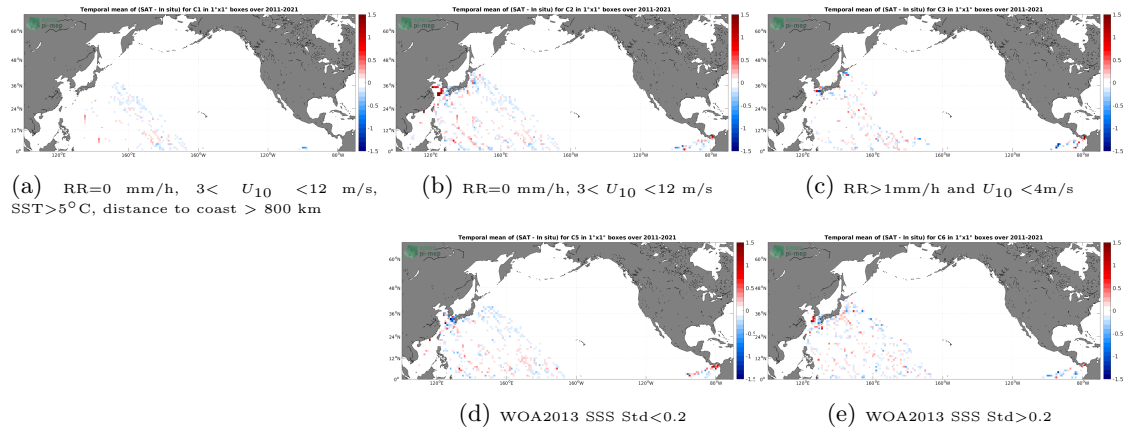
Figure 12: Temporal mean gridded over spatial boxes of size 1^\circ \times 1^\circ of \Delta SSS (SMAP SSS L4 OI v2 - Monthly (IPRC) - TSG (LEGOS-DM)) for 5 different subdatasets corresponding to: RR=0 mm/h, 3 < U_{10} < 12 m/s, SST > 5^\circ C , distance to coast > 800 km (a), RR=0 mm/h, 3 < U_{10} < 12 m/s (b), RR > 1mm/h and U_{10} < 4 m/s (c), WOA2013 SSS Std < 0.2 (d), WOA2013 SSS Std > 0.2 (e).
