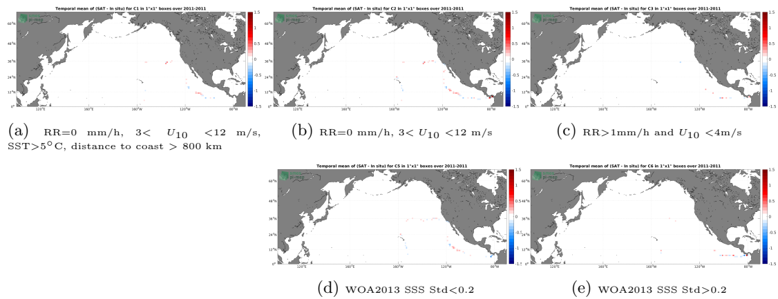
Figure 12: Temporal mean gridded over spatial boxes of size 1^\circ \times 1^\circ of \Delta\text{SSS} (SMAP SSS L4 OI v2 - Monthly (IPRC) - TSG (GOSUD-Sailing-ship)) for 5 different subdatasets corresponding to: RR=0 mm/h, 3 < U_{10} < 12 m/s, SST > 5°C, distance to coast > 800 km (a), RR=0 mm/h, 3 < U_{10} < 12 m/s (b), RR > 1 mm/h and U_{10} < 4 m/s (c), WOA2013 SSS Std < 0.2 (d), WOA2013 SSS Std > 0.2 (e).
