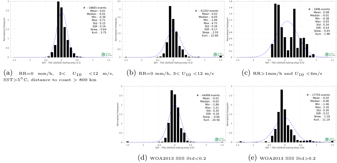
Figure 13: Normalized histogram of \Delta SSS (SMAP SSS L4 OI v2 - Monthly (IPRC) - TSG (GOSUD-Sailing-ship)) for 5 different subdatasets corresponding to: RR=0 mm/h, 3 < U_{10} < 12 m/s, SST>5°C, distance to coast > 800 km (a), RR=0 mm/h, 3 < U_{10} < 12 m/s (b), RR>1mm/h and U_{10} < 4 m/s (c), WOA2013 SSS Std<0.2 (d), WOA2013 SSS Std>0.2 (e).
