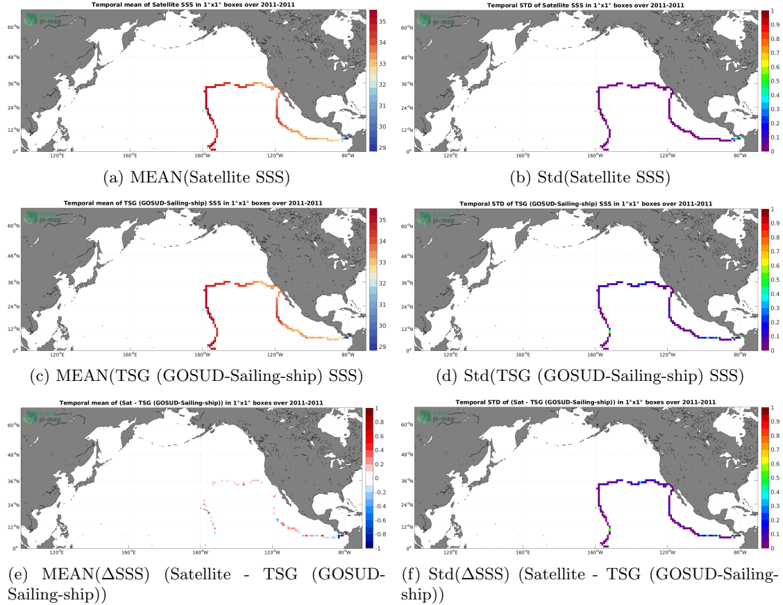
Figure 6: Temporal mean (left) and Std (right) of SSS from SMAP SSS L4 OI v2 - Monthly (IPRC) (top), TSG (GOSUD-Sailing-ship) (middle), and of \Delta\text{SSS} (Satellite - TSG (GOSUD-Sailing-ship)). Only match-up pairs are used to generate these maps.
