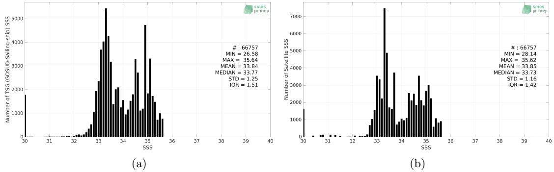
Figure 2: Histograms of SSS from TSG (GOSUD-Sailing-ship) (a) and SMAP SSS L4 OI v2 - Monthly (IPRC) (b) considering all match-up pairs per bins of 0.1 over the North Pacific Ocean Pi-MEP region and for the full satellite product period.
