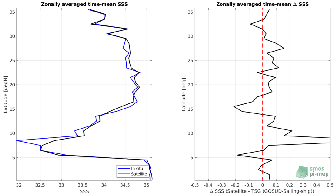
Figure 8: Left panel: Zonal mean SSS from SMAP SSS L4 OI v2 - Monthly (IPRC) satellite product (black) and from TSG (GOSUD-Sailing-ship) (blue). Right panel: Zonal mean of \Delta SSS (Satellite - TSG (GOSUD-Sailing-ship)) for all the collected Pi-MEP match-up pairs estimated over the full satellite product period.
