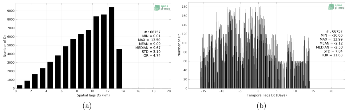
Figure 5: Histograms of the spatial (a) and temporal (b) lags between the location/time of the TSG (GOSUD-Sailing-ship) measurement and the date of the corresponding SMAP SSS L4 OI v2 - Monthly (IPRC) SSS pixel.
