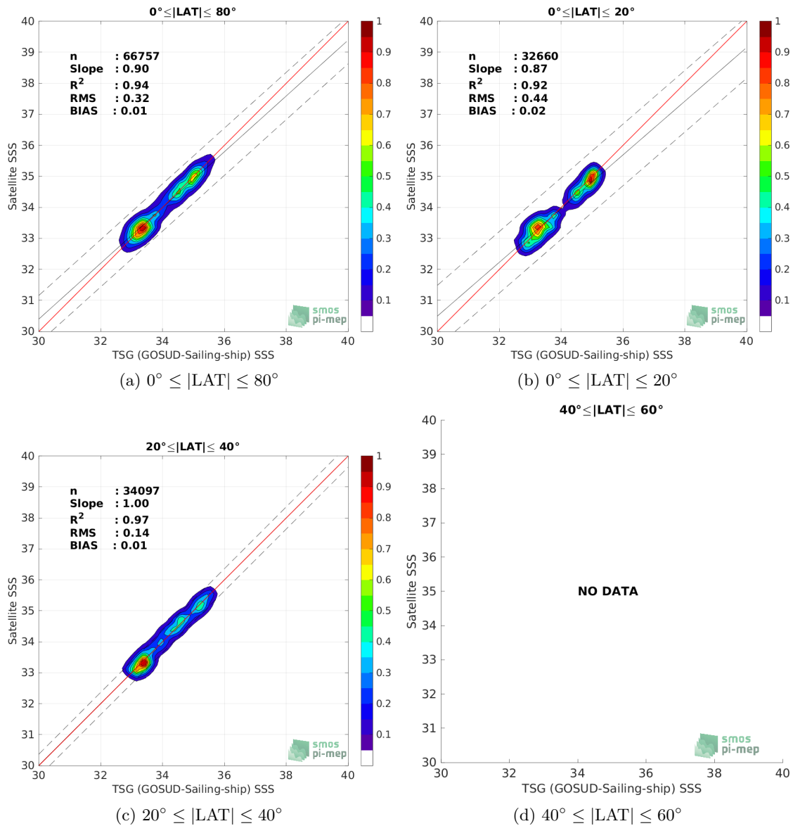
Figure 9: Contour maps of the concentration of SMAP SSS L4 OI v2 - Monthly (IPRC) SSS (y-axis) versus TSG (GOSUD-Sailing-ship) SSS (x-axis) at match-up pairs for different latitude bands. For each plot, the red line shows x=y . The black thin and dashed lines indicate a linear fit through the data cloud and the \pm 95\% confidence levels, respectively. The number match-up pairs n , the slope and R^2 coefficient of the linear fit, the root mean square (RMS) and the mean bias between satellite and in situ data are indicated for each latitude band in each plots.
