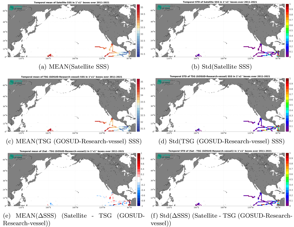
Figure 6: Temporal mean (left) and Std (right) of SSS from SMAP SSS L4 OI v2 - Monthly (IPRC) (top), TSG (GOSUD-Research-vessel) (middle), and of \Delta SSS (Satellite - TSG (GOSUD-Research-vessel)). Only match-up pairs are used to generate these maps.
