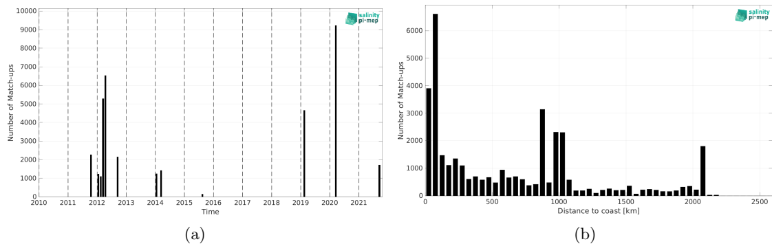
Figure 1: Number of match-ups between TSG (GOSUD-Research-vessel) and SMAP SSS L4 OI v2 - Monthly (IPRC) SSS as a function of time (a) and as function of the distance to coast (b) over the North Pacific Ocean Pi-MEP region and for the full satellite product period.
