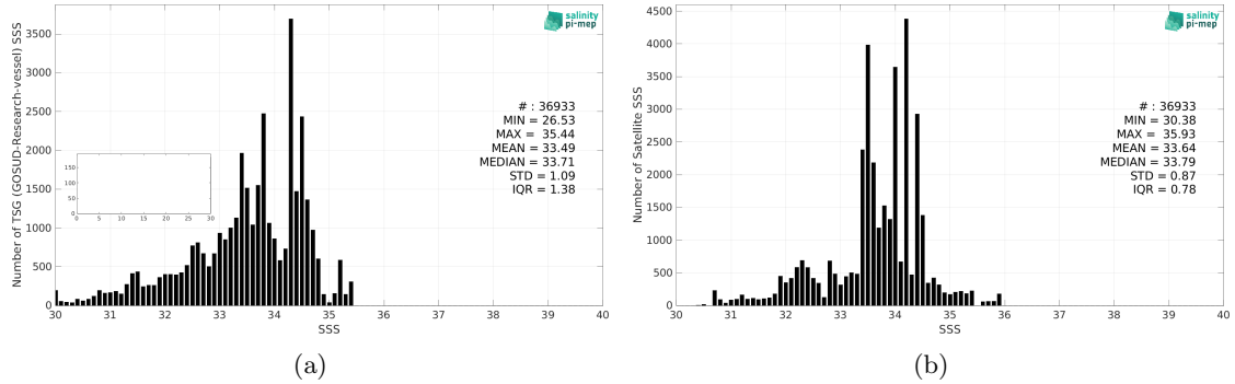
Figure 2: Histograms of SSS from TSG (GOSUD-Research-vessel) (a) and SMAP SSS L4 OI v2 - Monthly (IPRC) (b) considering all match-up pairs per bins of 0.1 over the North Pacific Ocean Pi-MEP region and for the full satellite product period.
