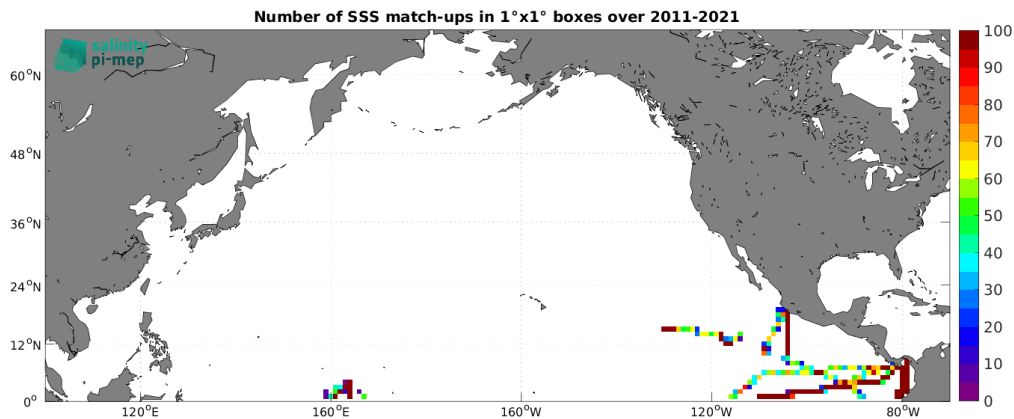
Figure 4: Number of SSS match-ups between TSG (GOSUD-Research-vessel) SSS and the SMAP SSS L4 OI v2 - Monthly (IPRC) SSS product for the North Pacific Ocean Pi-MEP region over 1^\circ \times 1^\circ boxes and for the full satellite product period.
