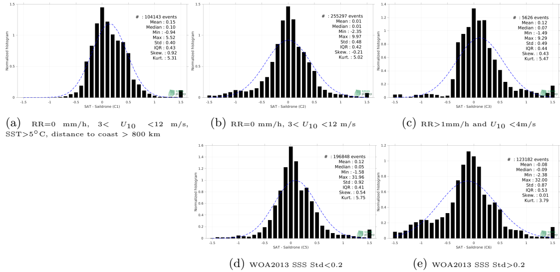
Figure 13: Normalized histogram of \Delta SSS (SMAP SSS L4 OI v2 - Monthly (IPRC) - Sairdronne) for 5 different subdatasets corresponding to: RR=0 mm/h, 3 < U_{10} < 12 m/s, SST>5°C, distance to coast > 800 km (a), RR=0 mm/h, 3 < U_{10} < 12 m/s (b), RR>1mm/h and U_{10} < 4 m/s (c), WOA2013 SSS Std<0.2 (d), WOA2013 SSS Std>0.2 (e).
