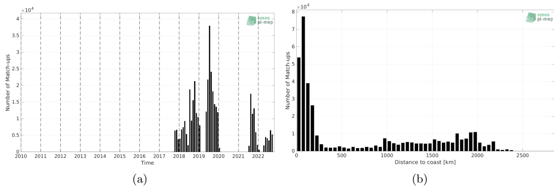
Figure 1: Number of match-ups between Saildrone and SMAP SSS L4 OI v2 - Monthly (IPRC) SSS as a function of time (a) and as function of the distance to coast (b) over the North Pacific Ocean Pi-MEP region and for the full satellite product period.
