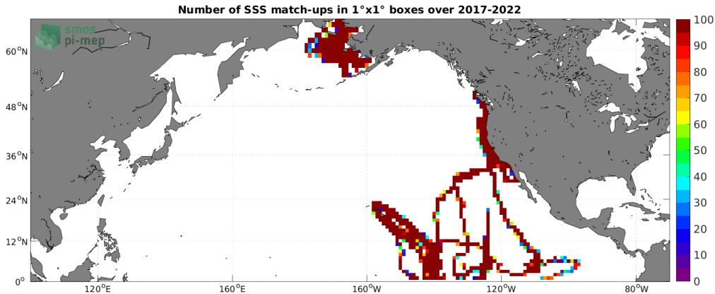
Figure 4: Number of SSS match-ups between Saildrone SSS and the SMAP SSS L4 OI v2 - Monthly (IPRC) SSS product for the North Pacific Ocean Pi-MEP region over 1^\circ \times 1^\circ boxes and for the full satellite product period.
