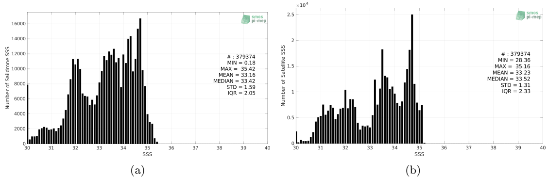
Figure 2: Histograms of SSS from Saildrone (a) and SMAP SSS L4 OI v2 - Monthly (IPRC) (b) considering all match-up pairs per bins of 0.1 over the North Pacific Ocean Pi-MEP region and for the full satellite product period.
