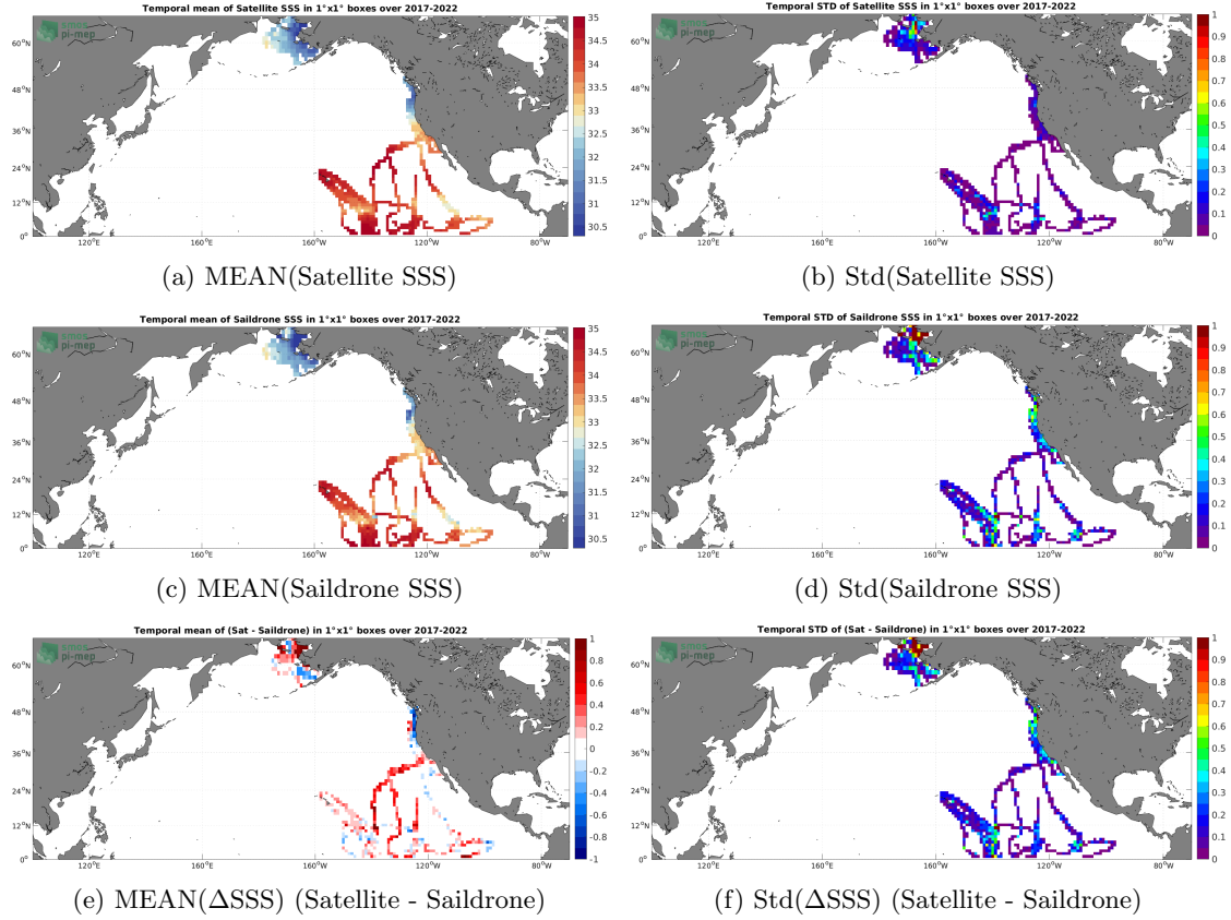
Figure 6: Temporal mean (left) and Std (right) of SSS from SMAP SSS L4 OI v2 - Monthly (IPRC) (top), Sairdrone (middle), and of \Delta\text{SSS} (Satellite - Sairdrone). Only match-up pairs are used to generate these maps.
