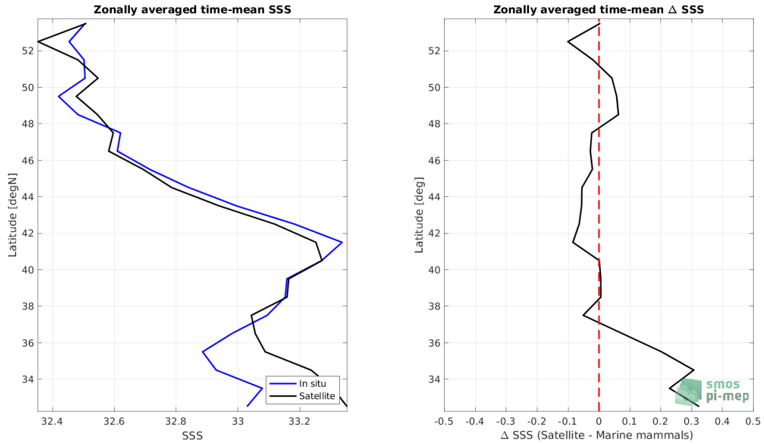
Figure 8: Left panel: Zonal mean SSS from SMAP SSS L4 OI v2 - Monthly (IPRC) satellite product (black) and from Marine mammals (blue). Right panel: Zonal mean of \Delta SSS (Satellite - Marine mammals) for all the collected Pi-MEP match-up pairs estimated over the full satellite product period.
