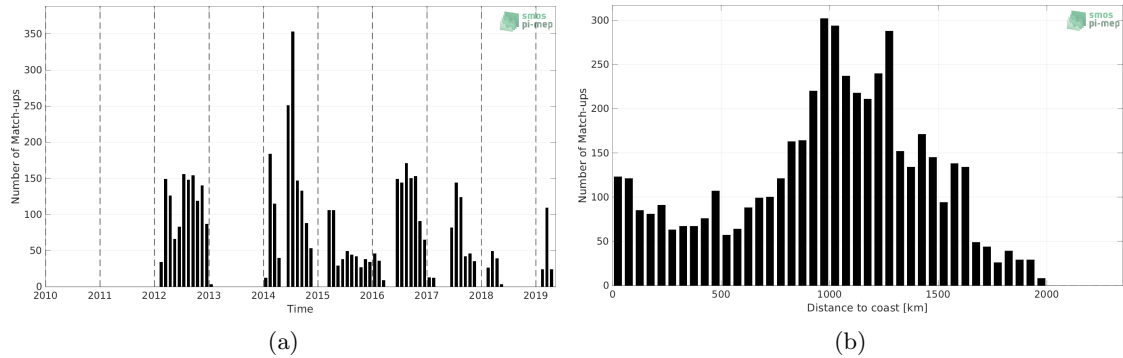
Figure 1: Number of match-ups between Marine mammals and SMAP SSS L4 OI v2 - Monthly (IPRC) SSS as a function of time (a) and as function of the distance to coast (b) over the North Pacific Ocean Pi-MEP region and for the full satellite product period.
