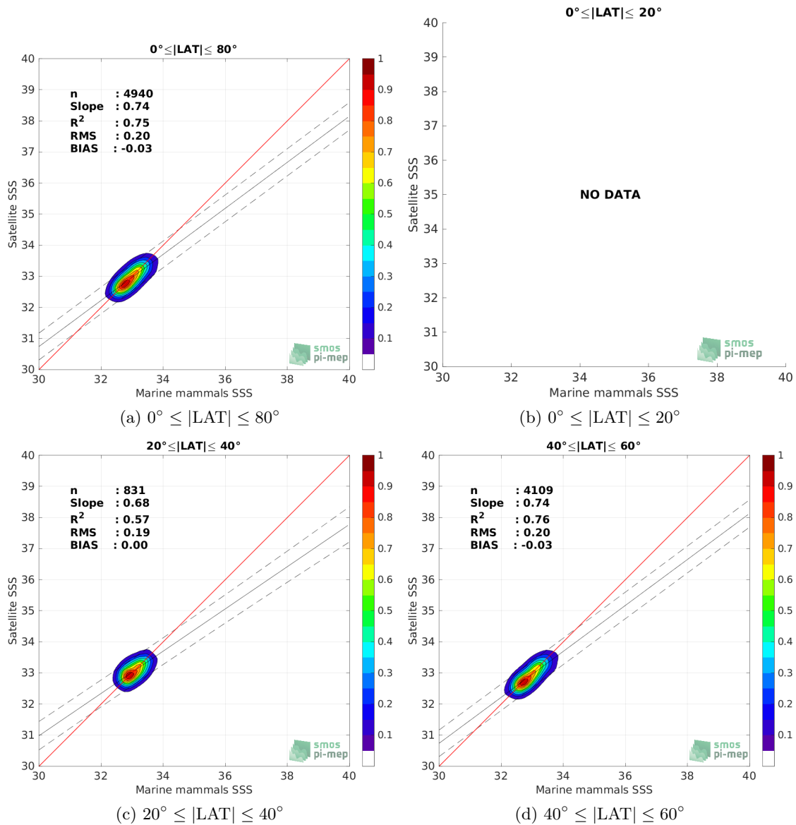
Figure 9: Contour maps of the concentration of SMAP SSS L4 OI v2 - Monthly (IPRC) SSS (y-axis) versus Marine mammals SSS (x-axis) at match-up pairs for different latitude bands. For each plot, the red line shows x=y . The black thin and dashed lines indicate a linear fit through the data cloud and the \pm 95\% confidence levels, respectively. The number match-up pairs n , the slope and R^2 coefficient of the linear fit, the root mean square (RMS) and the mean bias between satellite and in situ data are indicated for each latitude band in each plots.
