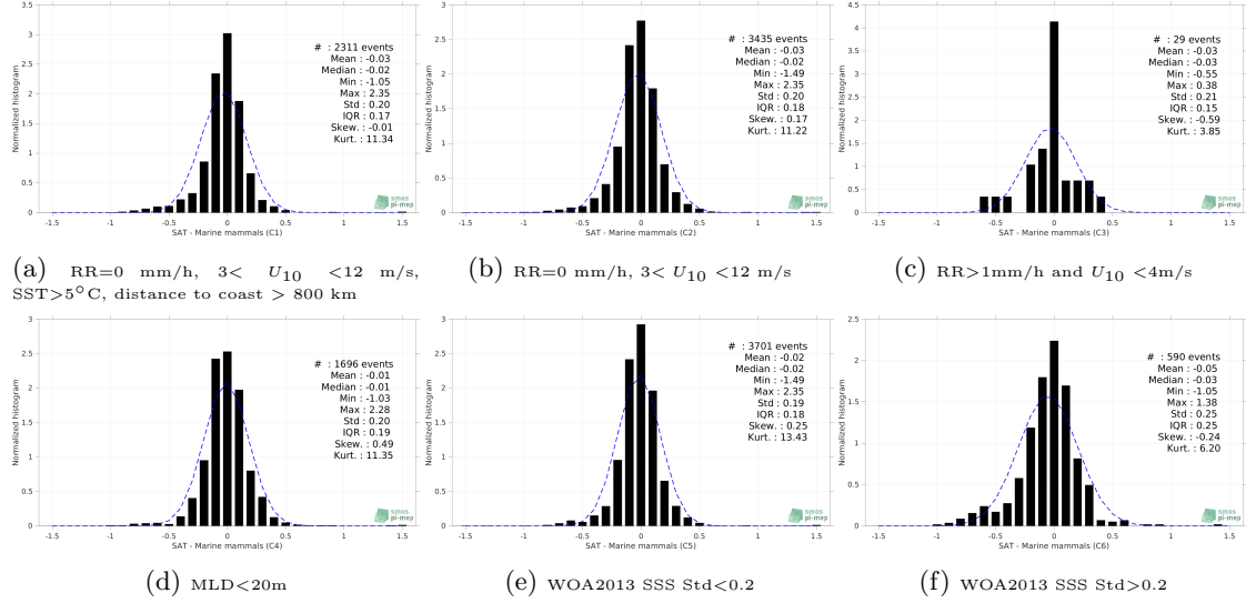
Figure 13: Normalized histogram of \Delta SSS (SMAP SSS L4 OI v2 - Monthly (IPRC) - Marine mammals) for 6 different subdatasets corresponding to: RR=0 mm/h, 3 < U_{10} < 12 m/s, SST>5°C, distance to coast > 800 km (a), RR=0 mm/h, 3 < U_{10} < 12 m/s (b), RR>1mm/h and U_{10} < 4 m/s (c), MLD<20m (d), WOA2013 SSS Std<0.2 (e), WOA2013 SSS Std>0.2 (f).
