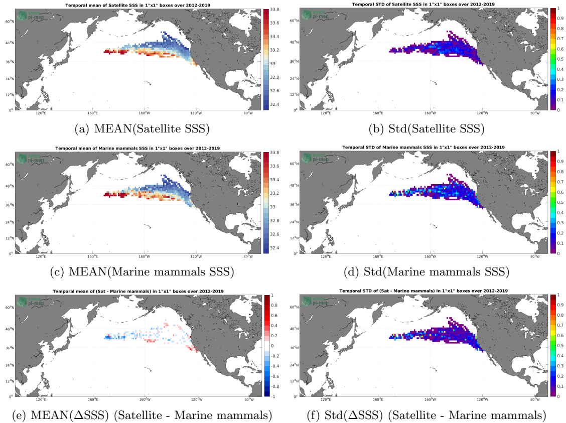
Figure 6: Temporal mean (left) and Std (right) of SSS from SMAP SSS L4 OI v2 - Monthly (IPRC) (top), Marine mammals (middle), and of \Delta SSS (Satellite - Marine mammals). Only match-up pairs are used to generate these maps.
