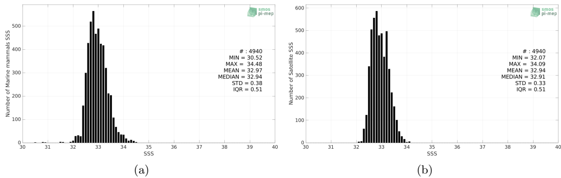
Figure 2: Histograms of SSS from Marine mammals (a) and SMAP SSS L4 OI v2 - Monthly (IPRC) (b) considering all match-up pairs per bins of 0.1 over the North Pacific Ocean Pi-MEP region and for the full satellite product period.
