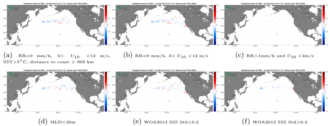
Figure 12: Temporal mean gridded over spatial boxes of size 1^\circ \times 1^\circ of \Delta SSS (SMAP SSS L4 OI v2 - Monthly (IPRC) - Marine mammals) for 6 different subdatasets corresponding to:RR=0 mm/h, 3 < U_{10} < 12 m/s, SST > 5^\circ C , distance to coast > 800 km (a), RR=0 mm/h, 3 < U_{10} < 12 m/s (b), RR > 1 mm/h and U_{10} < 4 m/s (c),MLD < 20 m (d),WOA2013 SSS Std < 0.2 (e),WOA2013 SSS Std > 0.2 (f).
