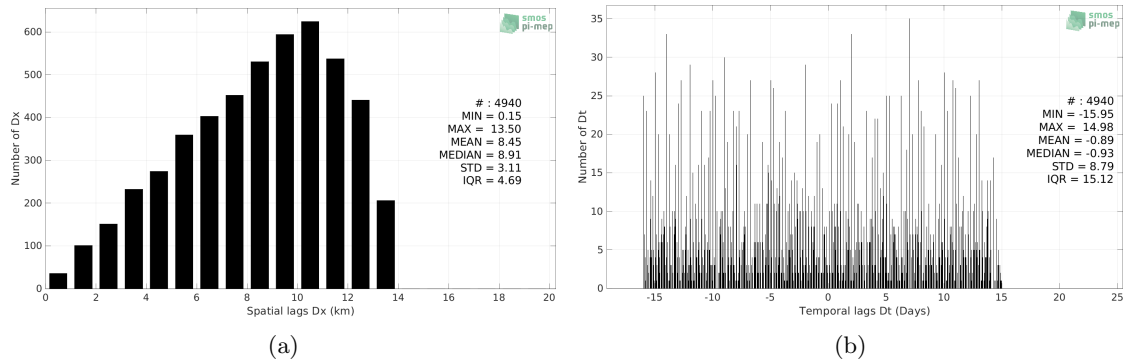
Figure 5: Histograms of the spatial (a) and temporal (b) lags between the location/time of the Marine mammals measurement and the date of the corresponding SMAP SSS L4 OI v2 - Monthly (IPRC) SSS pixel.
