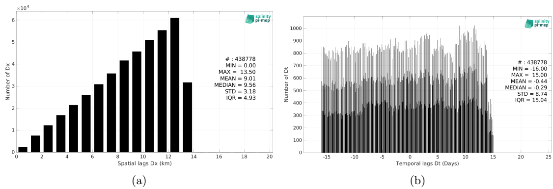
Figure 4: Histograms of the spatial (a) and temporal (b) lags between the location/time of the Surface drifters measurement and the date of the corresponding SMAP SSS L4 OI v2 - Monthly (IPRC) SSS pixel.
