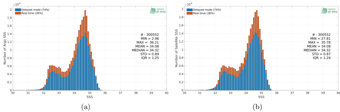
Figure 2: Histograms of SSS from Argo (a) and SMAP SSS L4 OI v2 - Monthly (IPRC) (b) considering all match-up pairs per bins of 0.1 over the North Pacific Ocean Pi-MEP region and for the full satellite product period.
