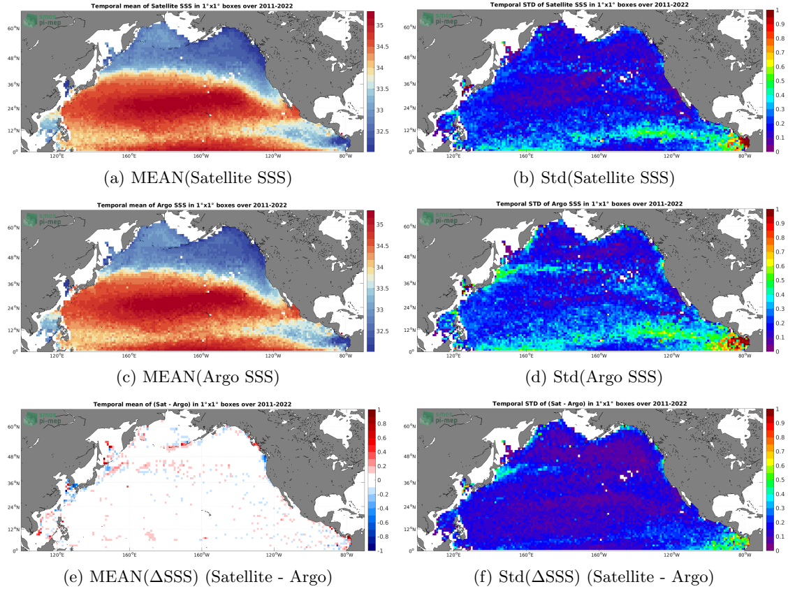
Figure 6: Temporal mean (left) and Std (right) of SSS from SMAP SSS L4 OI v2 - Monthly (IPRC) (top), Argo (middle), and of \Delta SSS (Satellite - Argo). Only match-up pairs are used to generate these maps.
