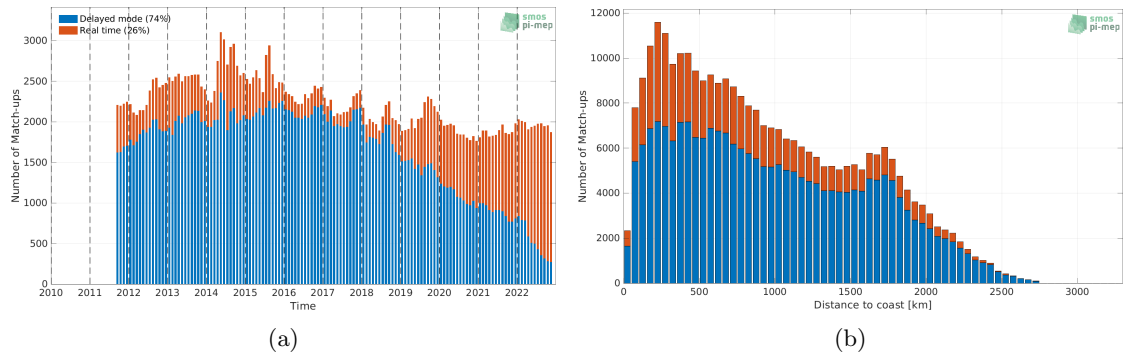
Figure 1: Number of match-ups between Argo and SMAP SSS L4 OI v2 - Monthly (IPRC) SSS as a function of time (a) and as function of the distance to coast (b) over the North Pacific Ocean Pi-MEP region and for the full satellite product period.
