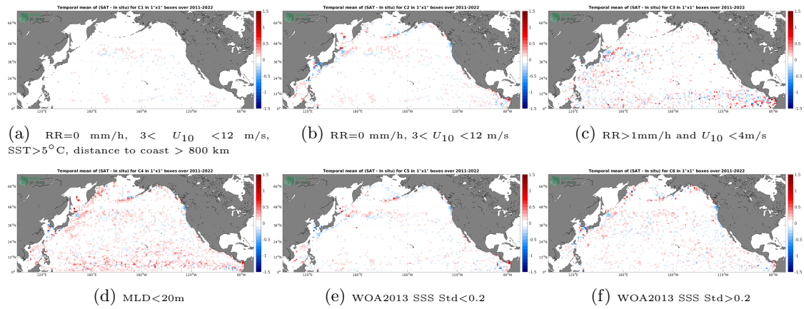
Figure 12: Temporal mean gridded over spatial boxes of size 1^\circ \times 1^\circ of \Delta SSS (SMAP SSS L4 OI v2 - Monthly (IPRC) - Argo) for 6 different subdatasets corresponding to:RR=0 mm/h, 3 < U_{10} < 12 m/s, SST >5^\circ\text{C} , distance to coast > 800 km (a), RR=0 mm/h, 3 < U_{10} < 12 m/s (b), RR >1 mm/h and U_{10} < 4 m/s (c),MLD <20 m (d),WOA2013 SSS Std <0.2 (e),WOA2013 SSS Std >0.2 (f).
