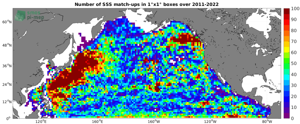
Figure 4: Number of SSS match-ups between Argo SSS and the SMAP SSS L4 OI v2 - Monthly (IPRC) SSS product for the North Pacific Ocean Pi-MEP region over 1^\circ \times 1^\circ boxes and for the full satellite product period.
