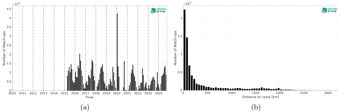
Figure 2: Number of match-ups between TSG (SAMOS) and SMAP SSS L3 v6 - 8-Day running (RSS) SSS as a function of time (a) and as function of the distance to coast (b) over the North Pacific Ocean Pi-MEP region and for the full satellite product period.
