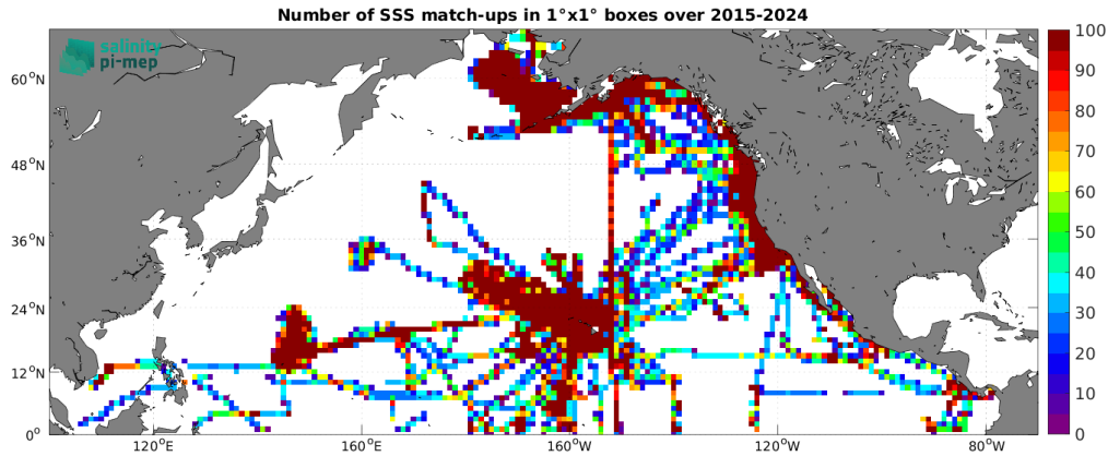
Figure 5: Number of SSS match-ups between TSG (SAMOS) SSS and the SMAP SSS L3 v6 - 8-Day running (RSS) SSS product for the North Pacific Ocean Pi-MEP region over 1^\circ \times 1^\circ boxes and for the full satellite product period.
