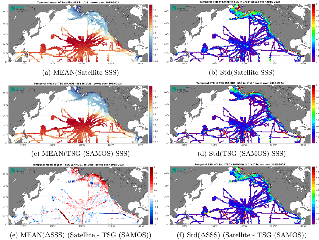
Figure 7: Temporal mean (left) and Std (right) of SSS from SMAP SSS L3 v6 - 8-Day running (RSS) (top), TSG (SAMOS) (middle), and of \Delta\text{SSS} (Satellite - TSG (SAMOS)). Only match-up pairs are used to generate these maps.
