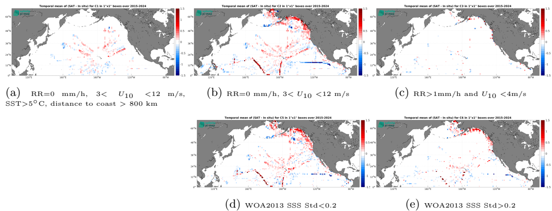
Figure 14: Temporal mean gridded over spatial boxes of size 1^\circ \times 1^\circ of \Delta SSS (SMAP SSS L3 v6 - 8-Day running (RSS) - TSG (SAMOS)) for 5 different subdatasets corresponding to:RR=0 mm/h, 3 < U_{10} < 12 m/s, SST >5^\circ C, distance to coast > 800 km (a), RR=0 mm/h, 3 < U_{10} < 12 m/s (b), RR >1 mm/h and U_{10} < 4 m/s (c), WOA2013 SSS Std <0.2 (d), WOA2013 SSS Std >0.2 (e).
