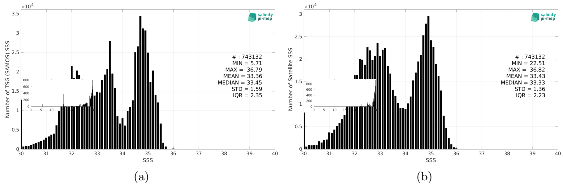
Figure 3: Histograms of SSS from TSG (SAMOS) (a) and SMAP SSS L3 v6 - 8-Day running (RSS) (b) considering all match-up pairs per bins of 0.1 over the North Pacific Ocean Pi-MEP region and for the full satellite product period.
