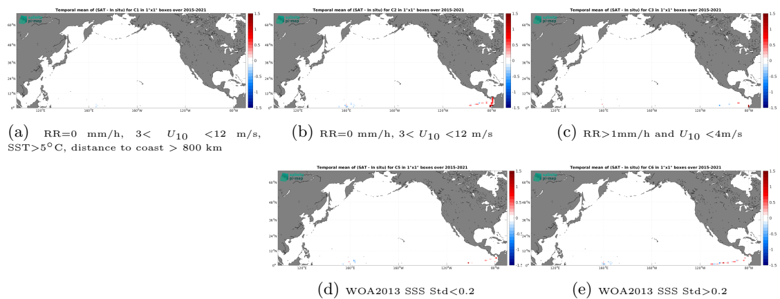
Figure 14: Temporal mean gridded over spatial boxes of size 1^\circ \times 1^\circ of \Delta SSS (SMAP SSS L3 v6 - 8-Day running (RSS) - TSG (GOSUD-Research-vessel)) for 5 different subdatasets corresponding to:RR=0 mm/h, 3 < U_{10} < 12 m/s, SST >5^\circ\text{C} , distance to coast > 800 km (a), RR=0 mm/h, 3 < U_{10} < 12 m/s (b), RR >1 mm/h and U_{10} < 4 m/s (c), WOA2013 SSS Std <0.2 (d), WOA2013 SSS Std >0.2 (e).
