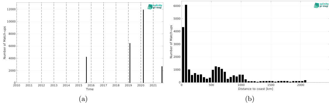
Figure 2: Number of match-ups between TSG (GOSUD-Research-vessel) and SMAP SSS L3 v6 - 8-Day running (RSS) SSS as a function of time (a) and as function of the distance to coast (b) over the North Pacific Ocean Pi-MEP region and for the full satellite product period.
