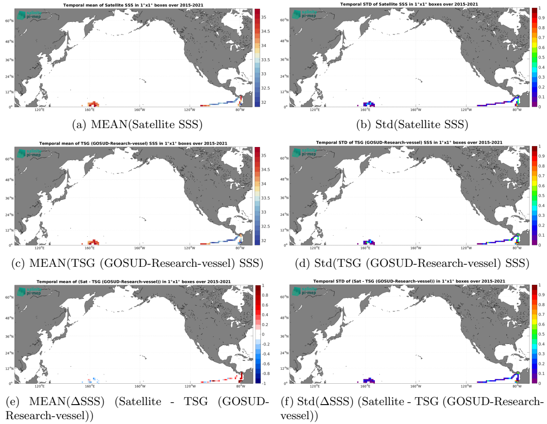
Figure 7: Temporal mean (left) and Std (right) of SSS from SMAP SSS L3 v6 - 8-Day running (RSS) (top), TSG (GOSUD-Research-vessel) (middle), and of \Delta SSS (Satellite - TSG (GOSUD-Research-vessel)). Only match-up pairs are used to generate these maps.
