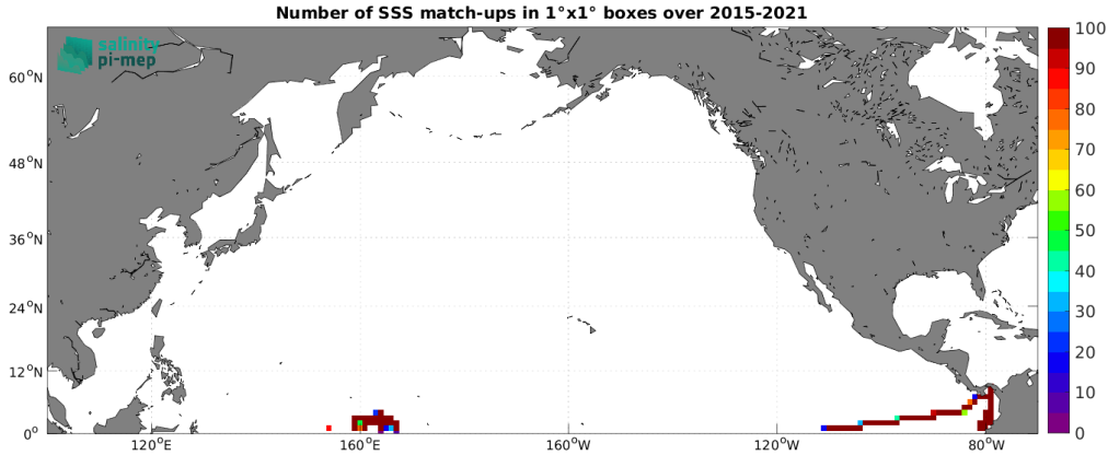
Figure 5: Number of SSS match-ups between TSG (GOSUD-Research-vessel) SSS and the SMAP SSS L3 v6 - 8-Day running (RSS) SSS product for the North Pacific Ocean Pi-MEP region over 1^\circ \times 1^\circ boxes and for the full satellite product period.
