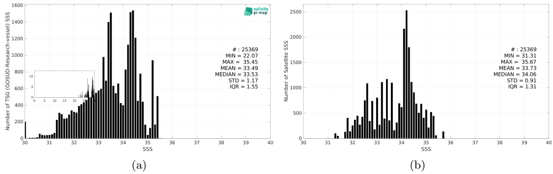
Figure 3: Histograms of SSS from TSG (GOSUD-Research-vessel) (a) and SMAP SSS L3 v6 - 8-Day running (RSS) (b) considering all match-up pairs per bins of 0.1 over the North Pacific Ocean Pi-MEP region and for the full satellite product period.
