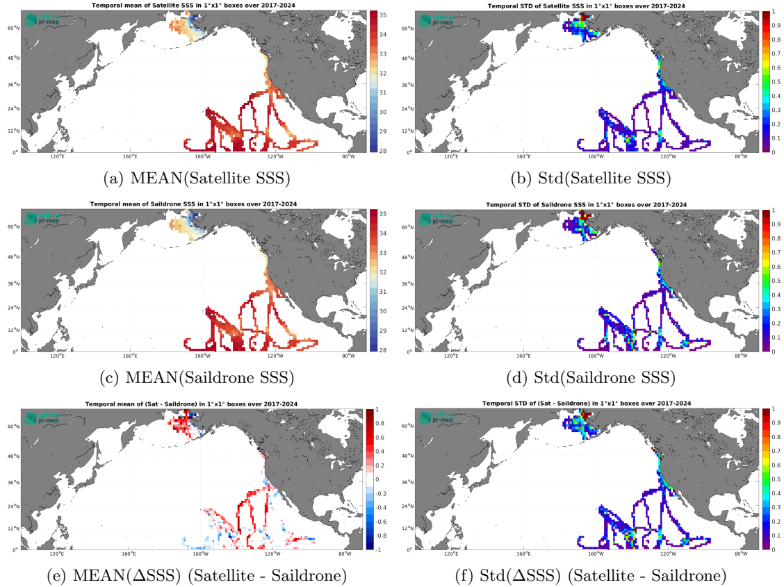
Figure 7: Temporal mean (left) and Std (right) of SSS from SMAP SSS L3 v6 - 8-Day running (RSS) (top), Saildrone (middle), and of \Delta SSS (Satellite - Saildrone). Only match-up pairs are used to generate these maps.
