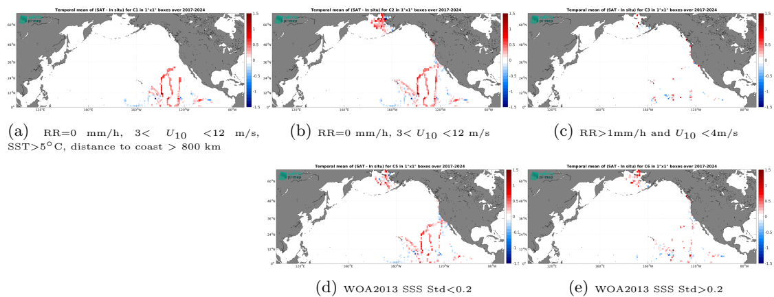
Figure 14: Temporal mean gridded over spatial boxes of size 1^\circ \times 1^\circ of \Delta SSS (SMAP SSS L3 v6 - 8-Day running (RSS) - Sairdrone) for 5 different subdatasets corresponding to:RR=0 mm/h, 3 < U_{10} < 12 m/s, SST > 5^\circ\text{C} , distance to coast > 800 km (a), RR=0 mm/h, 3 < U_{10} < 12 m/s (b), RR > 1 mm/h and U_{10} < 4 m/s (c), WOA2013 SSS Std < 0.2 (d), WOA2013 SSS Std > 0.2 (e).
