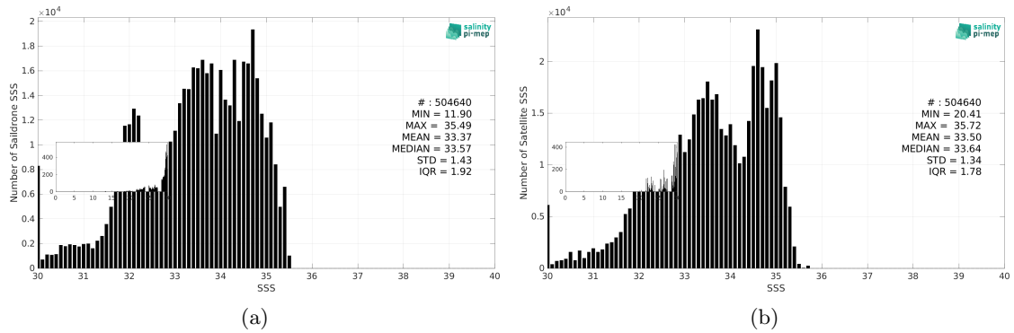
Figure 3: Histograms of SSS from Saildrone (a) and SMAP SSS L3 v6 - 8-Day running (RSS) (b) considering all match-up pairs per bins of 0.1 over the North Pacific Ocean Pi-MEP region and for the full satellite product period.
