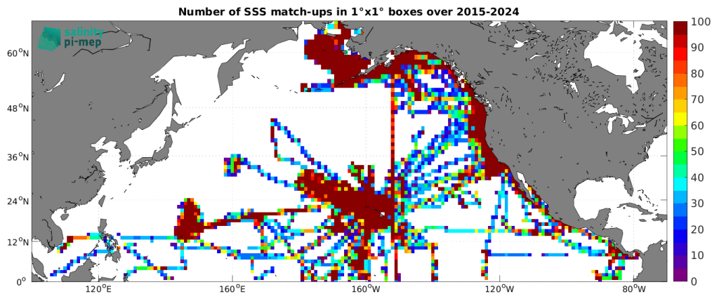
Figure 5: Number of SSS match-ups between TSG (SAMOS) SSS and the SMAP SSS L3 v6 - Monthly (RSS) SSS product for the North Pacific Ocean Pi-MEP region over 1^\circ \times 1^\circ boxes and for the full satellite product period.
