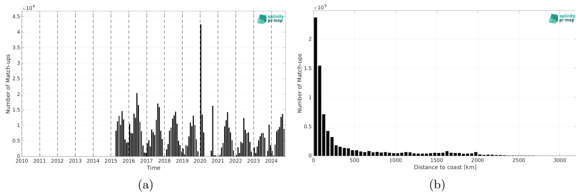
Figure 2: Number of match-ups between TSG (SAMOS) and SMAP SSS L3 v6 - Monthly (RSS) SSS as a function of time (a) and as function of the distance to coast (b) over the North Pacific Ocean Pi-MEP region and for the full satellite product period.
