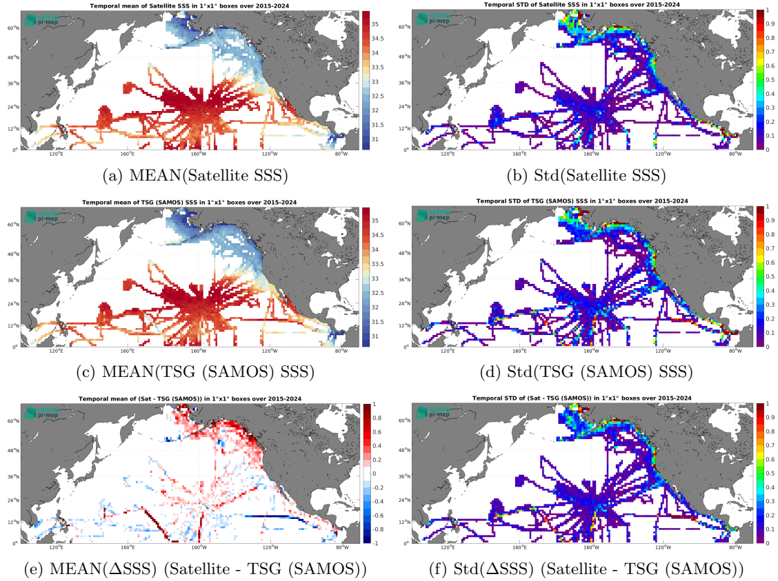
Figure 7: Temporal mean (left) and Std (right) of SSS from SMAP SSS L3 v6 - Monthly (RSS) (top), TSG (SAMOS) (middle), and of \Delta\text{SSS} (Satellite - TSG (SAMOS)). Only match-up pairs are used to generate these maps.
