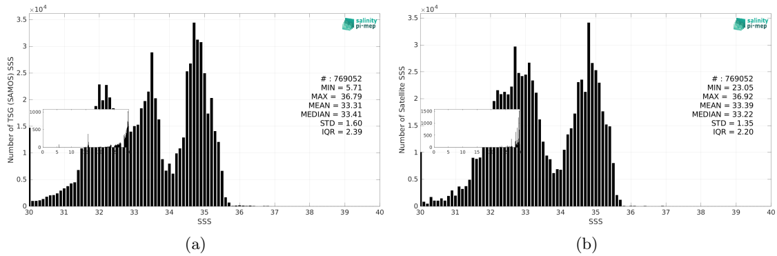
Figure 3: Histograms of SSS from TSG (SAMOS) (a) and SMAP SSS L3 v6 - Monthly (RSS) (b) considering all match-up pairs per bins of 0.1 over the North Pacific Ocean Pi-MEP region and for the full satellite product period.
