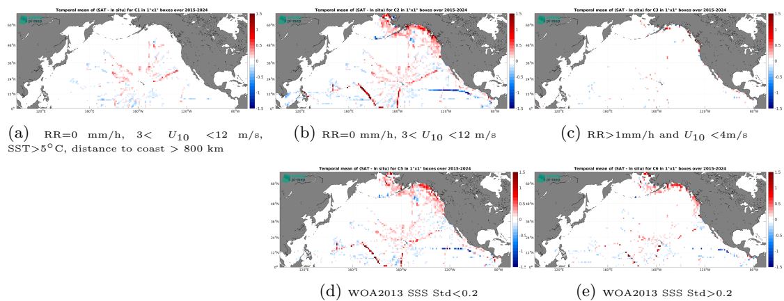
Figure 14: Temporal mean gridded over spatial boxes of size 1^\circ \times 1^\circ of \Delta SSS (SMAP SSS L3 v6 - Monthly (RSS) - TSG (SAMOS)) for 5 different subdatasets corresponding to: RR=0 mm/h, 3 < U_{10} < 12 m/s, SST > 5°C, distance to coast > 800 km (a), RR=0 mm/h, 3 < U_{10} < 12 m/s (b), RR > 1mm/h and U_{10} < 4 m/s (c), WOA2013 SSS Std < 0.2 (d), WOA2013 SSS Std > 0.2 (e).
