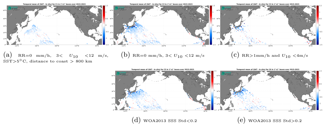
Figure 14: Temporal mean gridded over spatial boxes of size 1^\circ \times 1^\circ of \Delta\text{SSS} (SMAP SSS L3 v6 - Monthly (RSS) - TSG (LEGOS-DM)) for 5 different subdatasets corresponding to:RR=0 mm/h, 3 < U_{10} < 12 m/s, SST >5^\circ\text{C} , distance to coast > 800 km (a), RR=0 mm/h, 3 < U_{10} < 12 m/s (b), RR >1 mm/h and U_{10} < 4 m/s (c), WOA2013 SSS Std <0.2 (d), WOA2013 SSS Std >0.2 (e).
