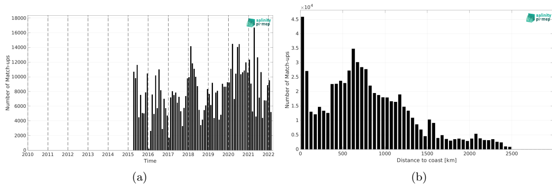
Figure 2: Number of match-ups between TSG (LEGOS-DM) and SMAP SSS L3 v6 - Monthly (RSS) SSS as a function of time (a) and as function of the distance to coast (b) over the North Pacific Ocean Pi-MEP region and for the full satellite product period.
