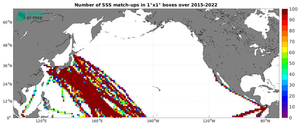
Figure 5: Number of SSS match-ups between TSG (LEGOS-DM) SSS and the SMAP SSS L3 v6 - Monthly (RSS) SSS product for the North Pacific Ocean Pi-MEP region over 1^\circ \times 1^\circ boxes and for the full satellite product period.
