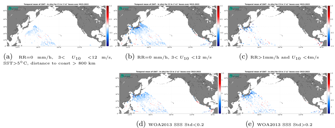
Figure 14: Temporal mean gridded over spatial boxes of size 1^\circ \times 1^\circ of \Delta SSS (SMAP SSS L3 v6 - Monthly (RSS) - TSG (LEGOS-DM)) for 5 different subdatasets corresponding to:RR=0 mm/h, 3 < U_{10} < 12 m/s, SST >5^\circ C, distance to coast > 800 km (a), RR=0 mm/h, 3 < U_{10} < 12 m/s (b), RR >1 mm/h and U_{10} < 4 m/s (c), WOA2013 SSS Std <0.2 (d), WOA2013 SSS Std >0.2 (e).
