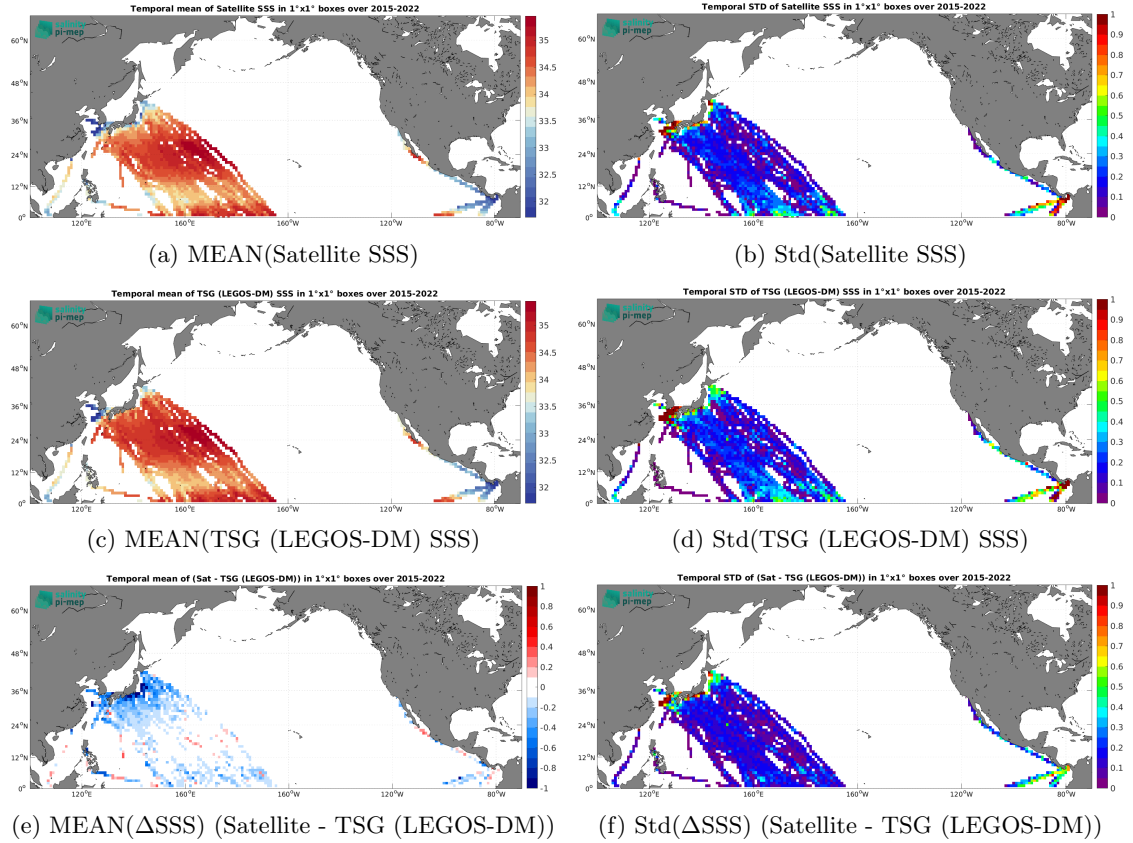
Figure 7: Temporal mean (left) and Std (right) of SSS from SMAP SSS L3 v6 - Monthly (RSS) (top), TSG (LEGOS-DM) (middle), and of \Delta\text{SSS} (Satellite - TSG (LEGOS-DM)). Only match-up pairs are used to generate these maps.
