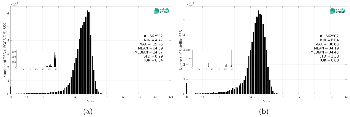
Figure 3: Histograms of SSS from TSG (LEGOS-DM) (a) and SMAP SSS L3 v6 - Monthly (RSS) (b) considering all match-up pairs per bins of 0.1 over the North Pacific Ocean Pi-MEP region and for the full satellite product period.
