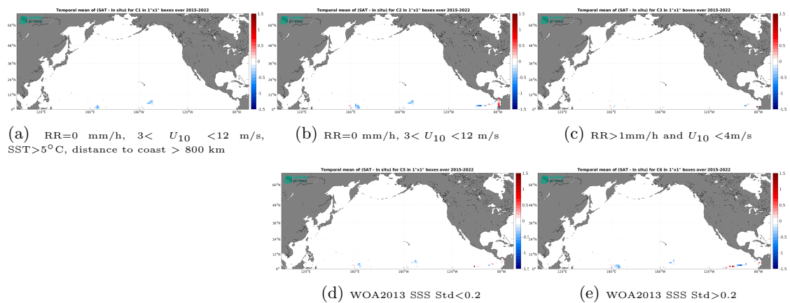
Figure 14: Temporal mean gridded over spatial boxes of size 1^\circ \times 1^\circ of \Delta\text{SSS} (SMAP SSS L3 v6 - Monthly (RSS) - TSG (GOSUD-Research-vessel)) for 5 different subdatasets corresponding to:RR=0 mm/h, 3 < U_{10} < 12 m/s, SST>5°C, distance to coast > 800 km (a), RR=0 mm/h, 3 < U_{10} < 12 m/s (b), RR>1mm/h and U_{10} < 4 m/s (c), WOA2013 SSS Std<0.2 (d), WOA2013 SSS Std>0.2 (e).
