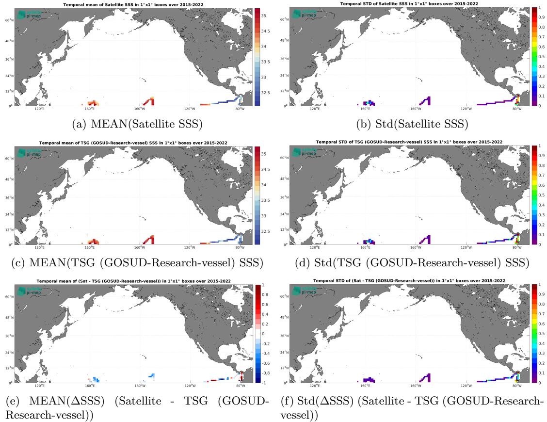
Figure 7: Temporal mean (left) and Std (right) of SSS from SMAP SSS L3 v6 - Monthly (RSS) (top), TSG (GOSUD-Research-vessel) (middle), and of \Delta\text{SSS} (Satellite - TSG (GOSUD-Research-vessel)). Only match-up pairs are used to generate these maps.
