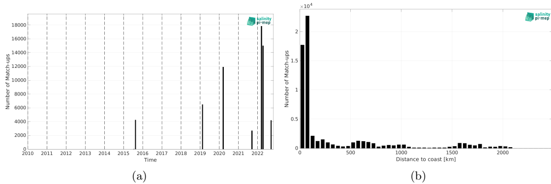
Figure 2: Number of match-ups between TSG (GOSUD-Research-vessel) and SMAP SSS L3 v6 - Monthly (RSS) SSS as a function of time (a) and as function of the distance to coast (b) over the North Pacific Ocean Pi-MEP region and for the full satellite product period.
