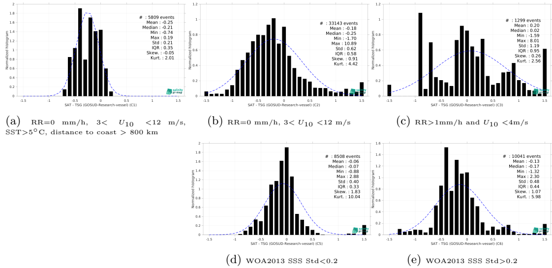
Figure 15: Normalized histogram of \Delta SSS (SMAP SSS L3 v6 - Monthly (RSS) - TSG (GOSUD-Research-vessel)) for 5 different subdatasets corresponding to: RR=0 mm/h, 3 < U_{10} < 12 m/s, SST > 5°C, distance to coast > 800 km (a), RR=0 mm/h, 3 < U_{10} < 12 m/s (b), RR > 1mm/h and U_{10} < 4 m/s (c), WOA2013 SSS Std < 0.2 (d), WOA2013 SSS Std > 0.2 (e).
