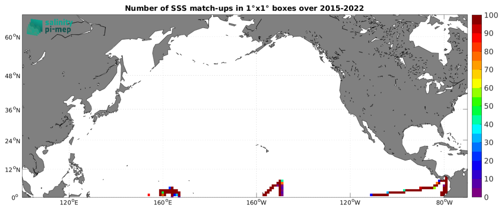
Figure 5: Number of SSS match-ups between TSG (GOSUD-Research-vessel) SSS and the SMAP SSS L3 v6 - Monthly (RSS) SSS product for the North Pacific Ocean Pi-MEP region over 1^\circ \times 1^\circ boxes and for the full satellite product period.
