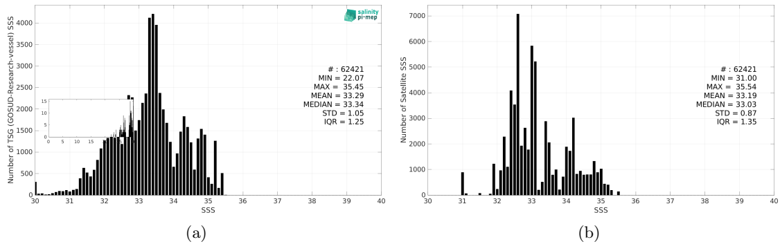
Figure 3: Histograms of SSS from TSG (GOSUD-Research-vessel) (a) and SMAP SSS L3 v6 - Monthly (RSS) (b) considering all match-up pairs per bins of 0.1 over the North Pacific Ocean Pi-MEP region and for the full satellite product period.
