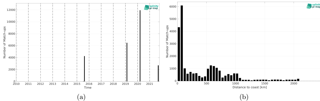
Figure 2: Number of match-ups between TSG (GOSUD-Research-vessel) and SMAP SSS L3 v6 - Monthly (RSS) SSS as a function of time (a) and as function of the distance to coast (b) over the North Pacific Ocean Pi-MEP region and for the full satellite product period.
