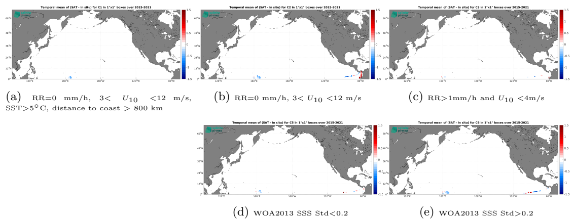
Figure 14: Temporal mean gridded over spatial boxes of size 1^\circ \times 1^\circ of \Delta SSS (SMAP SSS L3 v6 - Monthly (RSS) - TSG (GOSUD-Research-vessel)) for 5 different subdatasets corresponding to:RR=0 mm/h, 3 < U_{10} < 12 m/s, SST >5^\circ C, distance to coast > 800 km (a), RR=0 mm/h, 3 < U_{10} < 12 m/s (b), RR >1 mm/h and U_{10} < 4 m/s (c), WOA2013 SSS Std <0.2 (d), WOA2013 SSS Std >0.2 (e).
