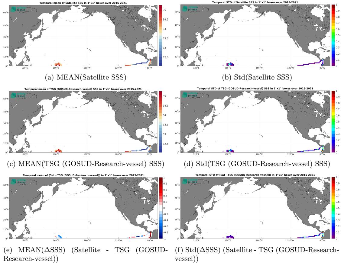
Figure 7: Temporal mean (left) and Std (right) of SSS from SMAP SSS L3 v6 - Monthly (RSS) (top), TSG (GOSUD-Research-vessel) (middle), and of \Delta SSS (Satellite - TSG (GOSUD-Research-vessel)). Only match-up pairs are used to generate these maps.
