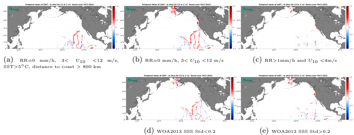
Figure 14: Temporal mean gridded over spatial boxes of size 1^\circ \times 1^\circ of \Delta SSS (SMAP SSS L3 v6 - Monthly (RSS) - Saildrone) for 5 different subdatasets corresponding to:RR=0 mm/h, 3 < U_{10} < 12 m/s, SST >5^\circ\text{C} , distance to coast > 800 km (a), RR=0 mm/h, 3 < U_{10} < 12 m/s (b), RR >1 mm/h and U_{10} < 4 m/s (c), WOA2013 SSS Std <0.2 (d), WOA2013 SSS Std >0.2 (e).
