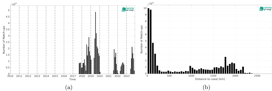
Figure 2: Number of match-ups between Saildrone and SMAP SSS L3 v6 - Monthly (RSS) SSS as a function of time (a) and as function of the distance to coast (b) over the North Pacific Ocean Pi-MEP region and for the full satellite product period.
