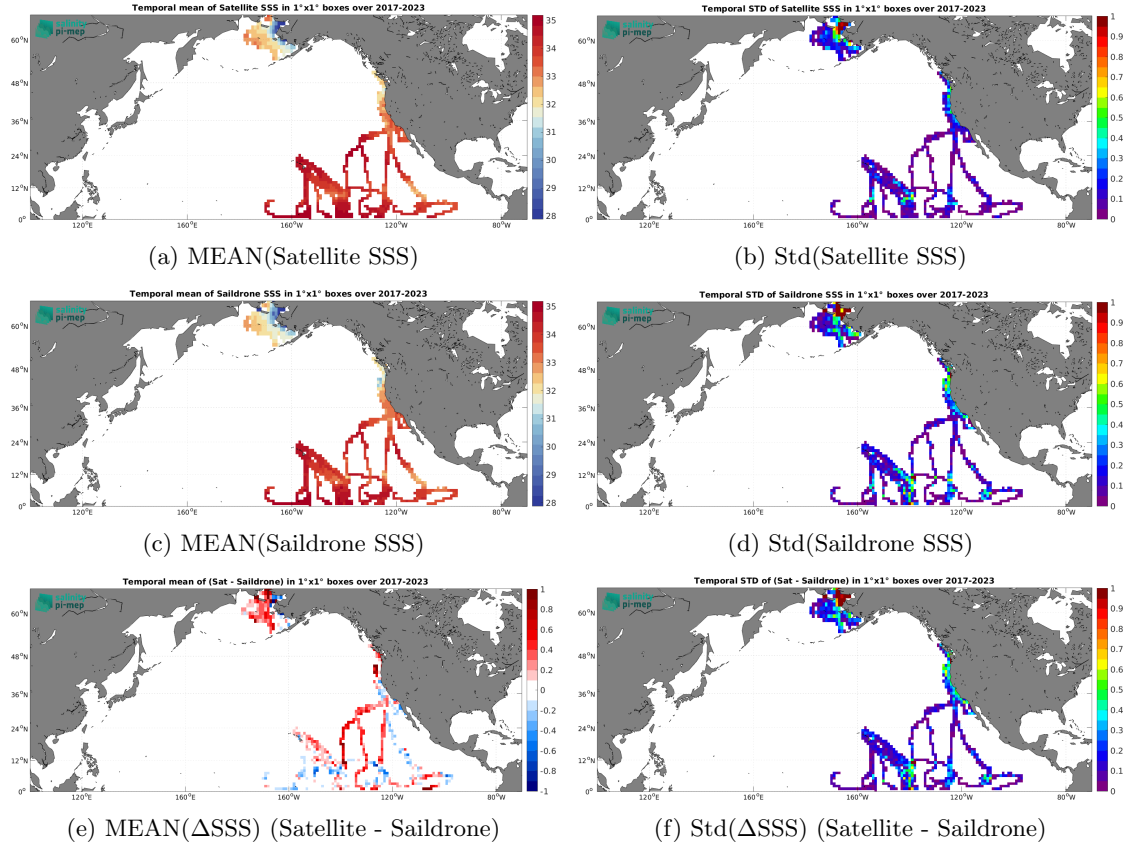
Figure 7: Temporal mean (left) and Std (right) of SSS from SMAP SSS L3 v6 - Monthly (RSS) (top), Saildrone (middle), and of \Delta\text{SSS} (Satellite - Saildrone). Only match-up pairs are used to generate these maps.
