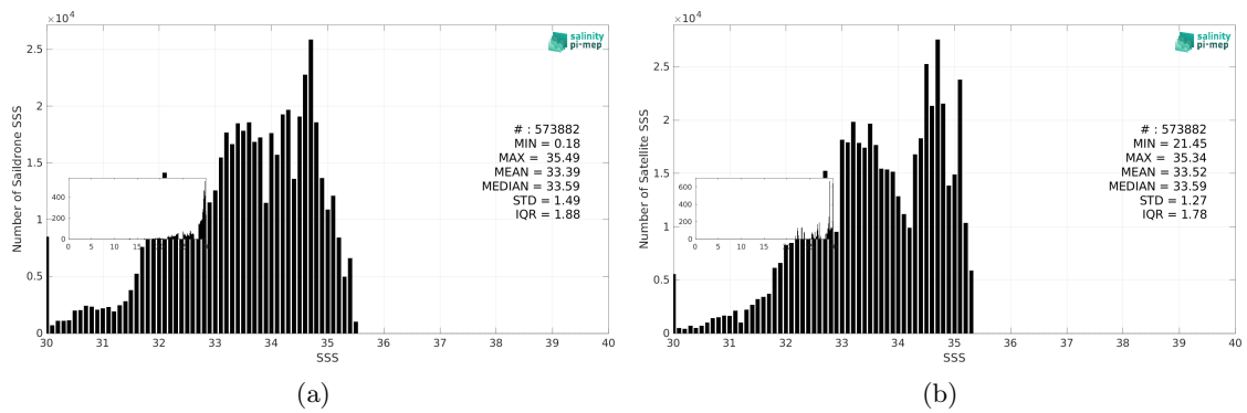
Figure 3: Histograms of SSS from Saldrone (a) and SMAP SSS L3 v6 - Monthly (RSS) (b) considering all match-up pairs per bins of 0.1 over the North Pacific Ocean Pi-MEP region and for the full satellite product period.
