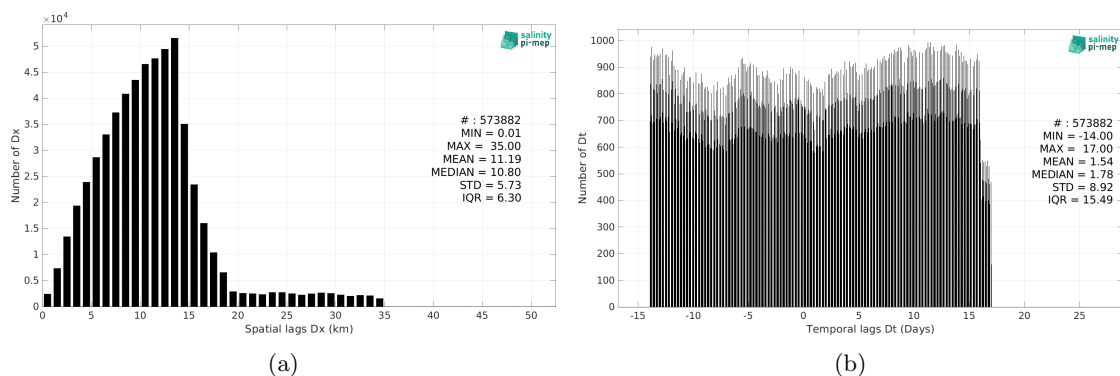
Figure 6: Histograms of the spatial (a) and temporal (b) lags between the location/time of the Sairdrone measurement and the date of the corresponding SMAP SSS L3 v6 - Monthly (RSS) SSS pixel.
