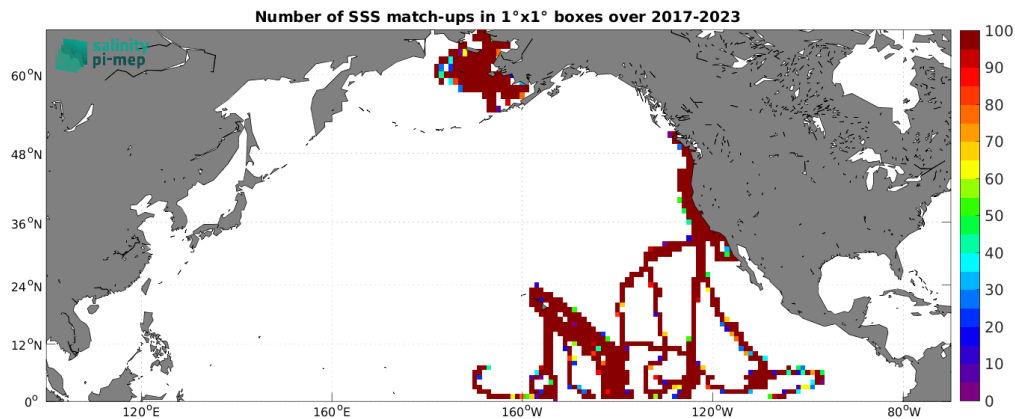
Figure 5: Number of SSS match-ups between Sairdrone SSS and the SMAP SSS L3 v6 - Monthly (RSS) SSS product for the North Pacific Ocean Pi-MEP region over 1^\circ \times 1^\circ boxes and for the full satellite product period.
