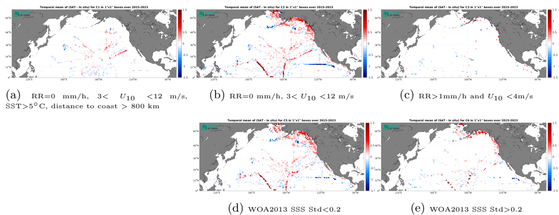
Figure 14: Temporal mean gridded over spatial boxes of size 1^\circ \times 1^\circ of \Delta SSS (SMAP SSS L3 v5.3 - 8-Day running (RSS) - TSG (SAMOS)) for 5 different subdatasets corresponding to:RR=0 mm/h, 3 < U_{10} < 12 m/s, SST>5°C, distance to coast > 800 km (a), RR=0 mm/h, 3 < U_{10} < 12 m/s (b), RR>1mm/h and U_{10} < 4 m/s (c), WOA2013 SSS Std<0.2 (d), WOA2013 SSS Std>0.2 (e).
