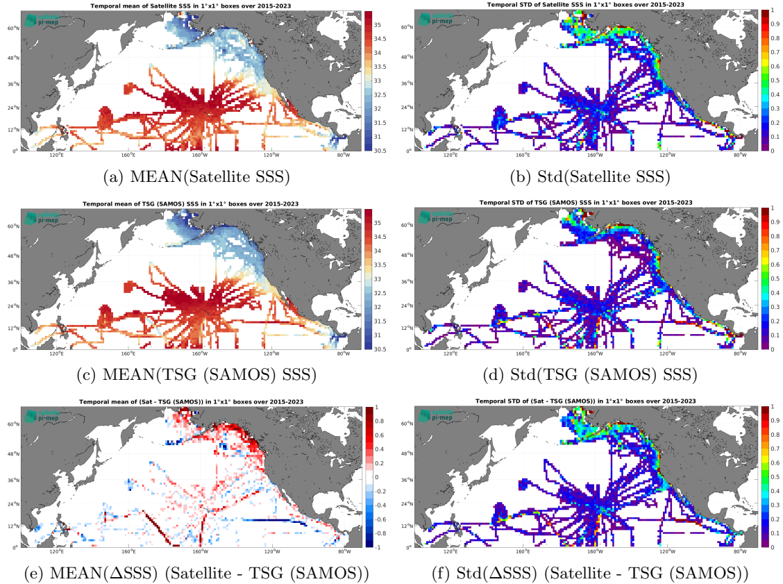
Figure 7: Temporal mean (left) and Std (right) of SSS from SMAP SSS L3 v5.3 - 8-Day running (RSS) (top), TSG (SAMOS) (middle), and of \Delta\text{SSS} (Satellite - TSG (SAMOS)). Only match-up pairs are used to generate these maps.
