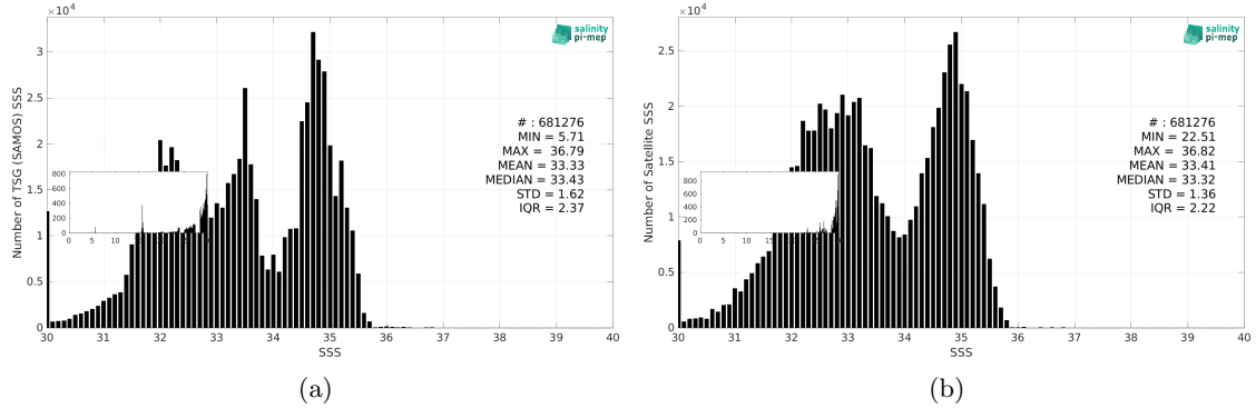
Figure 3: Histograms of SSS from TSG (SAMOS) (a) and SMAP SSS L3 v5.3 - 8-Day running (RSS) (b) considering all match-up pairs per bins of 0.1 over the North Pacific Ocean Pi-MEP region and for the full satellite product period.
