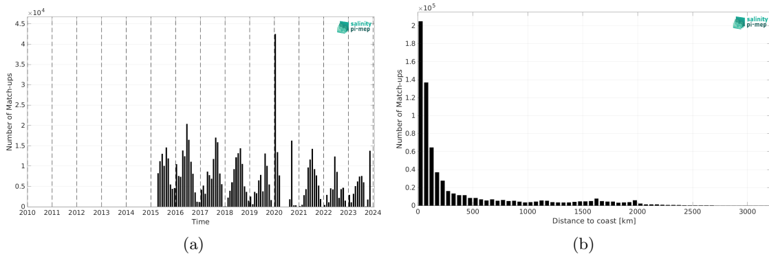
Figure 2: Number of match-ups between TSG (SAMOS) and SMAP SSS L3 v5.3 - 8-Day running (RSS) SSS as a function of time (a) and as function of the distance to coast (b) over the North Pacific Ocean Pi-MEP region and for the full satellite product period.
