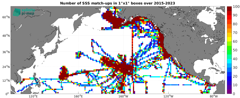
Figure 5: Number of SSS match-ups between TSG (SAMOS) SSS and the SMAP SSS L3 v5.3 - 8-Day running (RSS) SSS product for the North Pacific Ocean Pi-MEP region over 1^\circ \times 1^\circ boxes and for the full satellite product period.
