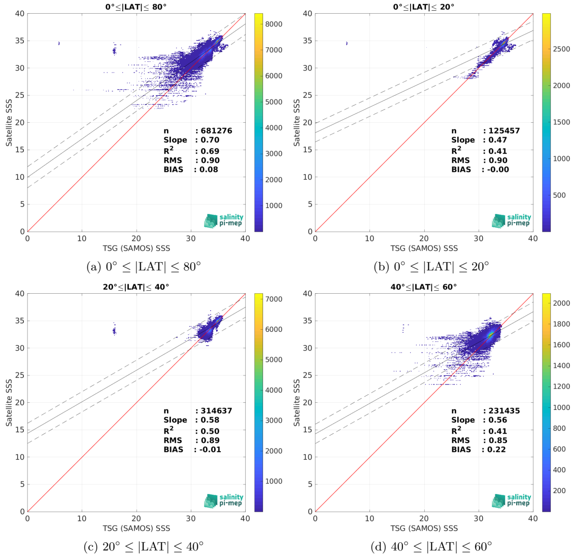
Figure 10: Contour maps of the concentration of SMAP SSS L3 v5.3 - 8-Day running (RSS) SSS (y-axis) versus TSG (SAMOS) SSS (x-axis) at match-up pairs for different latitude bands. For each plot, the red line shows x=y . The black thin and dashed lines indicate a linear fit through the data cloud and the \pm 95\% confidence levels, respectively. The number match-up pairs n , the slope and R^2 coefficient of the linear fit, the root mean square (RMS) and the mean bias between satellite and in situ data are indicated for each latitude band in each plots.
