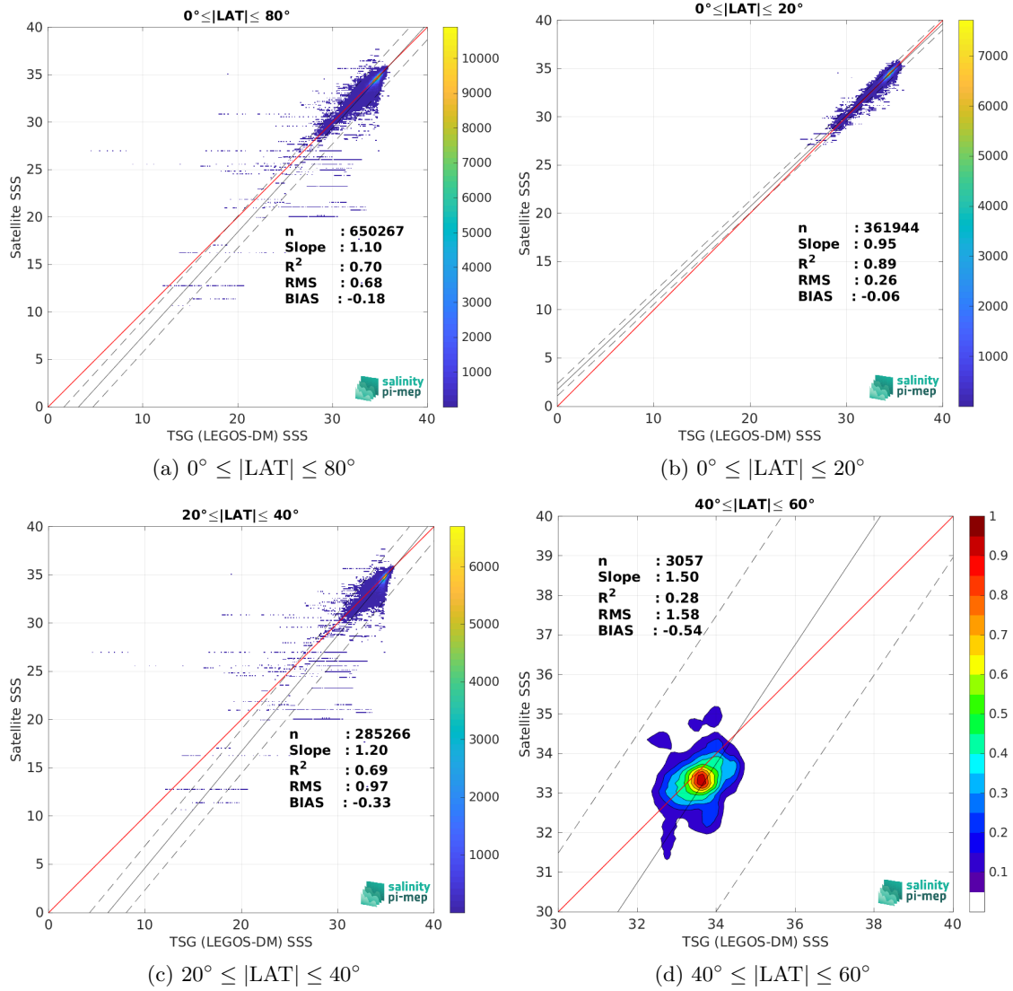
Figure 10: Contour maps of the concentration of SMAP SSS L3 v5.3 - 8-Day running (RSS) SSS (y-axis) versus TSG (LEGOS-DM) SSS (x-axis) at match-up pairs for different latitude bands. For each plot, the red line shows x=y . The black thin and dashed lines indicate a linear fit through the data cloud and the \pm 95\% confidence levels, respectively. The number match-up pairs n , the slope and R^2 coefficient of the linear fit, the root mean square (RMS) and the mean bias between satellite and in situ data are indicated for each latitude band in each plots.
