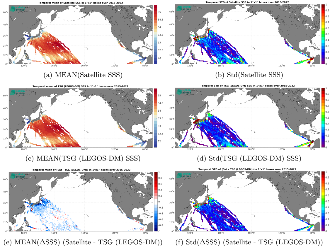
Figure 7: Temporal mean (left) and Std (right) of SSS from SMAP SSS L3 v5.3 - 8-Day running (RSS) (top), TSG (LEGOS-DM) (middle), and of \Delta\text{SSS} (Satellite - TSG (LEGOS-DM)). Only match-up pairs are used to generate these maps.
