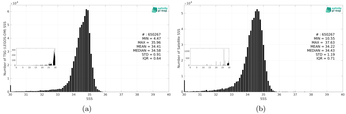
Figure 3: Histograms of SSS from TSG (LEGOS-DM) (a) and SMAP SSS L3 v5.3 - 8-Day running (RSS) (b) considering all match-up pairs per bins of 0.1 over the North Pacific Ocean Pi-MEP region and for the full satellite product period.
