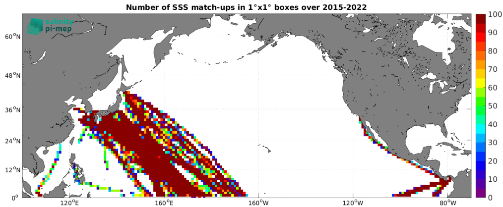
Figure 5: Number of SSS match-ups between TSG (LEGOS-DM) SSS and the SMAP SSS L3 v5.3 - 8-Day running (RSS) SSS product for the North Pacific Ocean Pi-MEP region over 1^\circ \times 1^\circ boxes and for the full satellite product period.
