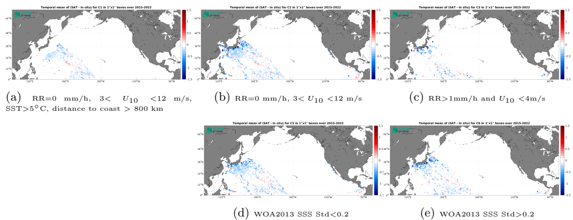
Figure 14: Temporal mean gridded over spatial boxes of size 1^\circ \times 1^\circ of \Delta SSS (SMAP SSS L3 v5.3 - 8-Day running (RSS) - TSG (LEGOS-DM)) for 5 different subdatasets corresponding to:RR=0 mm/h, 3 < U_{10} < 12 m/s, SST >5^\circ\text{C} , distance to coast > 800 km (a), RR=0 mm/h, 3 < U_{10} < 12 m/s (b), RR >1 mm/h and U_{10} < 4 m/s (c), WOA2013 SSS Std <0.2 (d), WOA2013 SSS Std >0.2 (e).
