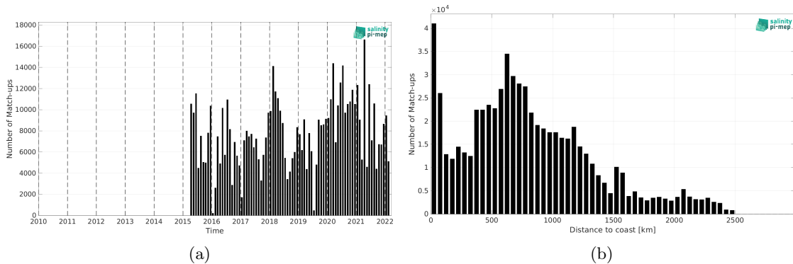
Figure 2: Number of match-ups between TSG (LEGOS-DM) and SMAP SSS L3 v5.3 - 8-Day running (RSS) SSS as a function of time (a) and as function of the distance to coast (b) over the North Pacific Ocean Pi-MEP region and for the full satellite product period.
