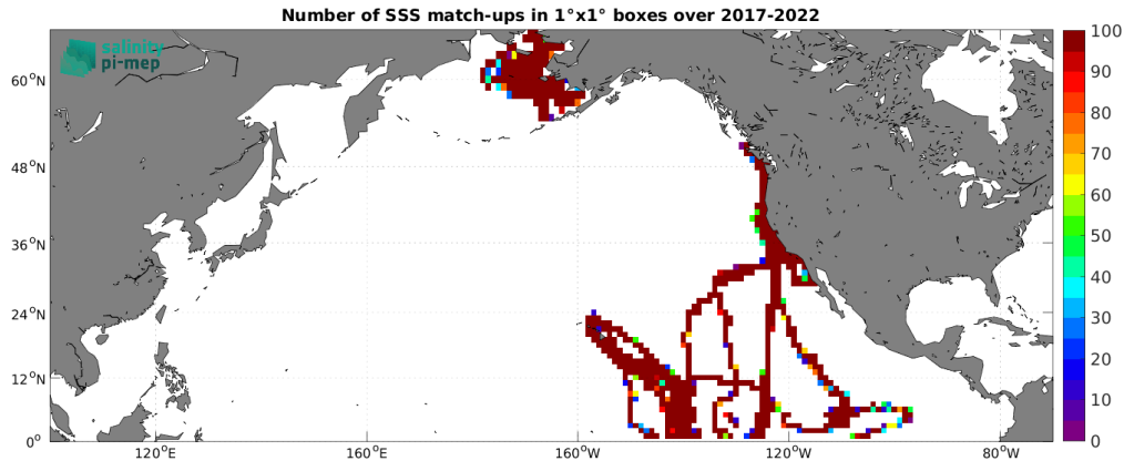
Figure 5: Number of SSS match-ups between Saildrone SSS and the SMAP SSS L3 v5.3 - 8-Day running (RSS) SSS product for the North Pacific Ocean Pi-MEP region over 1^\circ \times 1^\circ boxes and for the full satellite product period.
