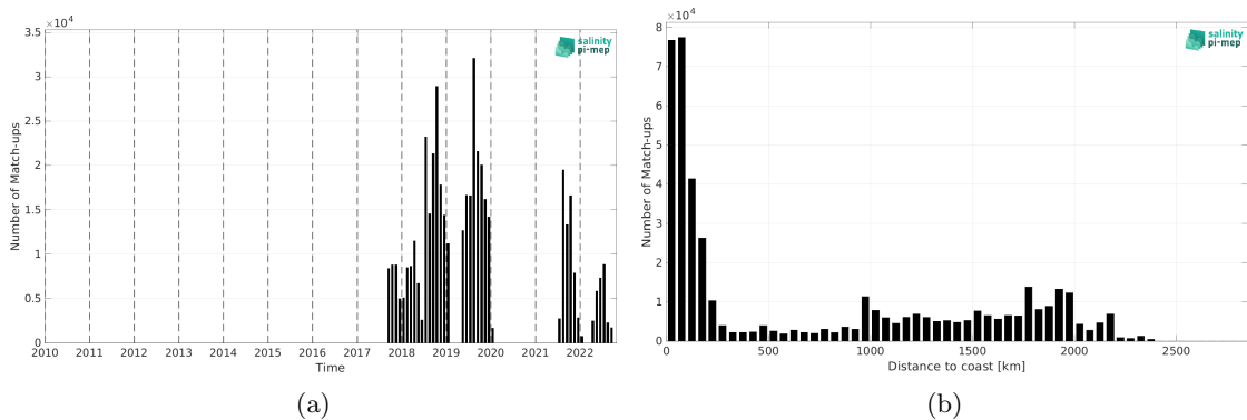
Figure 2: Number of match-ups between Saildrone and SMAP SSS L3 v5.3 - 8-Day running (RSS) SSS as a function of time (a) and as function of the distance to coast (b) over the North Pacific Ocean Pi-MEP region and for the full satellite product period.
