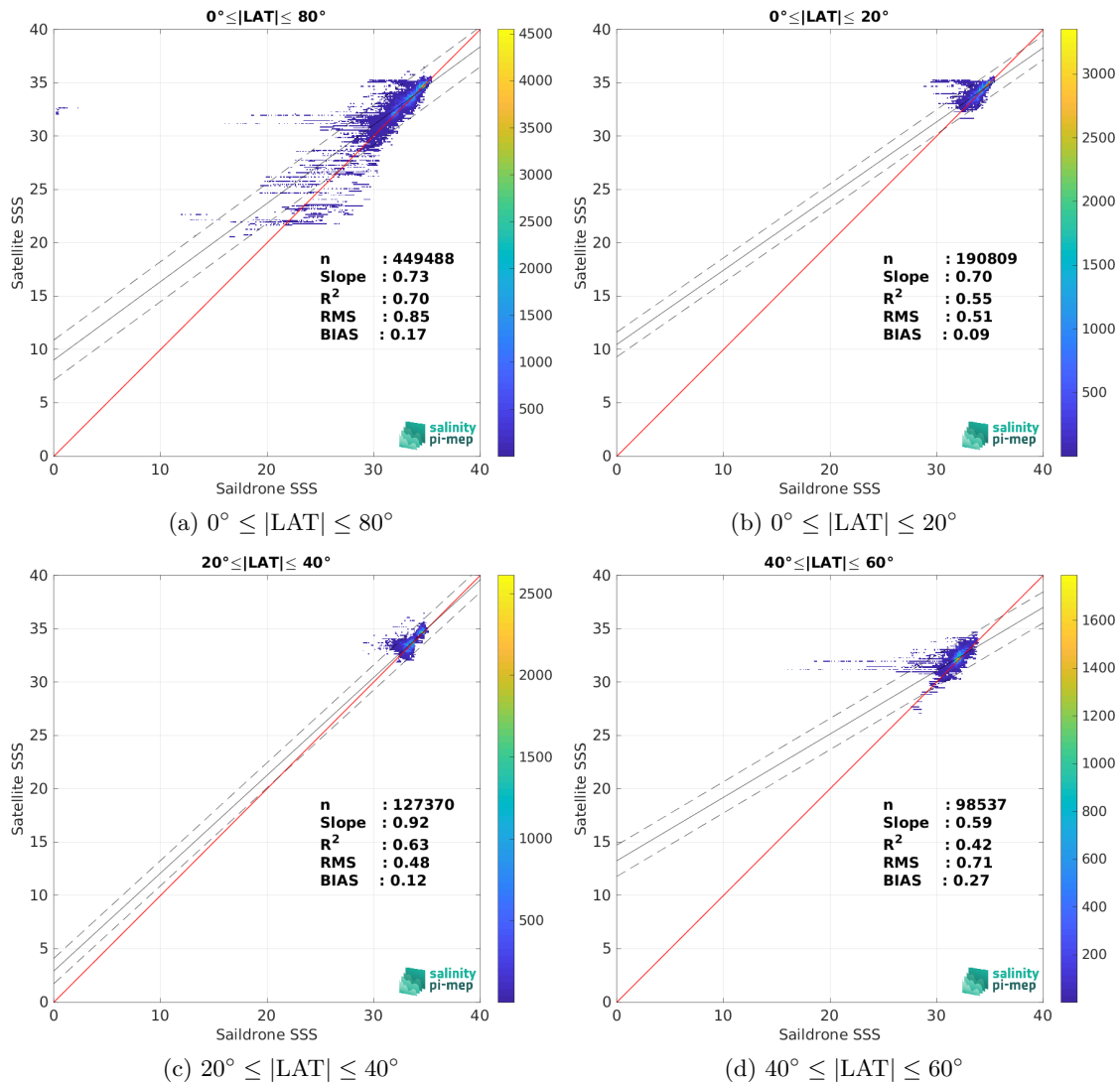
Figure 10: Contour maps of the concentration of SMAP SSS L3 v5.3 - 8-Day running (RSS) SSS (y-axis) versus Sairdrone SSS (x-axis) at match-up pairs for different latitude bands. For each plot, the red line shows x=y . The black thin and dashed lines indicate a linear fit through the data cloud and the \pm 95\% confidence levels, respectively. The number match-up pairs n , the slope and R^2 coefficient of the linear fit, the root mean square (RMS) and the mean bias between satellite and in situ data are indicated for each latitude band in each plots.
