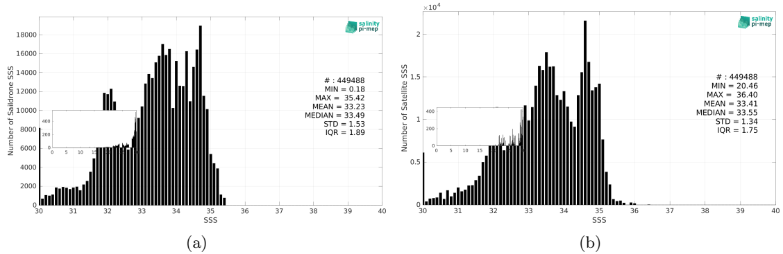
Figure 3: Histograms of SSS from Sairdrone (a) and SMAP SSS L3 v5.3 - 8-Day running (RSS) (b) considering all match-up pairs per bins of 0.1 over the North Pacific Ocean Pi-MEP region and for the full satellite product period.
