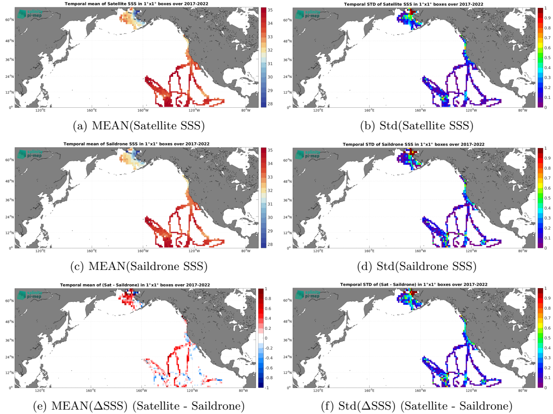
Figure 7: Temporal mean (left) and Std (right) of SSS from SMAP SSS L3 v5.3 - 8-Day running (RSS) (top), Saildrone (middle), and of \Delta SSS (Satellite - Saildrone). Only match-up pairs are used to generate these maps.
