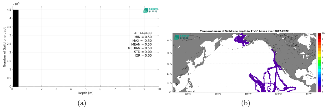
Figure 4: Histograms of the depth of the upper level SSS measurements from Sairdrone in the Match-up DataBase for the North Pacific Ocean Pi-MEP region (a) and temporal mean spatial distribution of pressure of the in situ SSS data over 1^\circ \times 1^\circ boxes and for the full satellite product period (b).
