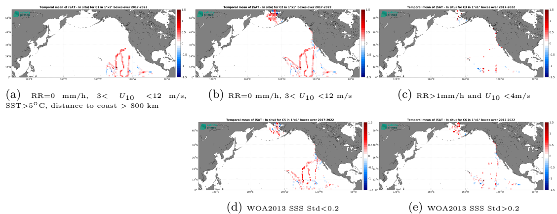
Figure 14: Temporal mean gridded over spatial boxes of size 1^\circ \times 1^\circ of \Delta SSS (SMAP SSS L3 v5.3 - 8-Day running (RSS) - Sairdrone) for 5 different subdatasets corresponding to:RR=0 mm/h, 3 < U_{10} < 12 m/s, SST >5^\circ C, distance to coast > 800 km (a), RR=0 mm/h, 3 < U_{10} < 12 m/s (b), RR >1 mm/h and U_{10} < 4 m/s (c), WOA2013 SSS Std <0.2 (d), WOA2013 SSS Std >0.2 (e).
