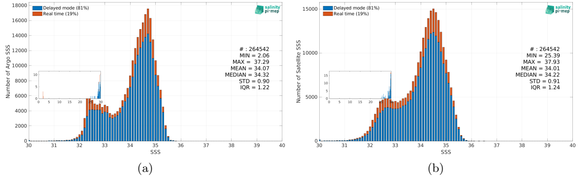
Figure 3: Histograms of SSS from Argo (a) and SMAP SSS L3 v5.3 - 8-Day running (RSS) (b) considering all match-up pairs per bins of 0.1 over the North Pacific Ocean Pi-MEP region and for the full satellite product period.
