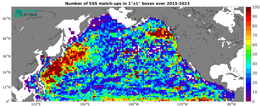
Figure 5: Number of SSS match-ups between Argo SSS and the SMAP SSS L3 v5.3 - 8-Day running (RSS) SSS product for the North Pacific Ocean Pi-MEP region over 1^\circ \times 1^\circ boxes and for the full satellite product period.
