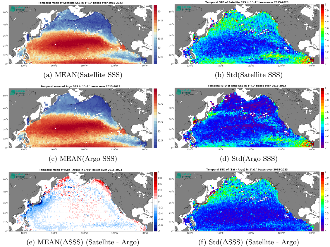
Figure 7: Temporal mean (left) and Std (right) of SSS from SMAP SSS L3 v5.3 - 8-Day running (RSS) (top), Argo (middle), and of \Delta\text{SSS} (Satellite - Argo). Only match-up pairs are used to generate these maps.
