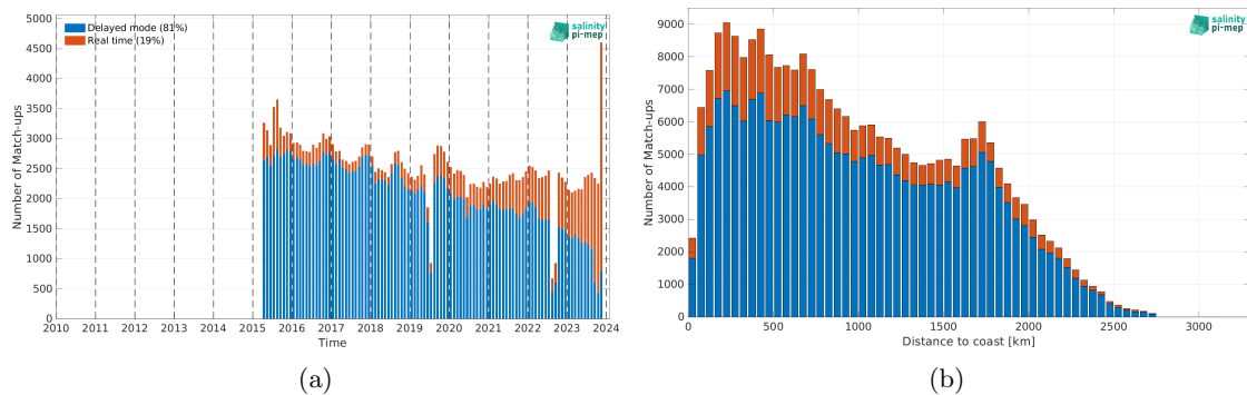
Figure 2: Number of match-ups between Argo and SMAP SSS L3 v5.3 - 8-Day running (RSS) SSS as a function of time (a) and as function of the distance to coast (b) over the North Pacific Ocean Pi-MEP region and for the full satellite product period.
