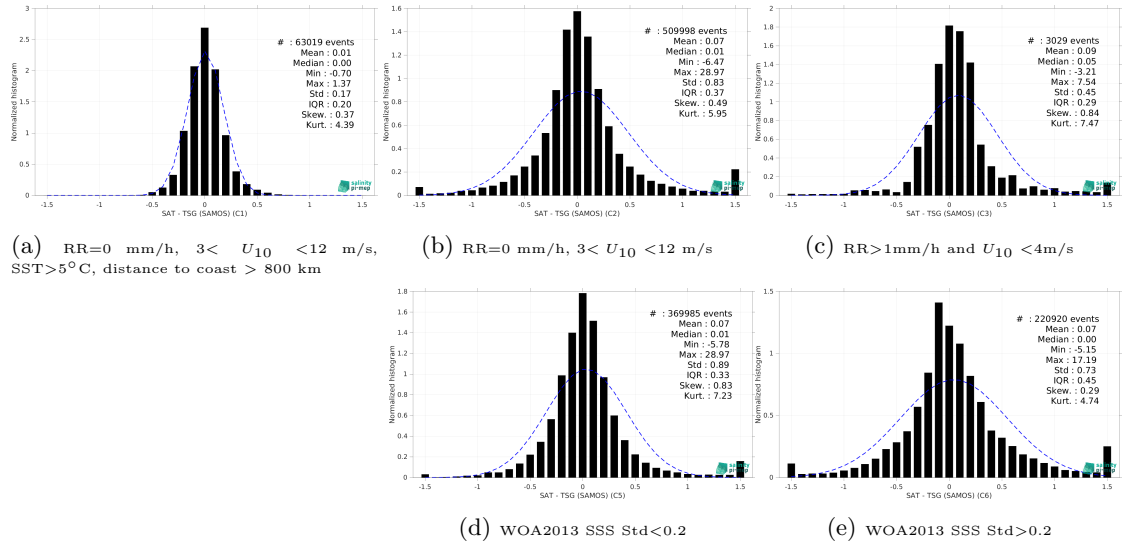
Figure 15: Normalized histogram of \Delta SSS (SMAP SSS L3 v5.3 - Monthly (RSS) - TSG (SAMOS)) for 5 different subdatasets corresponding to: RR=0 mm/h, 3 < U_{10} < 12 m/s, SST>5°C, distance to coast > 800 km (a), RR=0 mm/h, 3 < U_{10} < 12 m/s (b), RR>1mm/h and U_{10} < 4 m/s (c), WOA2013 SSS Std<0.2 (d), WOA2013 SSS Std>0.2 (e).
