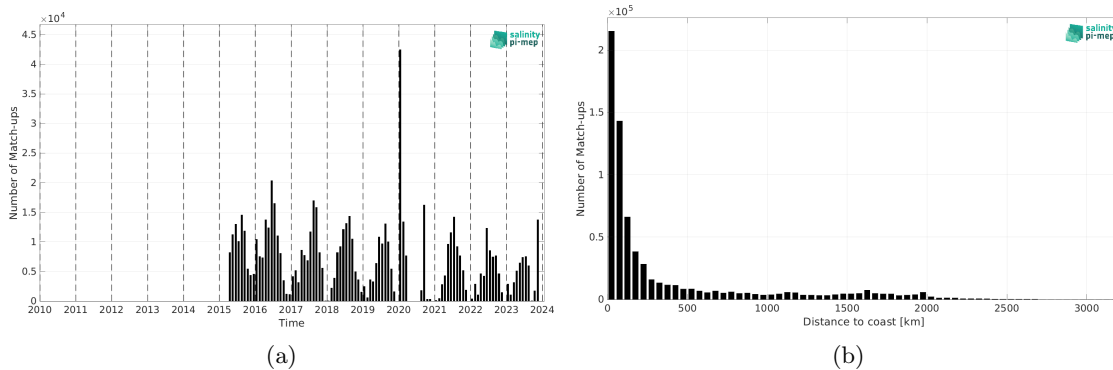
Figure 2: Number of match-ups between TSG (SAMOS) and SMAP SSS L3 v5.3 - Monthly (RSS) SSS as a function of time (a) and as function of the distance to coast (b) over the North Pacific Ocean Pi-MEP region and for the full satellite product period.
