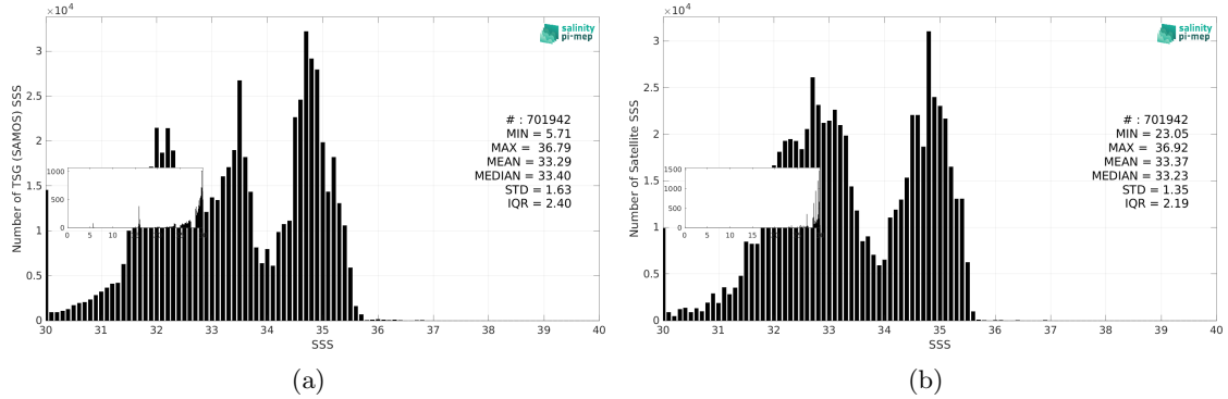
Figure 3: Histograms of SSS from TSG (SAMOS) (a) and SMAP SSS L3 v5.3 - Monthly (RSS) (b) considering all match-up pairs per bins of 0.1 over the North Pacific Ocean Pi-MEP region and for the full satellite product period.
