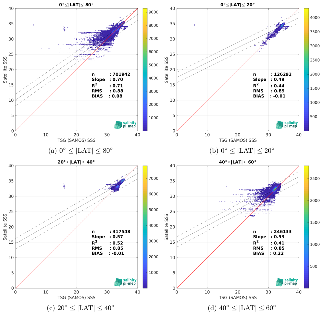
Figure 10: Contour maps of the concentration of SMAP SSS L3 v5.3 - Monthly (RSS) SSS (y-axis) versus TSG (SAMOS) SSS (x-axis) at match-up pairs for different latitude bands. For each plot, the red line shows x=y . The black thin and dashed lines indicate a linear fit through the data cloud and the \pm 95\% confidence levels, respectively. The number match-up pairs n , the slope and R^2 coefficient of the linear fit, the root mean square (RMS) and the mean bias between satellite and in situ data are indicated for each latitude band in each plots.
