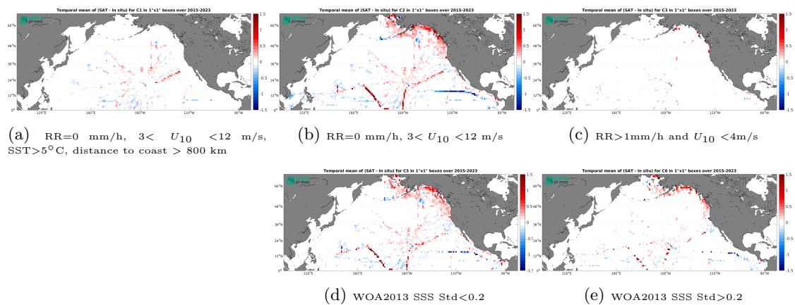
Figure 14: Temporal mean gridded over spatial boxes of size 1^\circ \times 1^\circ of \Delta SSS (SMAP SSS L3 v5.3 - Monthly (RSS) - TSG (SAMOS)) for 5 different subdatasets corresponding to:RR=0 mm/h, 3 < U_{10} < 12 m/s, SST > 5^\circ\text{C} , distance to coast > 800 km (a), RR=0 mm/h, 3 < U_{10} < 12 m/s (b), RR > 1 mm/h and U_{10} < 4 m/s (c), WOA2013 SSS Std < 0.2 (d), WOA2013 SSS Std > 0.2 (e).
