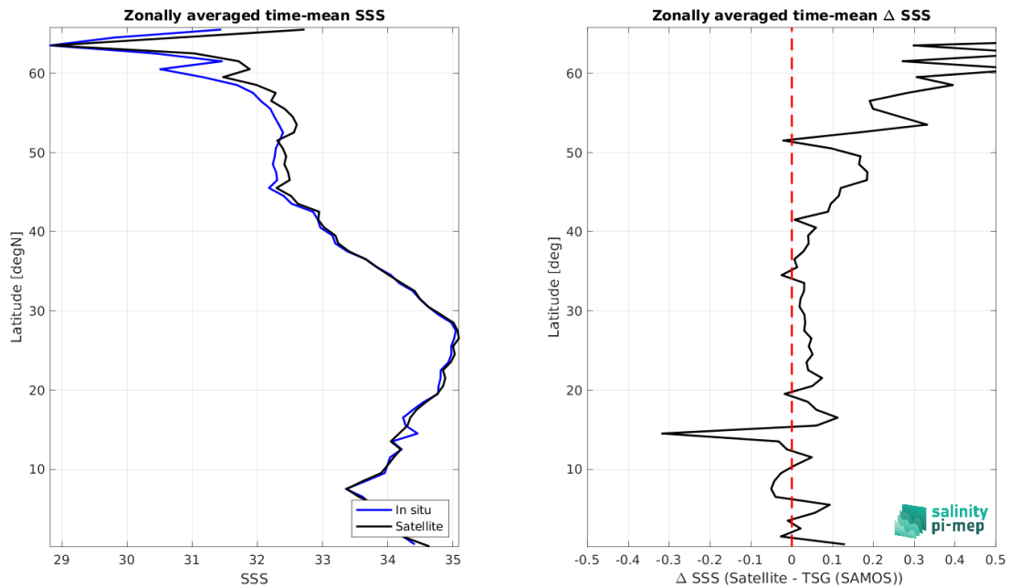
Figure 9: Left panel: Zonal mean SSS from SMAP SSS L3 v5.3 - Monthly (RSS) satellite product (black) and from TSG (SAMOS) (blue). Right panel: Zonal mean of \Delta SSS (Satellite - TSG (SAMOS)) for all the collected Pi-MEP match-up pairs estimated over the full satellite product period.
