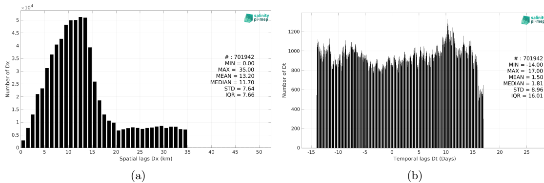
Figure 6: Histograms of the spatial (a) and temporal (b) lags between the location/time of the TSG (SAMOS) measurement and the date of the corresponding SMAP SSS L3 v5.3 - Monthly (RSS) SSS pixel.
