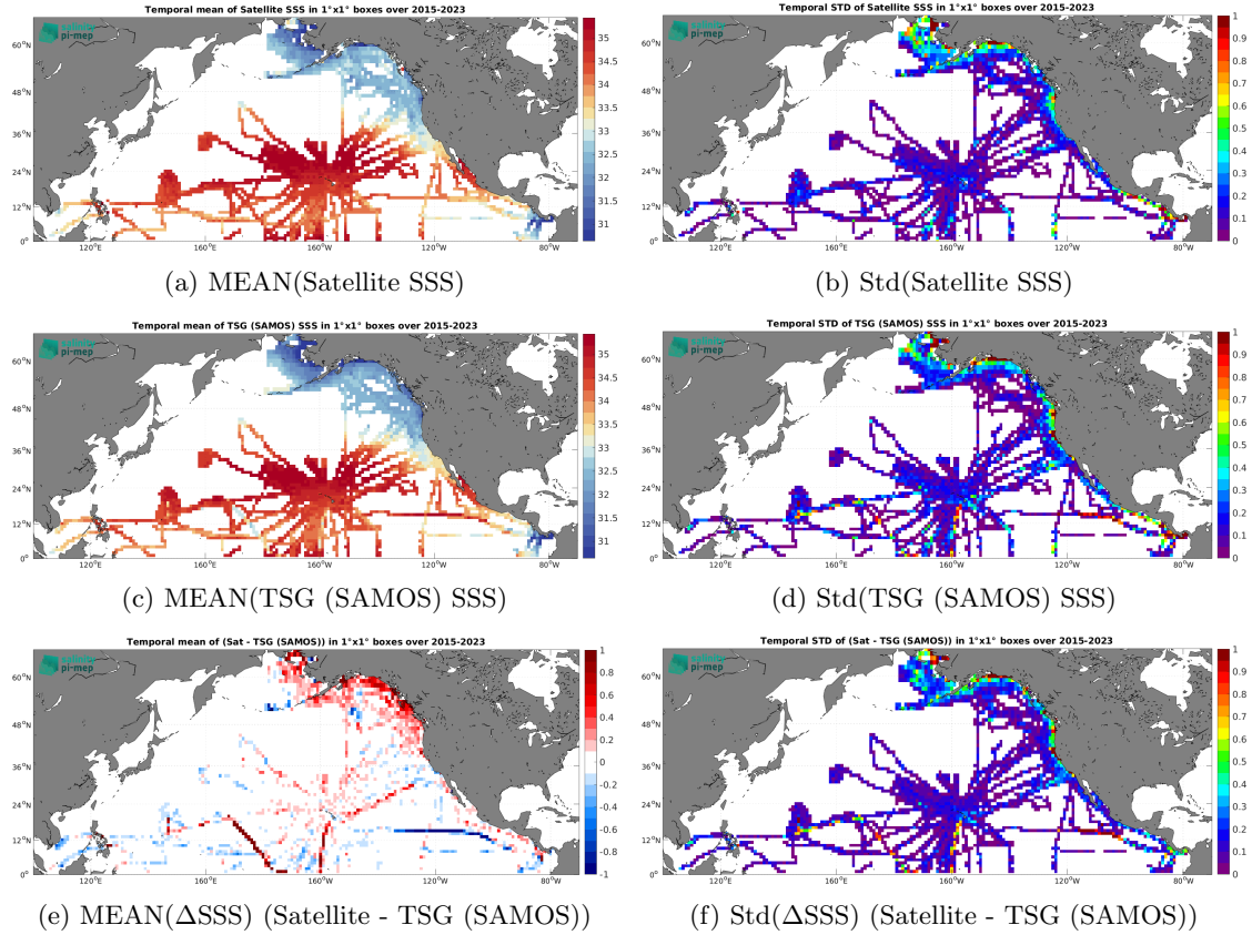
Figure 7: Temporal mean (left) and Std (right) of SSS from SMAP SSS L3 v5.3 - Monthly (RSS) (top), TSG (SAMOS) (middle), and of \Delta\text{SSS} (Satellite - TSG (SAMOS)). Only match-up pairs are used to generate these maps.
