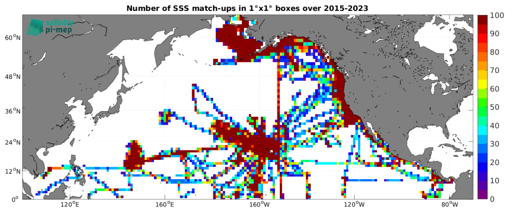
Figure 5: Number of SSS match-ups between TSG (SAMOS) SSS and the SMAP SSS L3 v5.3 - Monthly (RSS) SSS product for the North Pacific Ocean Pi-MEP region over 1^\circ \times 1^\circ boxes and for the full satellite product period.
