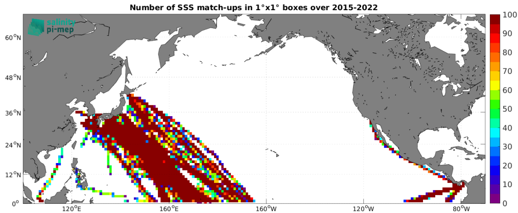
Figure 5: Number of SSS match-ups between TSG (LEGOS-DM) SSS and the SMAP SSS L3 v5.3 - Monthly (RSS) SSS product for the North Pacific Ocean Pi-MEP region over 1^\circ \times 1^\circ boxes and for the full satellite product period.
