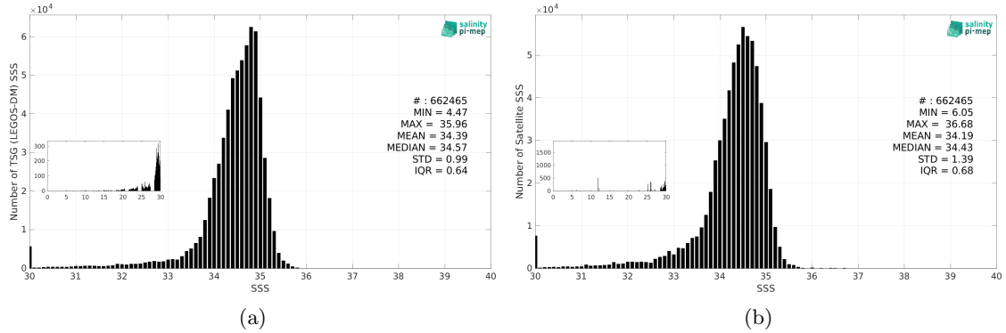
Figure 3: Histograms of SSS from TSG (LEGOS-DM) (a) and SMAP SSS L3 v5.3 - Monthly (RSS) (b) considering all match-up pairs per bins of 0.1 over the North Pacific Ocean Pi-MEP region and for the full satellite product period.
