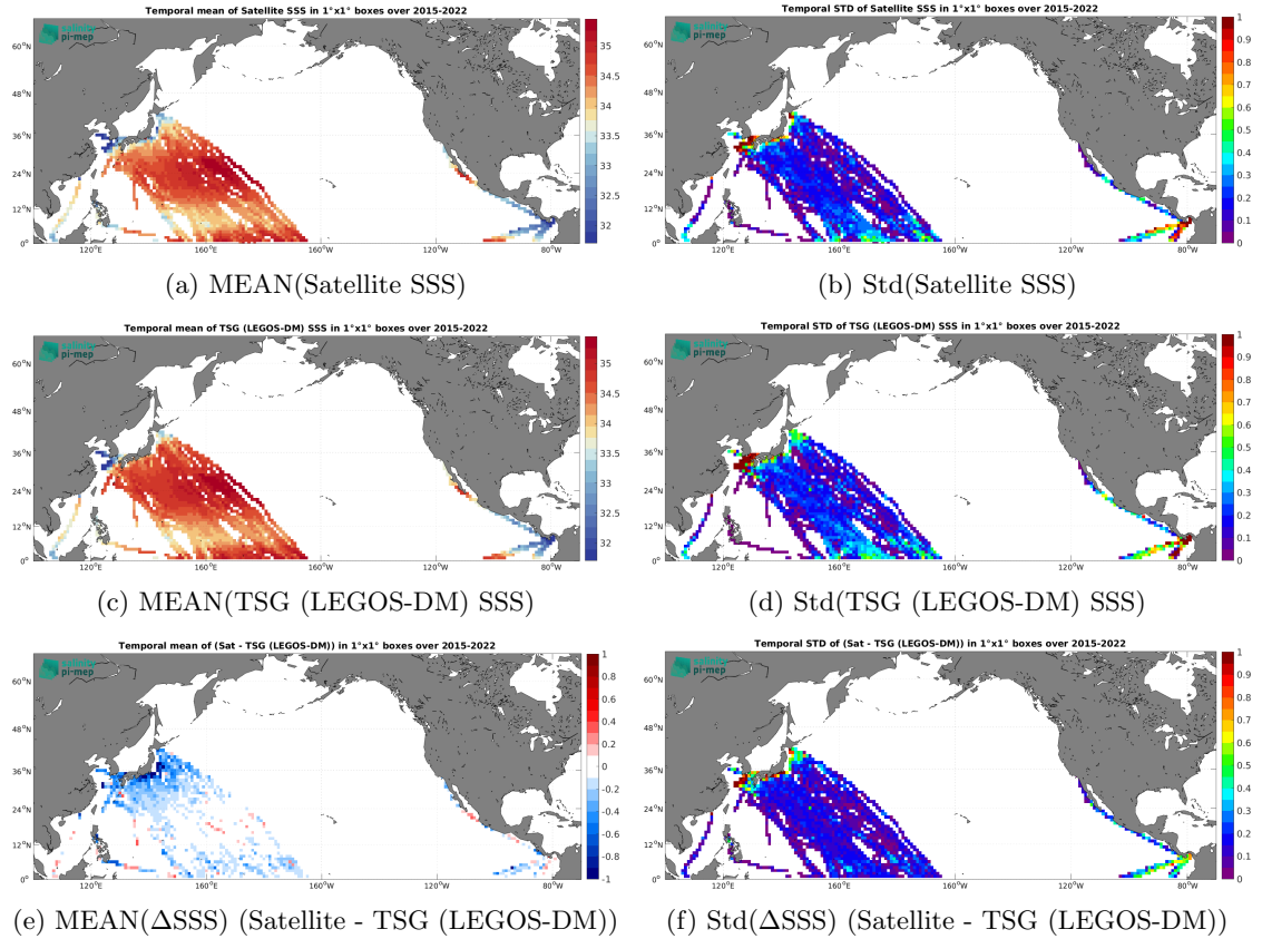
Figure 7: Temporal mean (left) and Std (right) of SSS from SMAP SSS L3 v5.3 - Monthly (RSS) (top), TSG (LEGOS-DM) (middle), and of \Delta\text{SSS} (Satellite - TSG (LEGOS-DM)). Only match-up pairs are used to generate these maps.
