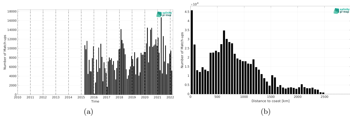
Figure 2: Number of match-ups between TSG (LEGOS-DM) and SMAP SSS L3 v5.3 - Monthly (RSS) SSS as a function of time (a) and as function of the distance to coast (b) over the North Pacific Ocean Pi-MEP region and for the full satellite product period.
