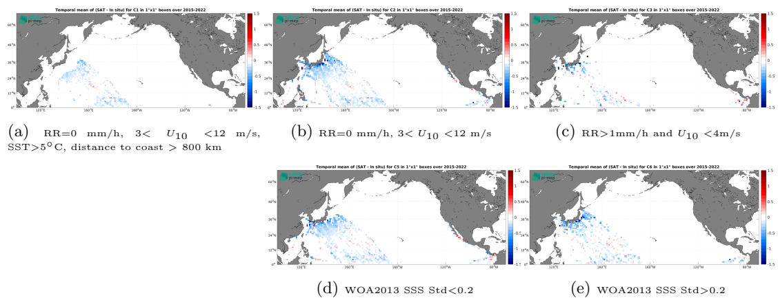
Figure 14: Temporal mean gridded over spatial boxes of size 1^\circ \times 1^\circ of \Delta\text{SSS} (SMAP SSS L3 v5.3 - Monthly (RSS) - TSG (LEGOS-DM)) for 5 different subdatasets corresponding to: RR=0 mm/h, 3 < U_{10} < 12 m/s, SST > 5°C, distance to coast > 800 km (a), RR=0 mm/h, 3 < U_{10} < 12 m/s (b), RR > 1mm/h and U_{10} < 4 m/s (c), WOA2013 SSS Std < 0.2 (d), WOA2013 SSS Std > 0.2 (e).
