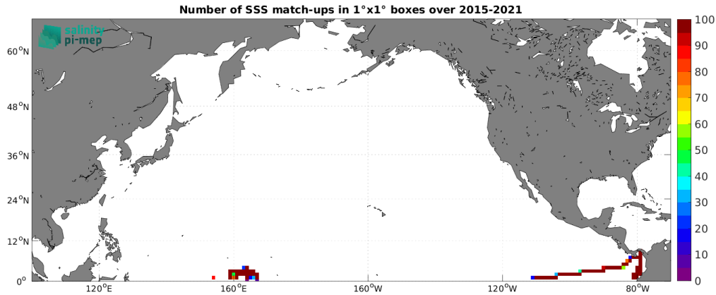
Figure 5: Number of SSS match-ups between TSG (GOSUD-Research-vessel) SSS and the SMAP SSS L3 v5.3 - Monthly (RSS) SSS product for the North Pacific Ocean Pi-MEP region over 1^\circ \times 1^\circ boxes and for the full satellite product period.
