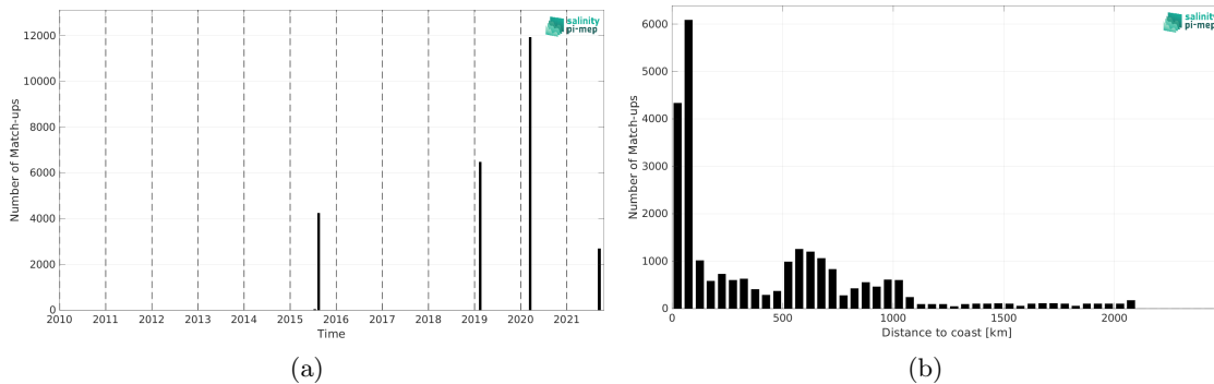
Figure 2: Number of match-ups between TSG (GOSUD-Research-vessel) and SMAP SSS L3 v5.3 - Monthly (RSS) SSS as a function of time (a) and as function of the distance to coast (b) over the North Pacific Ocean Pi-MEP region and for the full satellite product period.
