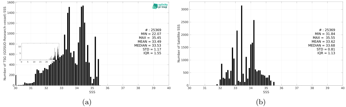
Figure 3: Histograms of SSS from TSG (GOSUD-Research-vessel) (a) and SMAP SSS L3 v5.3 - Monthly (RSS) (b) considering all match-up pairs per bins of 0.1 over the North Pacific Ocean Pi-MEP region and for the full satellite product period.
