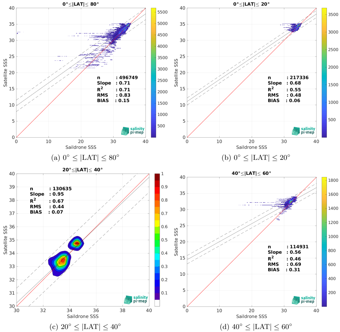
Figure 10: Contour maps of the concentration of SMAP SSS L3 v5.3 - Monthly (RSS) SSS (y-axis) versus Saildrone SSS (x-axis) at match-up pairs for different latitude bands. For each plot, the red line shows x=y . The black thin and dashed lines indicate a linear fit through the data cloud and the \pm 95\% confidence levels, respectively. The number match-up pairs n , the slope and R^2 coefficient of the linear fit, the root mean square (RMS) and the mean bias between satellite and in situ data are indicated for each latitude band in each plots.
