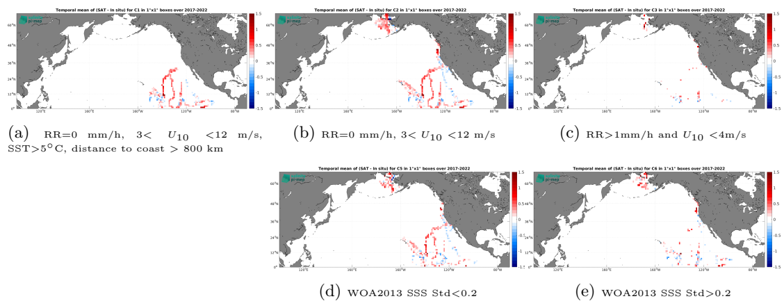
Figure 14: Temporal mean gridded over spatial boxes of size 1^\circ \times 1^\circ of \Delta SSS (SMAP SSS L3 v5.3 - Monthly (RSS) - Saifdrone) for 5 different subdatasets corresponding to:RR=0 mm/h, 3 < U_{10} < 12 m/s, SST >5^\circ\text{C} , distance to coast > 800 km (a), RR=0 mm/h, 3 < U_{10} < 12 m/s (b), RR >1 mm/h and U_{10} < 4 m/s (c), WOA2013 SSS Std <0.2 (d), WOA2013 SSS Std >0.2 (e).
