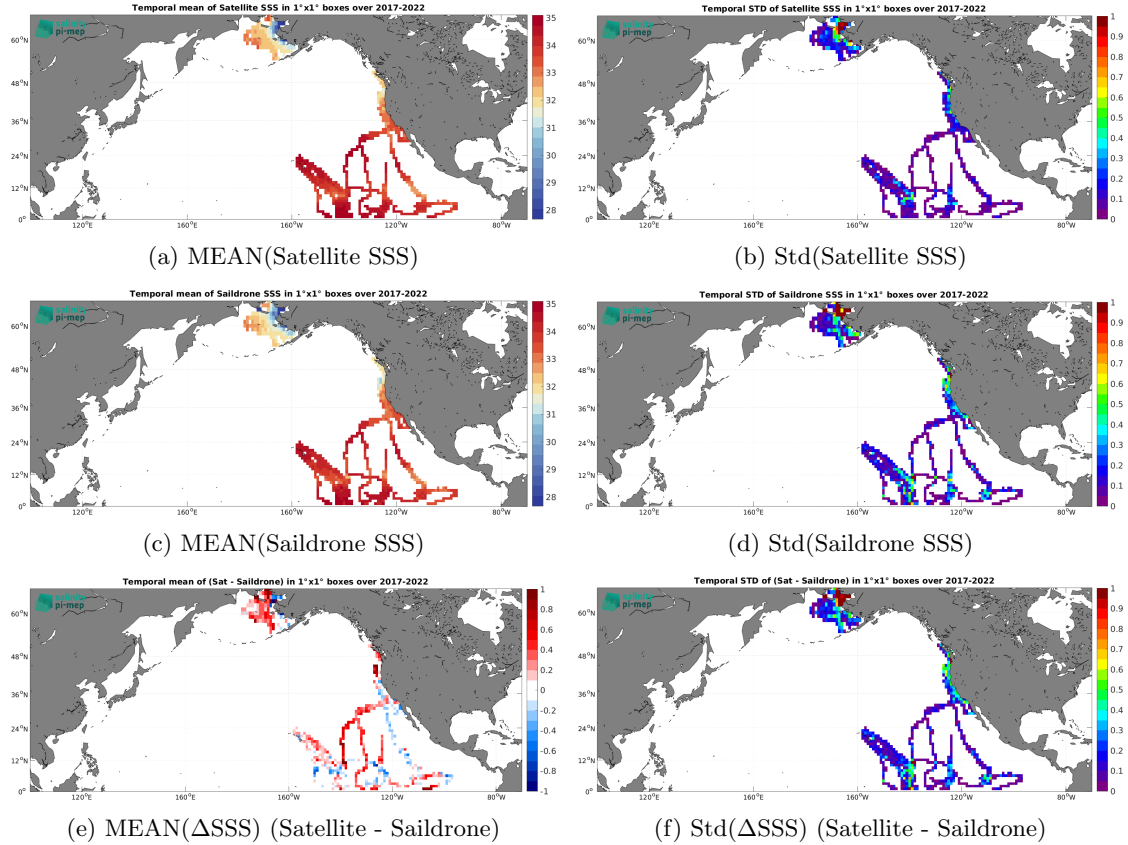
Figure 7: Temporal mean (left) and Std (right) of SSS from SMAP SSS L3 v5.3 - Monthly (RSS) (top), Saildrone (middle), and of \Delta\text{SSS} (Satellite - Saildrone). Only match-up pairs are used to generate these maps.
