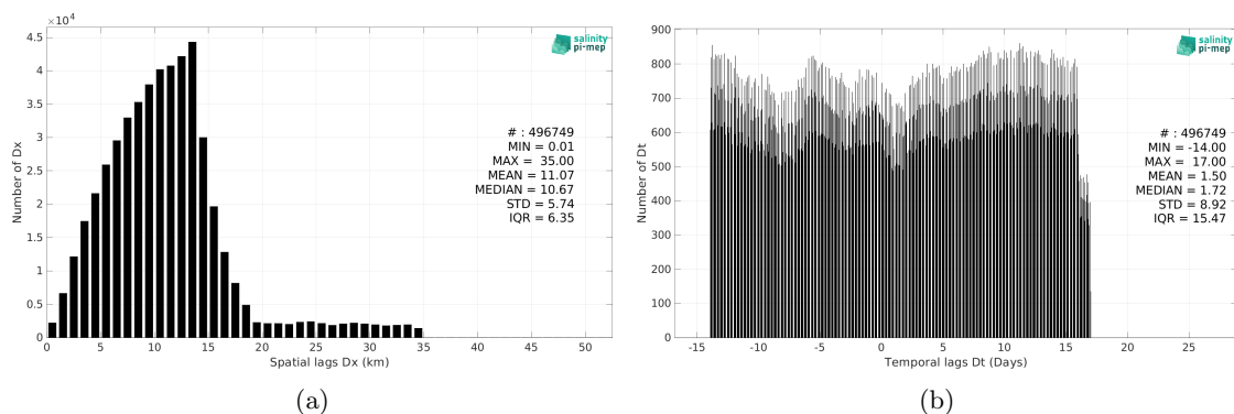
Figure 6: Histograms of the spatial (a) and temporal (b) lags between the location/time of the Saildrone measurement and the date of the corresponding SMAP SSS L3 v5.3 - Monthly (RSS) SSS pixel.
