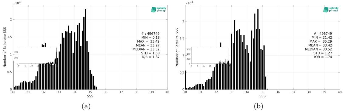
Figure 3: Histograms of SSS from Saildrone (a) and SMAP SSS L3 v5.3 - Monthly (RSS) (b) considering all match-up pairs per bins of 0.1 over the North Pacific Ocean Pi-MEP region and for the full satellite product period.
