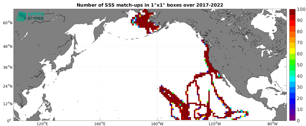
Figure 5: Number of SSS match-ups between Saildrone SSS and the SMAP SSS L3 v5.3 - Monthly (RSS) SSS product for the North Pacific Ocean Pi-MEP region over 1^\circ \times 1^\circ boxes and for the full satellite product period.
