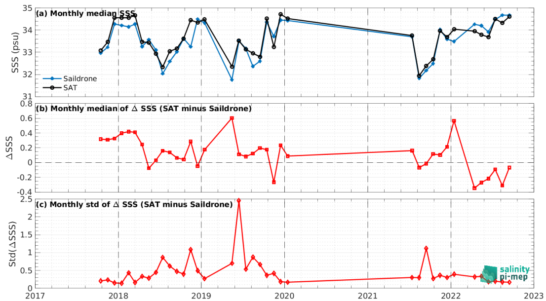
Figure 8: Time series of the monthly median SSS (top), median of \Delta SSS (Satellite - Saildrone) and Std of \Delta SSS (Satellite - Saildrone) over the North Pacific Ocean Pi-MEP region considering all match-ups collected by the Pi-MEP.
