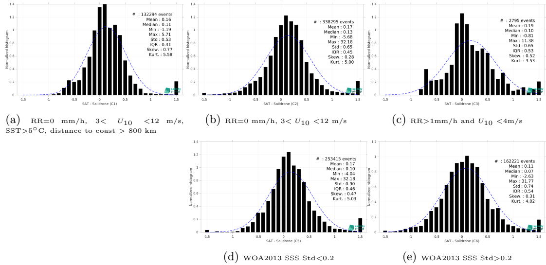
Figure 15: Normalized histogram of \Delta SSS (SMAP SSS L3 v5.3 - Monthly (RSS) - Saildrone) for 5 different subdatasets corresponding to: RR=0 mm/h, 3 < U_{10} < 12 m/s, SST>5°C, distance to coast > 800 km (a), RR=0 mm/h, 3 < U_{10} < 12 m/s (b), RR>1mm/h and U_{10} < 4 m/s (c), WOA2013 SSS Std<0.2 (d), WOA2013 SSS Std>0.2 (e).
