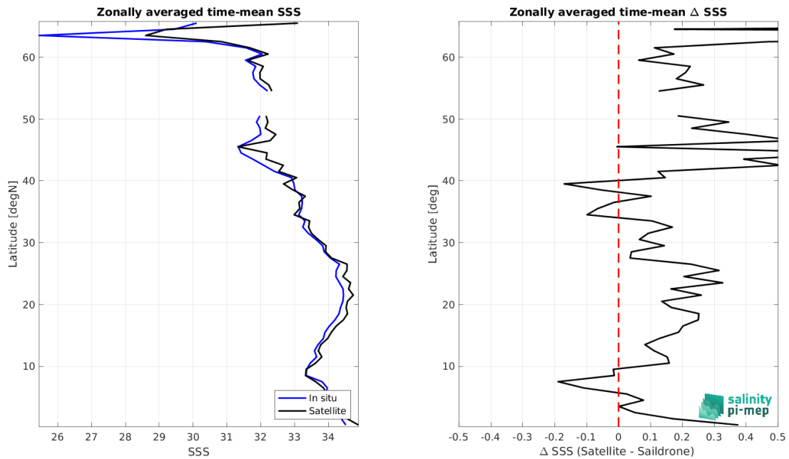
Figure 9: Left panel: Zonal mean SSS from SMAP SSS L3 v5.3 - Monthly (RSS) satellite product (black) and from Saildrone (blue). Right panel: Zonal mean of \Delta SSS (Satellite - Saildrone) for all the collected Pi-MEP match-up pairs estimated over the full satellite product period.
