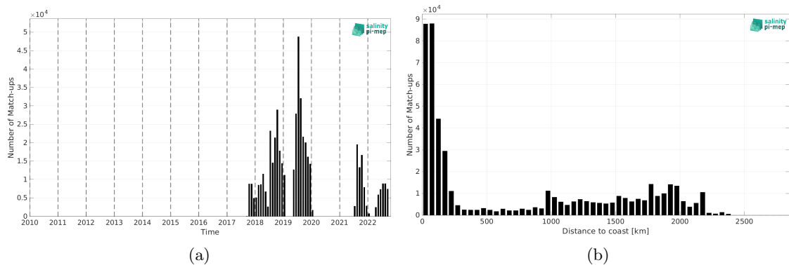
Figure 2: Number of match-ups between Saildrone and SMAP SSS L3 v5.3 - Monthly (RSS) SSS as a function of time (a) and as function of the distance to coast (b) over the North Pacific Ocean Pi-MEP region and for the full satellite product period.
