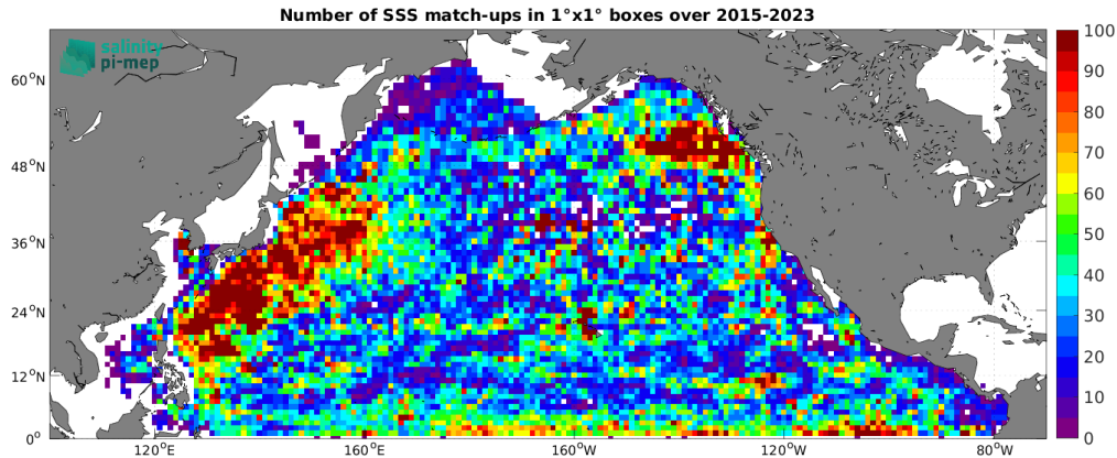
Figure 5: Number of SSS match-ups between Argo SSS and the SMAP SSS L3 v5.3 - Monthly (RSS) SSS product for the North Pacific Ocean Pi-MEP region over 1^\circ \times 1^\circ boxes and for the full satellite product period.
