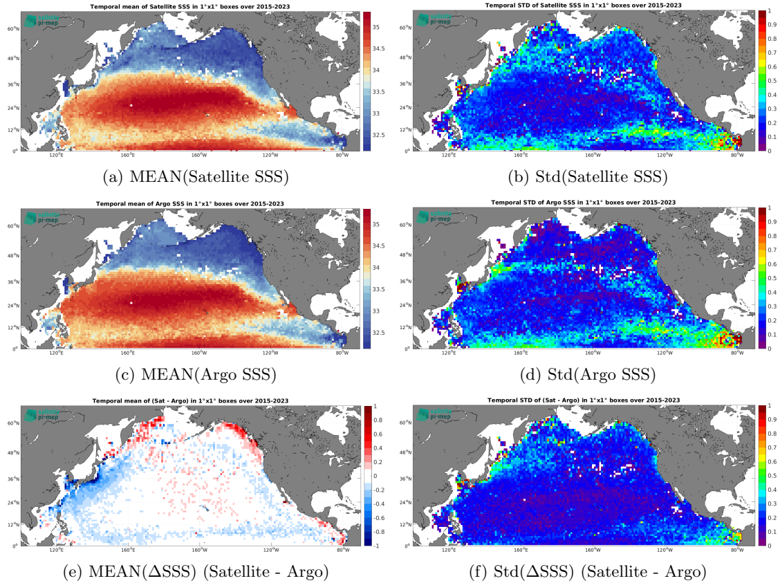
Figure 7: Temporal mean (left) and Std (right) of SSS from SMAP SSS L3 v5.3 - Monthly (RSS) (top), Argo (middle), and of \Delta\text{SSS} (Satellite - Argo). Only match-up pairs are used to generate these maps.
