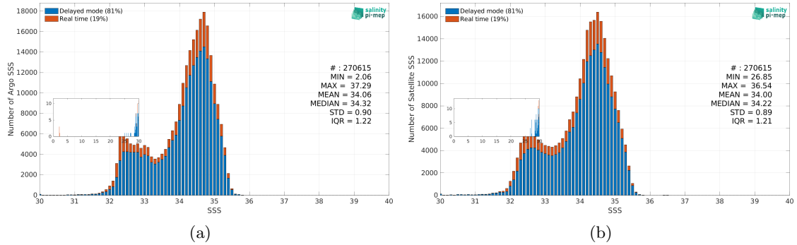
Figure 3: Histograms of SSS from Argo (a) and SMAP SSS L3 v5.3 - Monthly (RSS) (b) considering all match-up pairs per bins of 0.1 over the North Pacific Ocean Pi-MEP region and for the full satellite product period.
