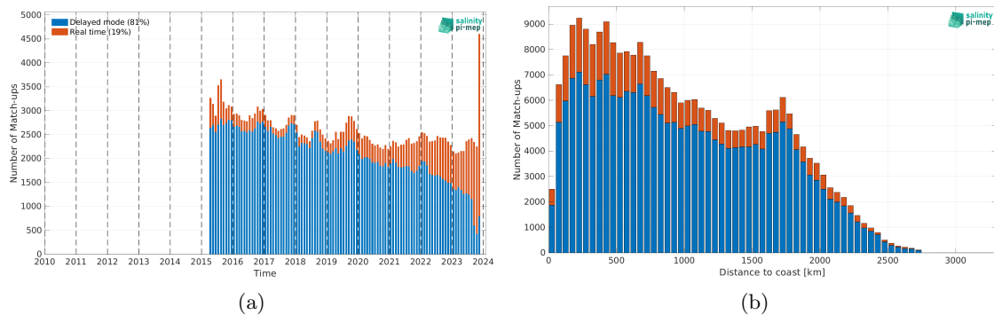
Figure 2: Number of match-ups between Argo and SMAP SSS L3 v5.3 - Monthly (RSS) SSS as a function of time (a) and as function of the distance to coast (b) over the North Pacific Ocean Pi-MEP region and for the full satellite product period.
