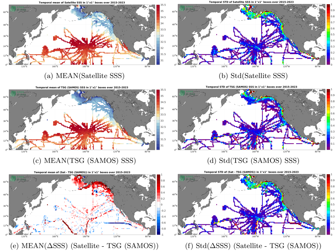
Figure 6: Temporal mean (left) and Std (right) of SSS from SMAP SSS L3 v5 - 8-Day running (RSS) (top), TSG (SAMOS) (middle), and of \Delta SSS (Satellite - TSG (SAMOS)). Only match-up pairs are used to generate these maps.
