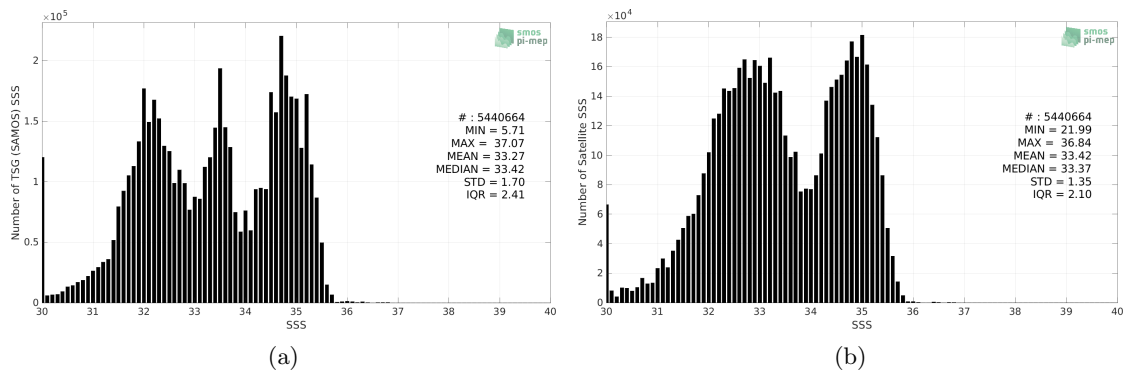
Figure 2: Histograms of SSS from TSG (SAMOS) (a) and SMAP SSS L3 v5 - 8-Day running (RSS) (b) considering all match-up pairs per bins of 0.1 over the North Pacific Ocean Pi-MEP region and for the full satellite product period.
