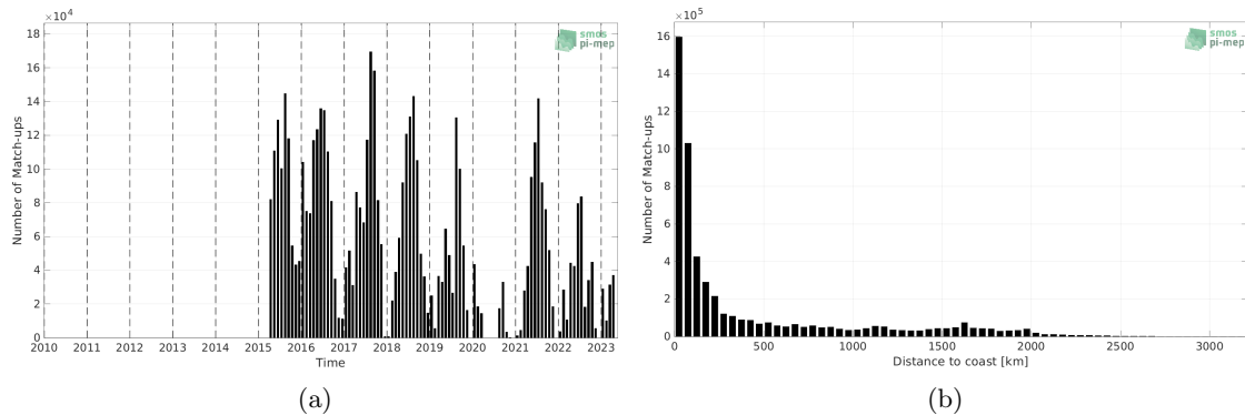
Figure 1: Number of match-ups between TSG (SAMOS) and SMAP SSS L3 v5 - 8-Day running (RSS) SSS as a function of time (a) and as function of the distance to coast (b) over the North Pacific Ocean Pi-MEP region and for the full satellite product period.
