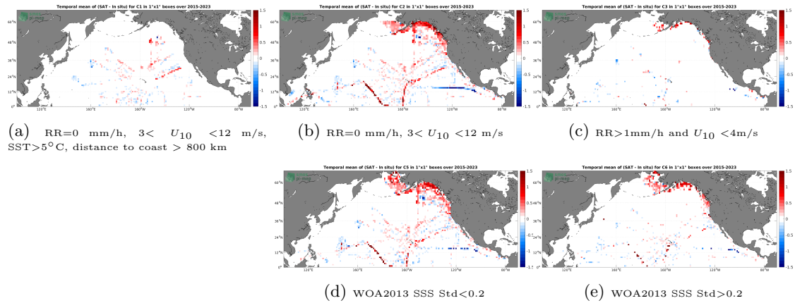
Figure 12: Temporal mean gridded over spatial boxes of size 1^\circ \times 1^\circ of \Delta SSS (SMAP SSS L3 v5 - 8-Day running (RSS) - TSG (SAMOS)) for 5 different subdatasets corresponding to:RR=0 mm/h, 3 < U_{10} < 12 m/s, SST > 5^\circ C , distance to coast > 800 km (a), RR=0 mm/h, 3 < U_{10} < 12 m/s (b), RR >1 mm/h and U_{10} < 4 m/s (c), WOA2013 SSS Std <0.2 (d), WOA2013 SSS Std >0.2 (e).
