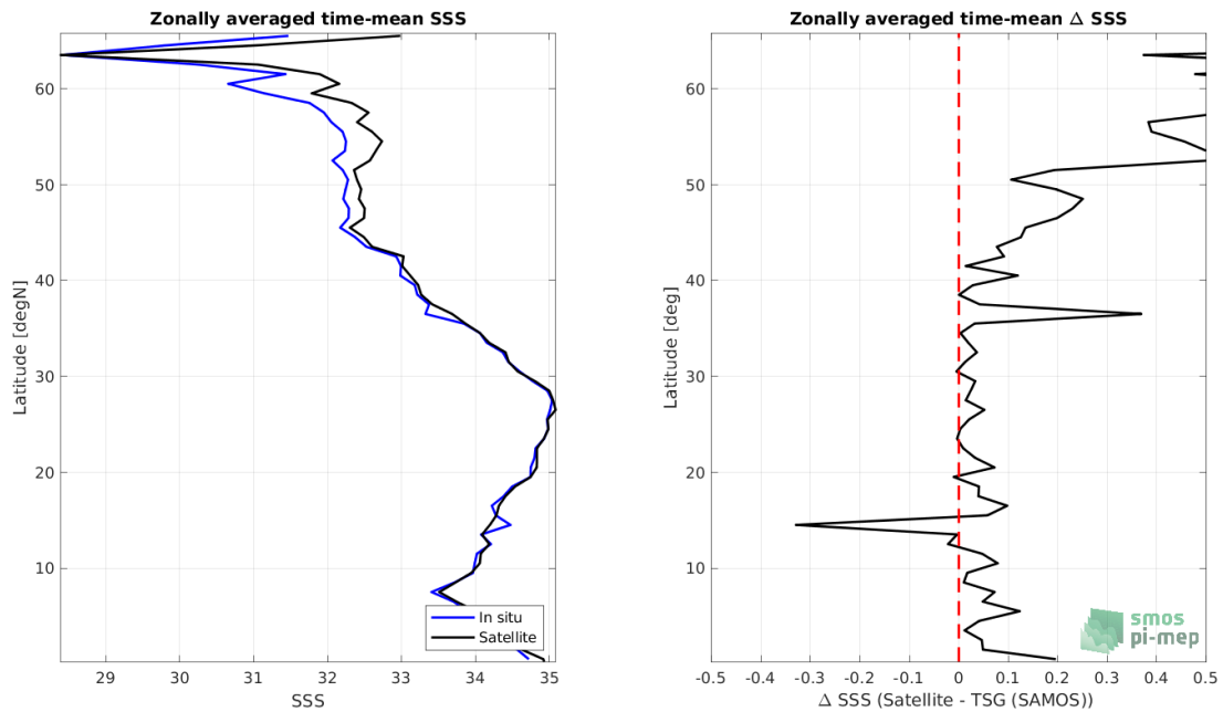
Figure 8: Left panel: Zonal mean SSS from SMAP SSS L3 v5 - 8-Day running (RSS) satellite product (black) and from TSG (SAMOS) (blue). Right panel: Zonal mean of \Delta SSS (Satellite - TSG (SAMOS)) for all the collected Pi-MEP match-up pairs estimated over the full satellite product period.
