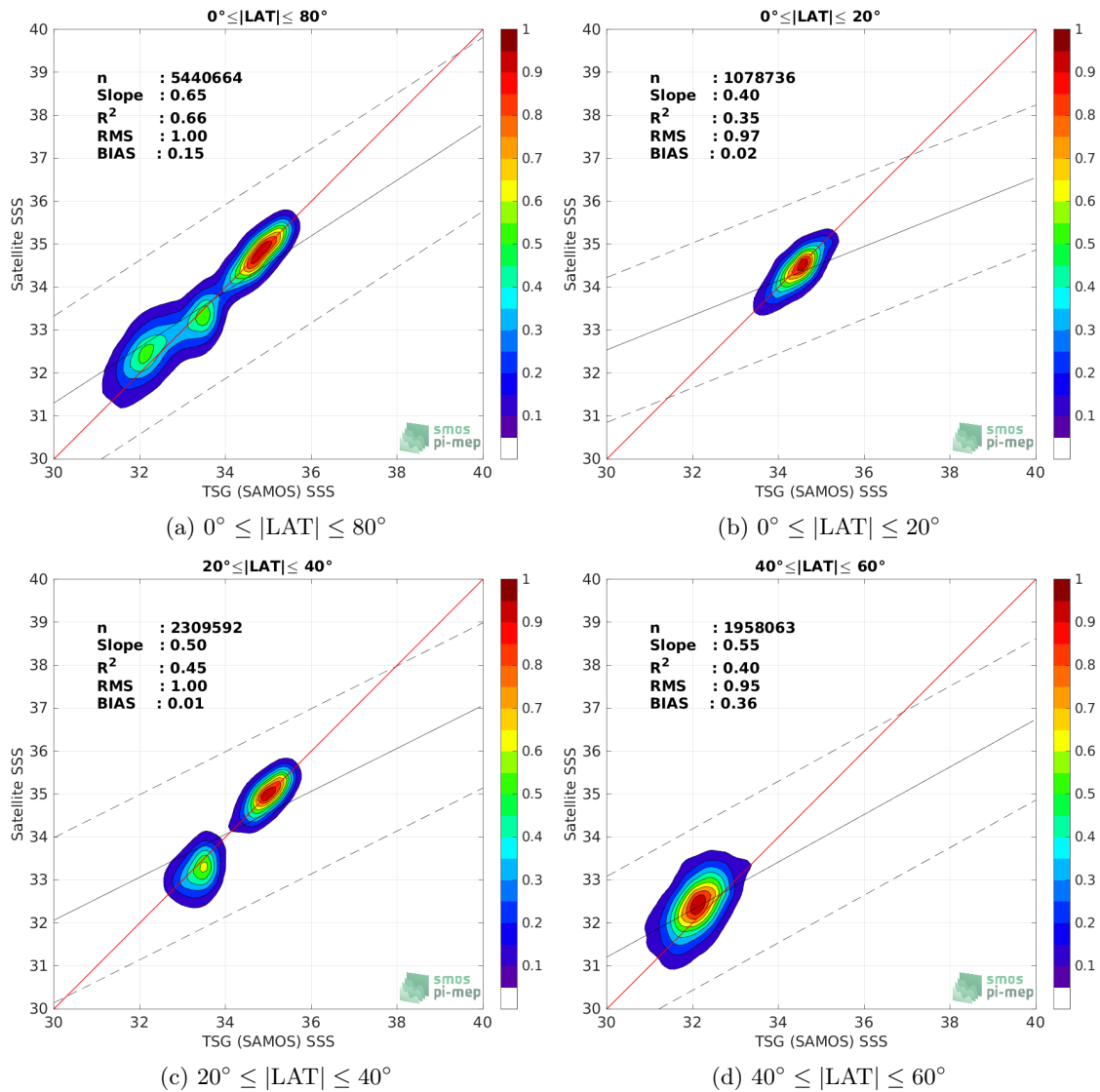
Figure 9: Contour maps of the concentration of SMAP SSS L3 v5 - 8-Day running (RSS) SSS (y-axis) versus TSG (SAMOS) SSS (x-axis) at match-up pairs for different latitude bands. For each plot, the red line shows x=y . The black thin and dashed lines indicate a linear fit through the data cloud and the \pm 95\% confidence levels, respectively. The number match-up pairs n , the slope and R^2 coefficient of the linear fit, the root mean square (RMS) and the mean bias between satellite and in situ data are indicated for each latitude band in each plots.
