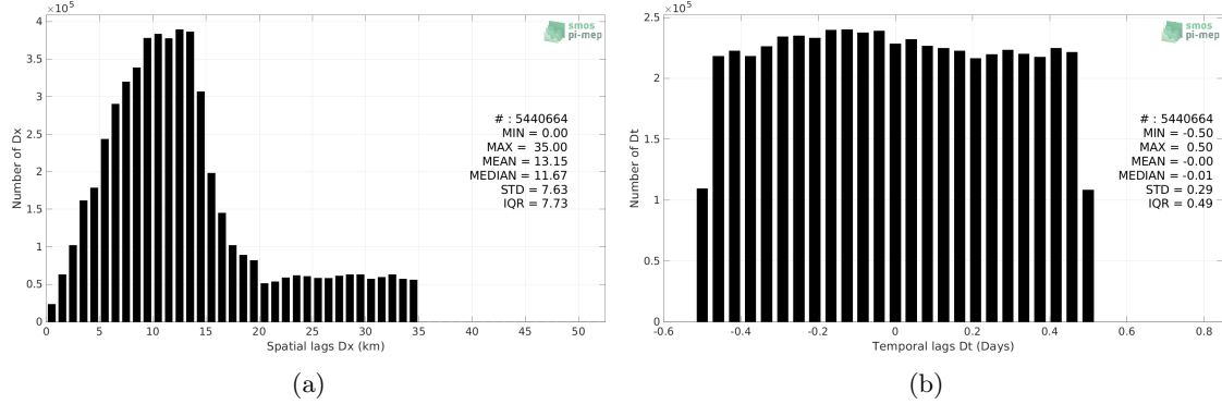
Figure 5: Histograms of the spatial (a) and temporal (b) lags between the location/time of the TSG (SAMOS) measurement and the date of the corresponding SMAP SSS L3 v5 - 8-Day running (RSS) SSS pixel.
