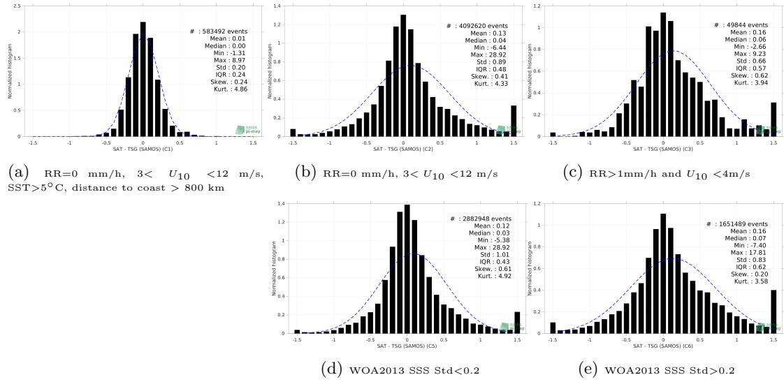
Figure 13: Normalized histogram of \Delta SSS (SMAP SSS L3 v5 - 8-Day running (RSS) - TSG (SAMOS)) for 5 different subdatasets corresponding to: RR=0 mm/h, 3 < U_{10} < 12 m/s, SST>5°C, distance to coast > 800 km (a), RR=0 mm/h, 3 < U_{10} < 12 m/s (b), RR>1mm/h and U_{10} < 4 m/s (c), WOA2013 SSS Std<0.2 (d), WOA2013 SSS Std>0.2 (e).
