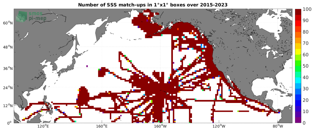
Figure 4: Number of SSS match-ups between TSG (SAMOS) SSS and the SMAP SSS L3 v5 - 8-Day running (RSS) SSS product for the North Pacific Ocean Pi-MEP region over 1^\circ \times 1^\circ boxes and for the full satellite product period.
