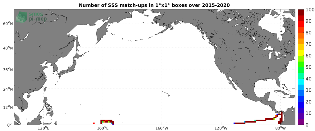
Figure 4: Number of SSS match-ups between TSG (GOSUD-Research-vessel) SSS and the SMAP SSS L3 v5 - 8-Day running (RSS) SSS product for the North Pacific Ocean Pi-MEP region over 1^\circ \times 1^\circ boxes and for the full satellite product period.
