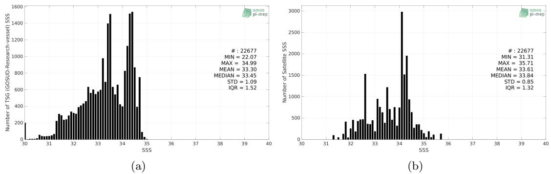
Figure 2: Histograms of SSS from TSG (GOSUD-Research-vessel) (a) and SMAP SSS L3 v5 - 8-Day running (RSS) (b) considering all match-up pairs per bins of 0.1 over the North Pacific Ocean Pi-MEP region and for the full satellite product period.
