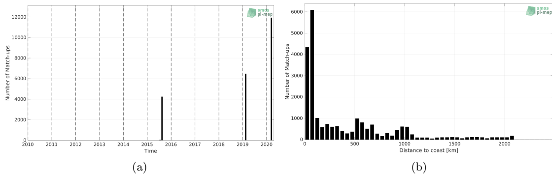
Figure 1: Number of match-ups between TSG (GOSUD-Research-vessel) and SMAP SSS L3 v5 - 8-Day running (RSS) SSS as a function of time (a) and as function of the distance to coast (b) over the North Pacific Ocean Pi-MEP region and for the full satellite product period.
