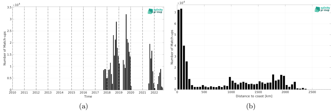
Figure 1: Number of match-ups between Saildrone and SMAP SSS L3 v5 - 8-Day running (RSS) SSS as a function of time (a) and as function of the distance to coast (b) over the North Pacific Ocean Pi-MEP region and for the full satellite product period.
