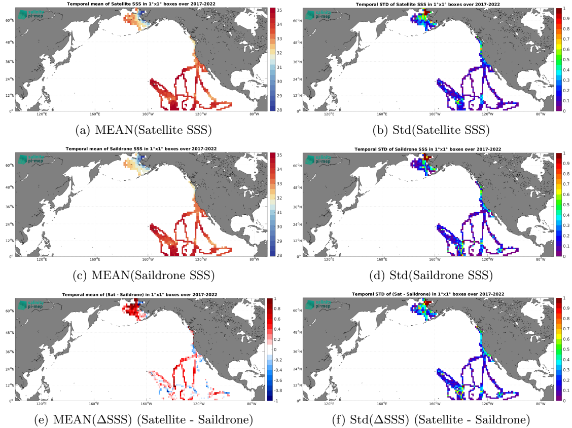
Figure 6: Temporal mean (left) and Std (right) of SSS from SMAP SSS L3 v5 - 8-Day running (RSS) (top), Saildrone (middle), and of \Delta SSS (Satellite - Saildrone). Only match-up pairs are used to generate these maps.
