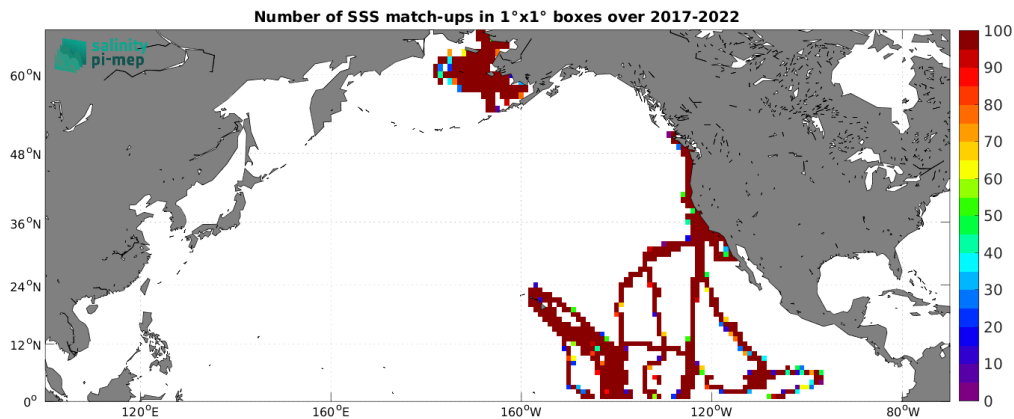
Figure 4: Number of SSS match-ups between Saildrone SSS and the SMAP SSS L3 v5 - 8-Day running (RSS) SSS product for the North Pacific Ocean Pi-MEP region over 1^\circ \times 1^\circ boxes and for the full satellite product period.
