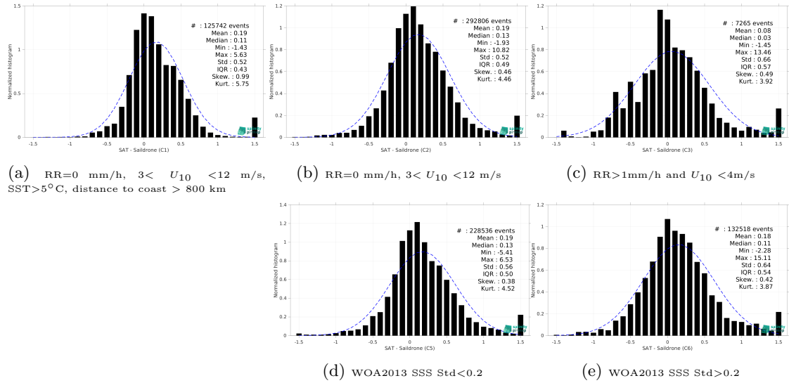
Figure 13: Normalized histogram of \Delta SSS (SMAP SSS L3 v5 - 8-Day running (RSS) - Sairdrome) for 5 different subdatasets corresponding to: RR=0 mm/h, 3 < U_{10} < 12 m/s, SST > 5°C, distance to coast > 800 km (a), RR=0 mm/h, 3 < U_{10} < 12 m/s (b), RR > 1mm/h and U_{10} < 4 m/s (c), WOA2013 SSS Std < 0.2 (d), WOA2013 SSS Std > 0.2 (e).
