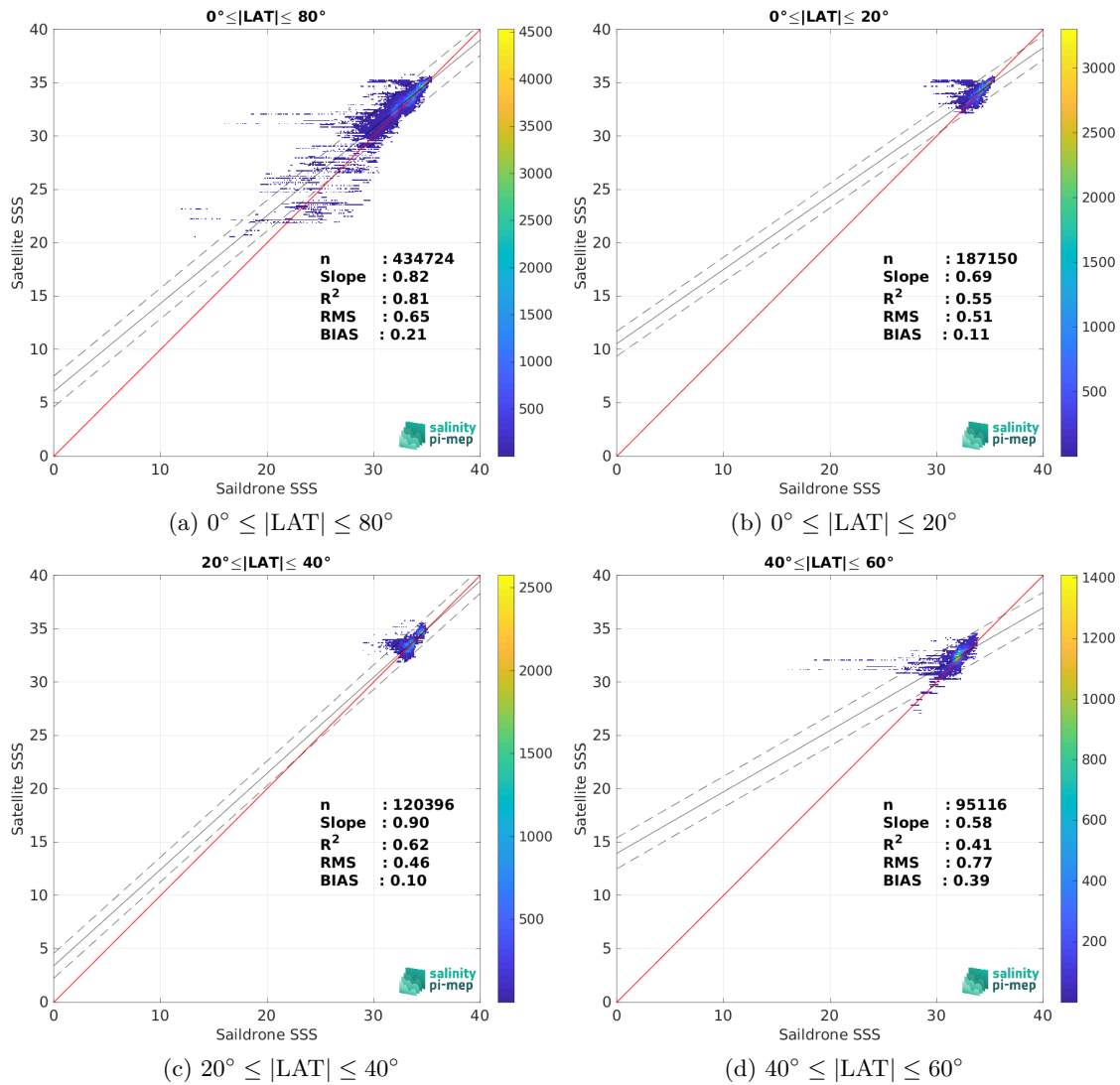
Figure 9: Contour maps of the concentration of SMAP SSS L3 v5 - 8-Day running (RSS) SSS (y-axis) versus Sairdrone SSS (x-axis) at match-up pairs for different latitude bands. For each plot, the red line shows x=y . The black thin and dashed lines indicate a linear fit through the data cloud and the \pm 95\% confidence levels, respectively. The number match-up pairs n , the slope and R^2 coefficient of the linear fit, the root mean square (RMS) and the mean bias between satellite and in situ data are indicated for each latitude band in each plots.
