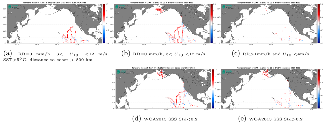
Figure 12: Temporal mean gridded over spatial boxes of size 1^\circ \times 1^\circ of \Delta SSS (SMAP SSS L3 v5 - 8-Day running (RSS) - Sairdron) for 5 different subdatasets corresponding to:RR=0 mm/h, 3 < U_{10} < 12 m/s, SST > 5^\circ C , distance to coast > 800 km (a), RR=0 mm/h, 3 < U_{10} < 12 m/s (b), RR>1mm/h and U_{10} < 4 m/s (c), WOA2013 SSS Std<0.2 (d), WOA2013 SSS Std>0.2 (e).
