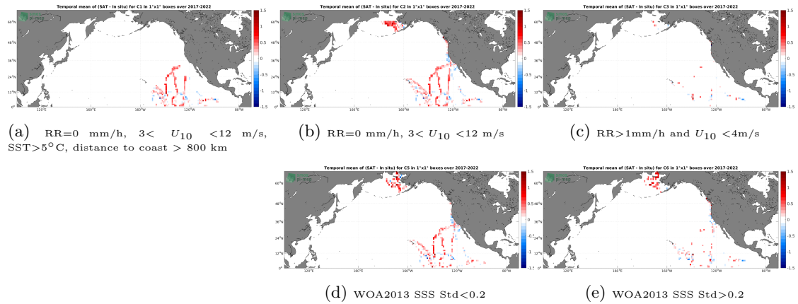
Figure 12: Temporal mean gridded over spatial boxes of size 1^\circ \times 1^\circ of \Delta SSS (SMAP SSS L3 v5 - 8-Day running (RSS) - Sairdrone) for 5 different subdatasets corresponding to:RR=0 mm/h, 3 < U_{10} < 12 m/s, SST > 5^\circ C , distance to coast > 800 km (a), RR=0 mm/h, 3 < U_{10} < 12 m/s (b), RR >1 mm/h and U_{10} < 4 m/s (c), WOA2013 SSS Std <0.2 (d), WOA2013 SSS Std >0.2 (e).
