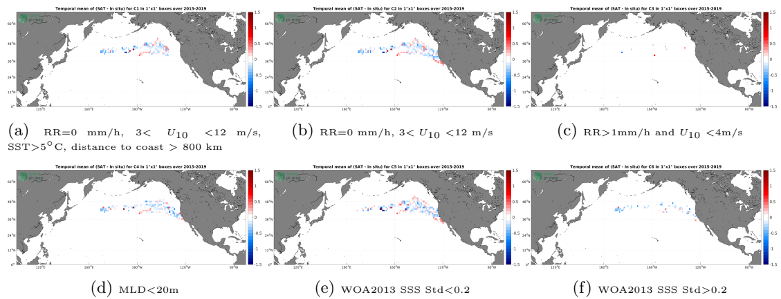
Figure 12: Temporal mean gridded over spatial boxes of size 1^\circ \times 1^\circ of \Delta SSS (SMAP SSS L3 v5 - 8-Day running (RSS) - Marine mammals) for 6 different subdatasets corresponding to:RR=0 mm/h, 3 < U_{10} < 12 m/s, SST >5^\circ C, distance to coast > 800 km (a), RR=0 mm/h, 3 < U_{10} < 12 m/s (b), RR >1 mm/h and U_{10} < 4 m/s (c),MLD <20 m (d),WOA2013 SSS Std <0.2 (e),WOA2013 SSS Std >0.2 (f).
