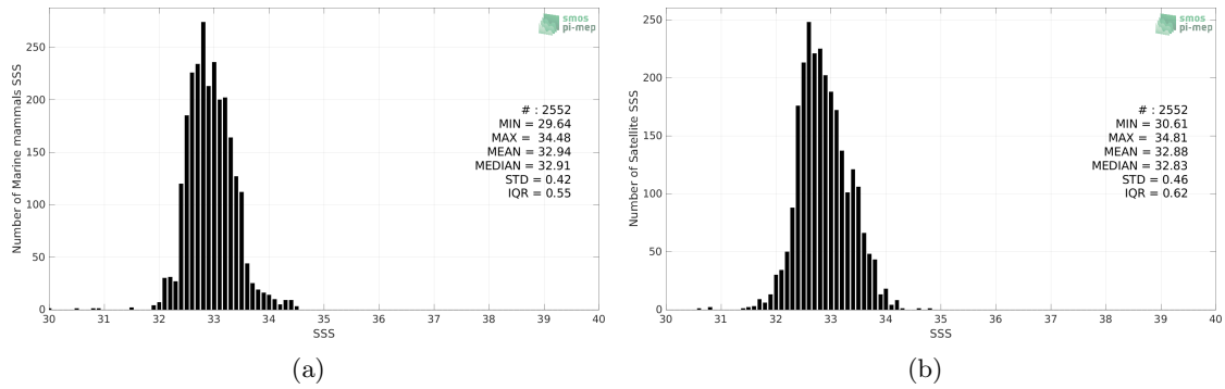
Figure 2: Histograms of SSS from Marine mammals (a) and SMAP SSS L3 v5 - 8-Day running (RSS) (b) considering all match-up pairs per bins of 0.1 over the North Pacific Ocean Pi-MEP region and for the full satellite product period.
