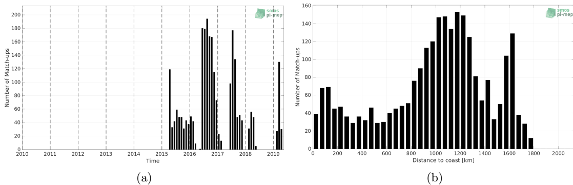
Figure 1: Number of match-ups between Marine mammals and SMAP SSS L3 v5 - 8-Day running (RSS) SSS as a function of time (a) and as function of the distance to coast (b) over the North Pacific Ocean Pi-MEP region and for the full satellite product period.
