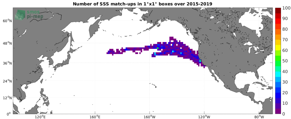
Figure 4: Number of SSS match-ups between Marine mammals SSS and the SMAP SSS L3 v5 - 8-Day running (RSS) SSS product for the North Pacific Ocean Pi-MEP region over 1^\circ \times 1^\circ boxes and for the full satellite product period.
