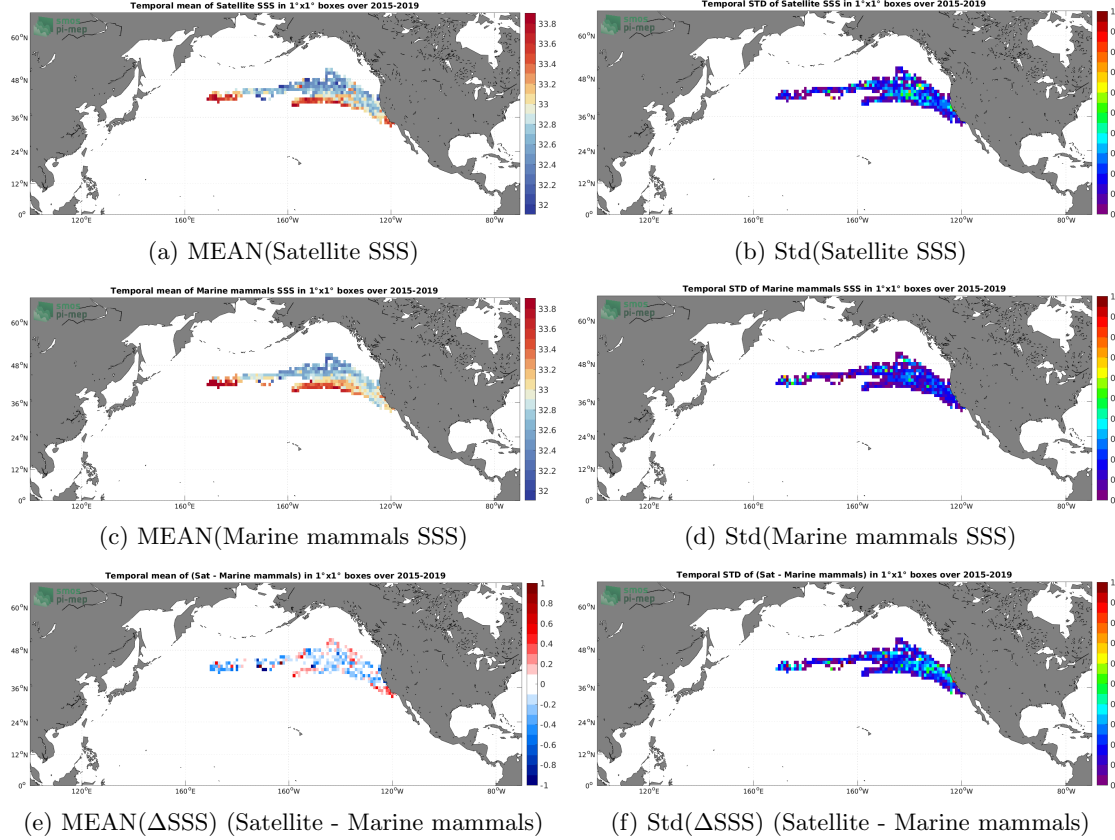
Figure 6: Temporal mean (left) and Std (right) of SSS from SMAP SSS L3 v5 - 8-Day running (RSS) (top), Marine mammals (middle), and of \Delta SSS (Satellite - Marine mammals). Only match-up pairs are used to generate these maps.
