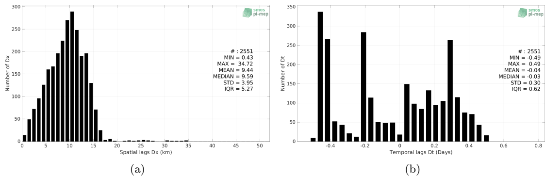
Figure 5: Histograms of the spatial (a) and temporal (b) lags between the location/time of the Marine mammals measurement and the date of the corresponding SMAP SSS L3 v5 - 8-Day running (RSS) SSS pixel.
