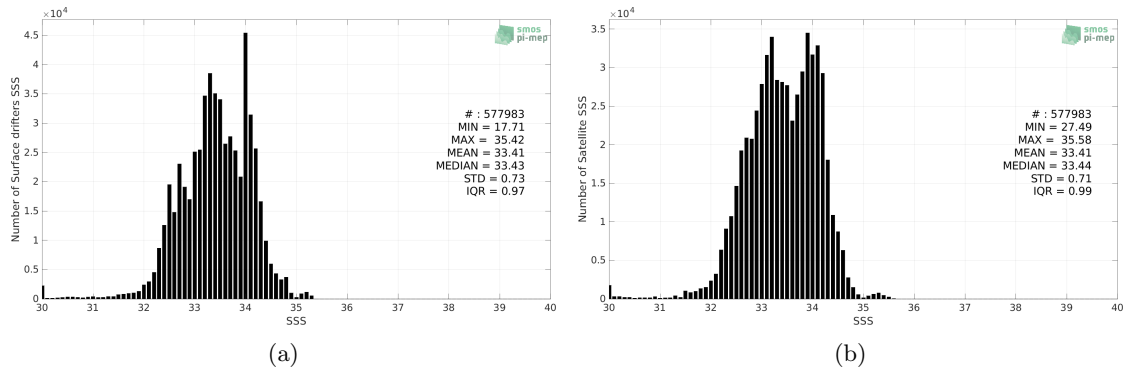
Figure 2: Histograms of SSS from Surface drifters (a) and SMAP SSS L3 v5 - 8-Day running (RSS) (b) considering all match-up pairs per bins of 0.1 over the North Pacific Ocean Pi-MEP region and for the full satellite product period.
