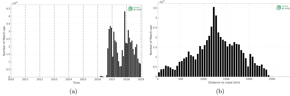
Figure 1: Number of match-ups between Surface drifters and SMAP SSS L3 v5 - 8-Day running (RSS) SSS as a function of time (a) and as function of the distance to coast (b) over the North Pacific Ocean Pi-MEP region and for the full satellite product period.
