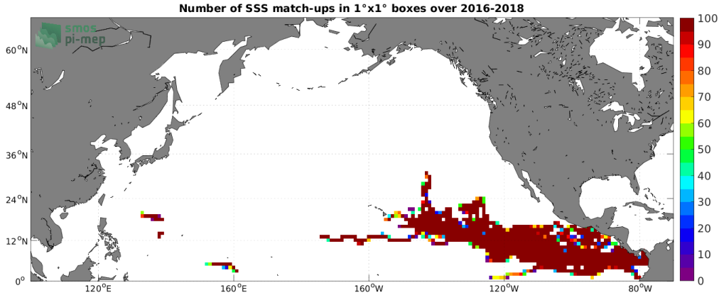
Figure 3: Number of SSS match-ups between Surface drifters SSS and the SMAP SSS L3 v5 - 8-Day running (RSS) SSS product for the North Pacific Ocean Pi-MEP region over 1^\circ \times 1^\circ boxes and for the full satellite product period.
