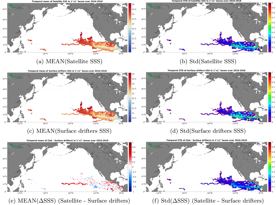
Figure 5: Temporal mean (left) and Std (right) of SSS from SMAP SSS L3 v5 - 8-Day running (RSS) (top), Surface drifters (middle), and of \Delta SSS (Satellite - Surface drifters). Only match-up pairs are used to generate these maps.
