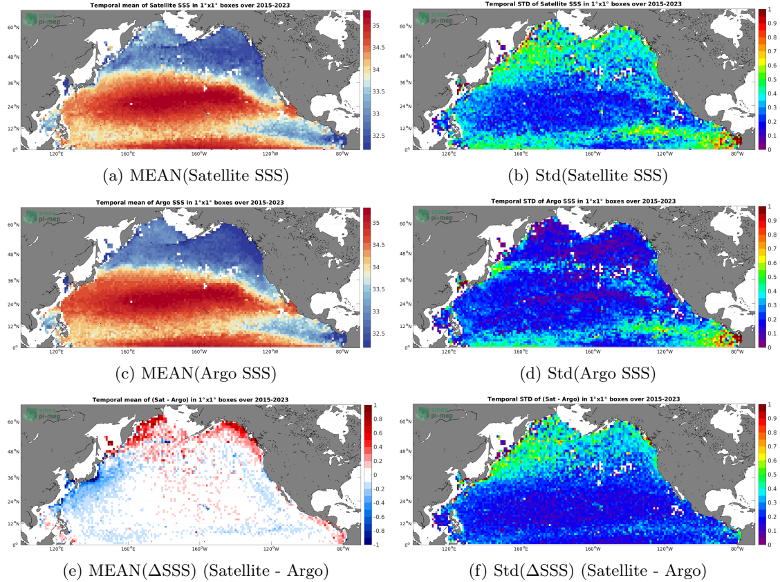
Figure 6: Temporal mean (left) and Std (right) of SSS from SMAP SSS L3 v5 - 8-Day running (RSS) (top), Argo (middle), and of \Delta\text{SSS} (Satellite - Argo). Only match-up pairs are used to generate these maps.
