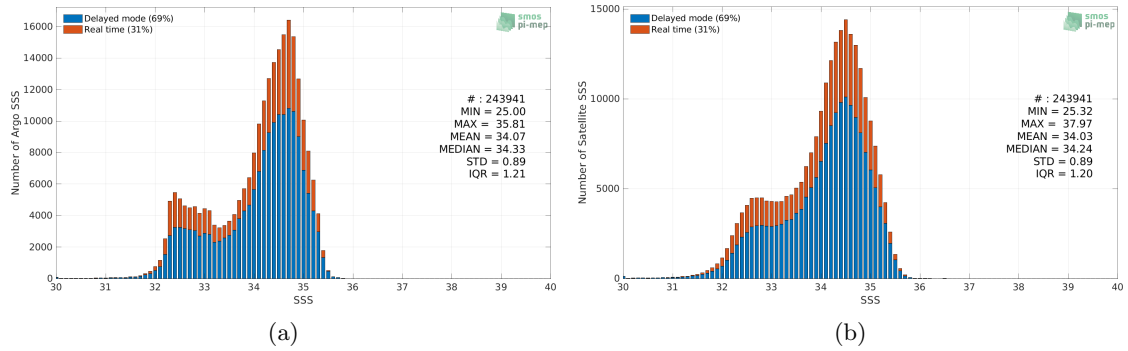
Figure 2: Histograms of SSS from Argo (a) and SMAP SSS L3 v5 - 8-Day running (RSS) (b) considering all match-up pairs per bins of 0.1 over the North Pacific Ocean Pi-MEP region and for the full satellite product period.
