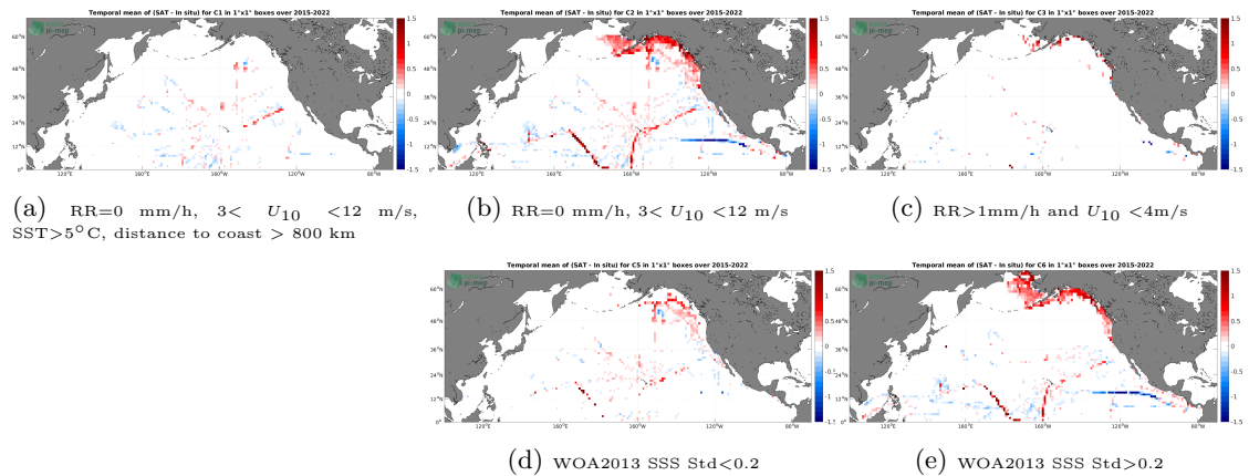
Figure 12: Temporal mean gridded over spatial boxes of size 1^\circ \times 1^\circ of \Delta SSS (SMAP SSS L3 v5 - Monthly (RSS) - TSG (SAMOS)) for 5 different subdatasets corresponding to:RR=0 mm/h, 3 < U_{10} < 12 m/s, SST > 5^\circ C , distance to coast > 800 km (a), RR=0 mm/h, 3 < U_{10} < 12 m/s (b), RR >1 mm/h and U_{10} < 4 m/s (c), WOA2013 SSS Std <0.2 (d), WOA2013 SSS Std >0.2 (e).
