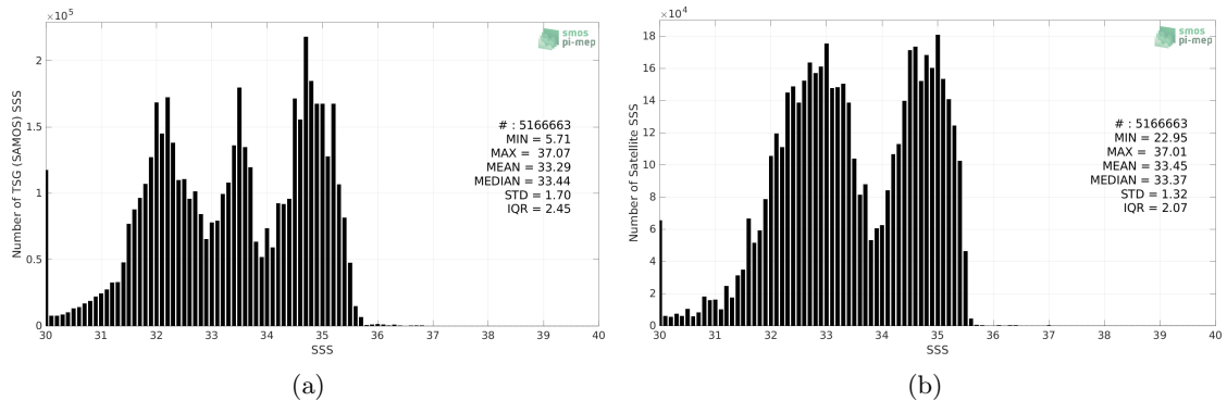
Figure 2: Histograms of SSS from TSG (SAMOS) (a) and SMAP SSS L3 v5 - Monthly (RSS) (b) considering all match-up pairs per bins of 0.1 over the North Pacific Ocean Pi-MEP region and for the full satellite product period.
