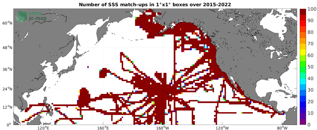
Figure 4: Number of SSS match-ups between TSG (SAMOS) SSS and the SMAP SSS L3 v5 - Monthly (RSS) SSS product for the North Pacific Ocean Pi-MEP region over 1^\circ \times 1^\circ boxes and for the full satellite product period.
