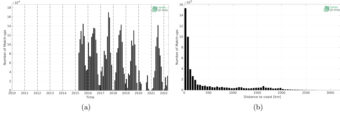
Figure 1: Number of match-ups between TSG (SAMOS) and SMAP SSS L3 v5 - Monthly (RSS) SSS as a function of time (a) and as function of the distance to coast (b) over the North Pacific Ocean Pi-MEP region and for the full satellite product period.
