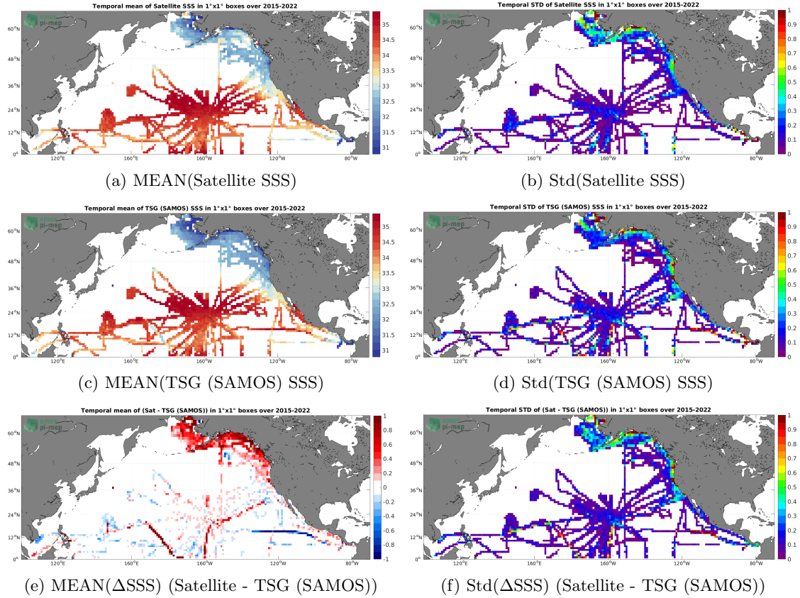
Figure 6: Temporal mean (left) and Std (right) of SSS from SMAP SSS L3 v5 - Monthly (RSS) (top), TSG (SAMOS) (middle), and of \Delta SSS (Satellite - TSG (SAMOS)). Only match-up pairs are used to generate these maps.
