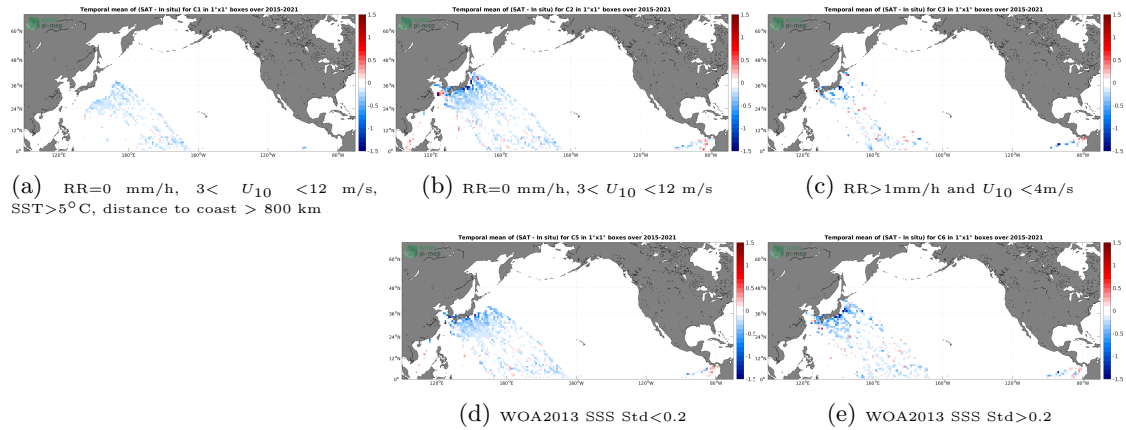
Figure 12: Temporal mean gridded over spatial boxes of size 1^\circ \times 1^\circ of \Delta SSS (SMAP SSS L3 v5 - Monthly (RSS) - TSG (LEGOS-DM)) for 5 different subdatasets corresponding to: RR=0 mm/h, 3 < U_{10} < 12 m/s, SST > 5^\circ C , distance to coast > 800 km (a), RR=0 mm/h, 3 < U_{10} < 12 m/s (b), RR>1mm/h and U_{10} < 4 m/s (c), WOA2013 SSS Std<0.2 (d), WOA2013 SSS Std>0.2 (e).
