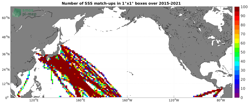
Figure 4: Number of SSS match-ups between TSG (LEGOS-DM) SSS and the SMAP SSS L3 v5 - Monthly (RSS) SSS product for the North Pacific Ocean Pi-MEP region over 1^\circ \times 1^\circ boxes and for the full satellite product period.
