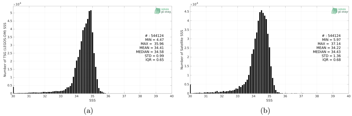
Figure 2: Histograms of SSS from TSG (LEGOS-DM) (a) and SMAP SSS L3 v5 - Monthly (RSS) (b) considering all match-up pairs per bins of 0.1 over the North Pacific Ocean Pi-MEP region and for the full satellite product period.
