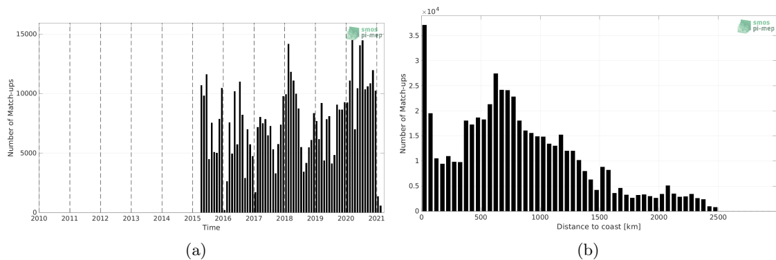
Figure 1: Number of match-ups between TSG (LEGOS-DM) and SMAP SSS L3 v5 - Monthly (RSS) SSS as a function of time (a) and as function of the distance to coast (b) over the North Pacific Ocean Pi-MEP region and for the full satellite product period.
