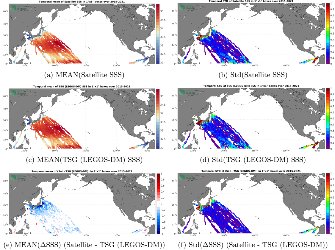
Figure 6: Temporal mean (left) and Std (right) of SSS from SMAP SSS L3 v5 - Monthly (RSS) (top), TSG (LEGOS-DM) (middle), and of \Delta\text{SSS} (Satellite - TSG (LEGOS-DM)). Only match-up pairs are used to generate these maps.
