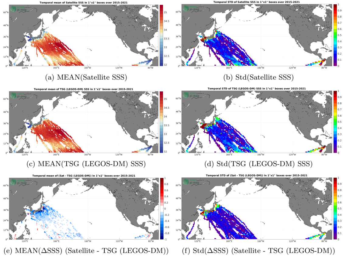
Figure 6: Temporal mean (left) and Std (right) of SSS from SMAP SSS L3 v5 - Monthly (RSS) (top), TSG (LEGOS-DM) (middle), and of \Delta SSS (Satellite - TSG (LEGOS-DM)). Only match-up pairs are used to generate these maps.
