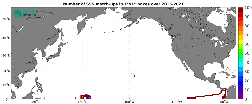
Figure 4: Number of SSS match-ups between TSG (GOSUD-Research-vessel) SSS and the SMAP SSS L3 v5 - Monthly (RSS) SSS product for the North Pacific Ocean Pi-MEP region over 1^\circ \times 1^\circ boxes and for the full satellite product period.
