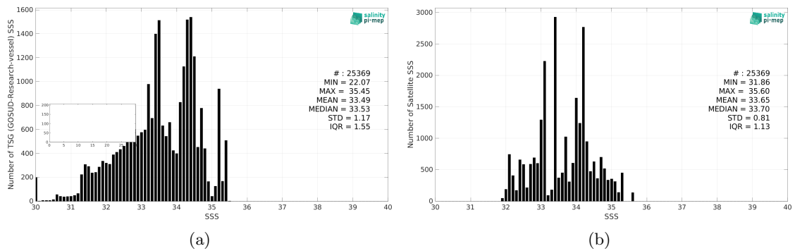
Figure 2: Histograms of SSS from TSG (GOSUD-Research-vessel) (a) and SMAP SSS L3 v5 - Monthly (RSS) (b) considering all match-up pairs per bins of 0.1 over the North Pacific Ocean Pi-MEP region and for the full satellite product period.
