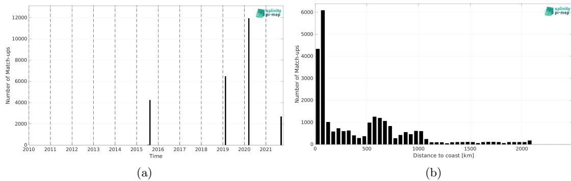
Figure 1: Number of match-ups between TSG (GOSUD-Research-vessel) and SMAP SSS L3 v5 - Monthly (RSS) SSS as a function of time (a) and as function of the distance to coast (b) over the North Pacific Ocean Pi-MEP region and for the full satellite product period.
