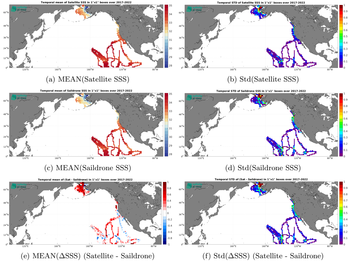
Figure 6: Temporal mean (left) and Std (right) of SSS from SMAP SSS L3 v5 - Monthly (RSS) (top), Saildrone (middle), and of \Delta\text{SSS} (Satellite - Saildrone). Only match-up pairs are used to generate these maps.
