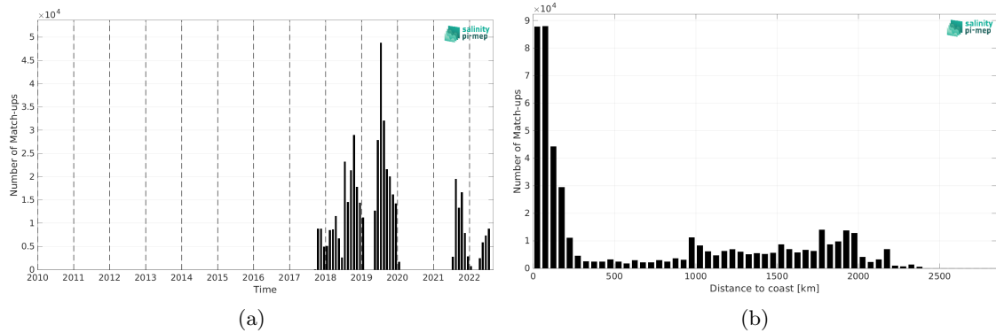
Figure 1: Number of match-ups between Sairdron and SMAP SSS L3 v5 - Monthly (RSS) SSS as a function of time (a) and as function of the distance to coast (b) over the North Pacific Ocean Pi-MEP region and for the full satellite product period.
