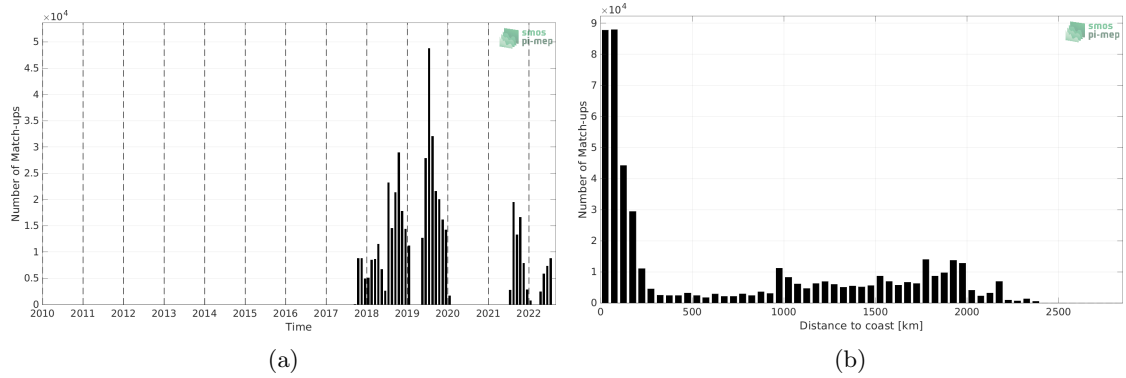
Figure 1: Number of match-ups between Sairdrone and SMAP SSS L3 v5 - Monthly (RSS) SSS as a function of time (a) and as function of the distance to coast (b) over the North Pacific Ocean Pi-MEP region and for the full satellite product period.
