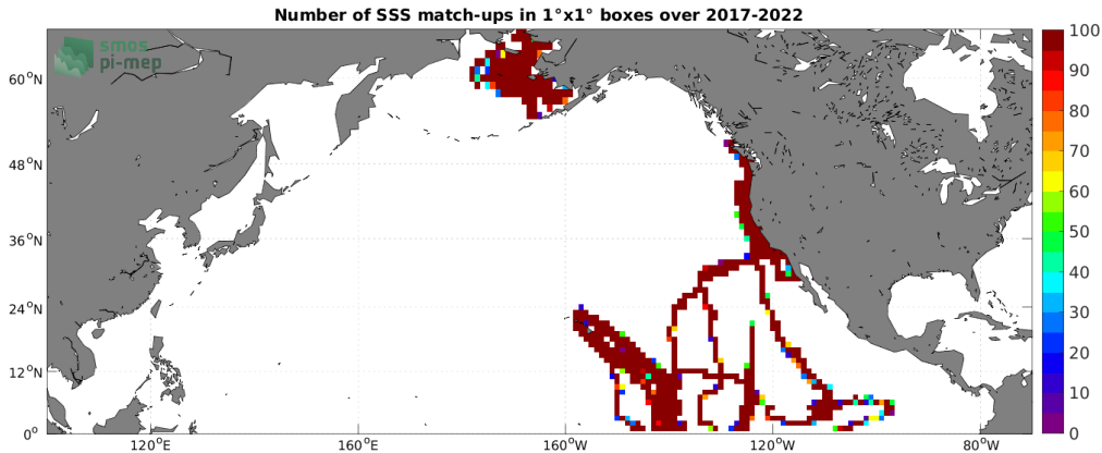
Figure 4: Number of SSS match-ups between Sairdrone SSS and the SMAP SSS L3 v5 - Monthly (RSS) SSS product for the North Pacific Ocean Pi-MEP region over 1^\circ \times 1^\circ boxes and for the full satellite product period.
