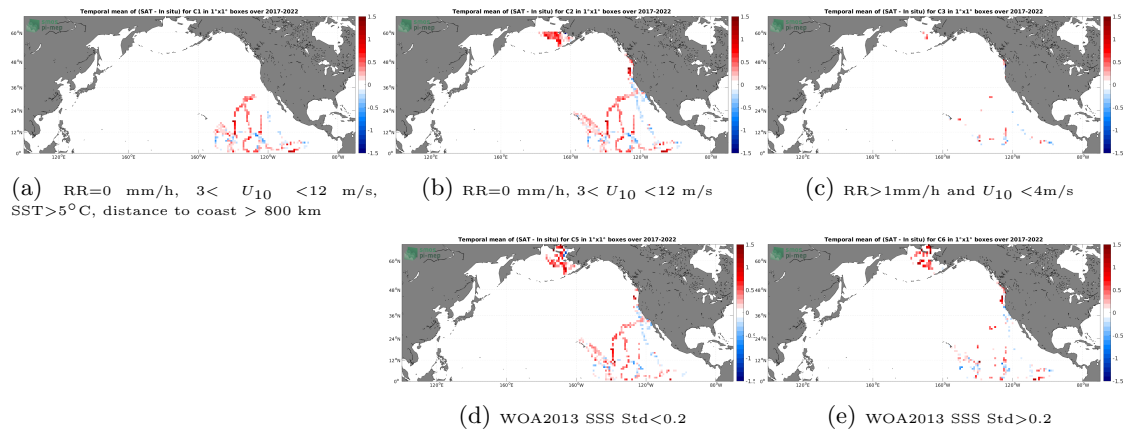
Figure 12: Temporal mean gridded over spatial boxes of size 1^\circ \times 1^\circ of \Delta SSS (SMAP SSS L3 v5 - Monthly (RSS) - Saildrone) for 5 different subdatasets corresponding to:RR=0 mm/h, 3 < U_{10} < 12 m/s, SST > 5^\circ C , distance to coast > 800 km (a), RR=0 mm/h, 3 < U_{10} < 12 m/s (b), RR>1mm/h and U_{10} < 4 m/s (c), WOA2013 SSS Std<0.2 (d), WOA2013 SSS Std>0.2 (e).
