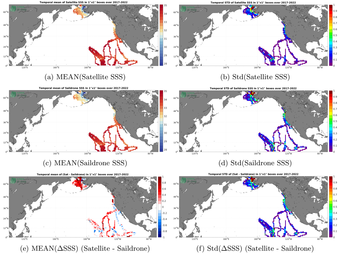
Figure 6: Temporal mean (left) and Std (right) of SSS from SMAP SSS L3 v5 - Monthly (RSS) (top), Sairdrone (middle), and of \Delta\text{SSS} (Satellite - Sairdrone). Only match-up pairs are used to generate these maps.
