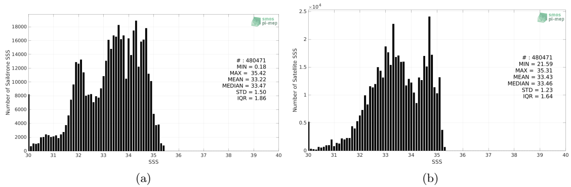
Figure 2: Histograms of SSS from Saildrone (a) and SMAP SSS L3 v5 - Monthly (RSS) (b) considering all match-up pairs per bins of 0.1 over the North Pacific Ocean Pi-MEP region and for the full satellite product period.
