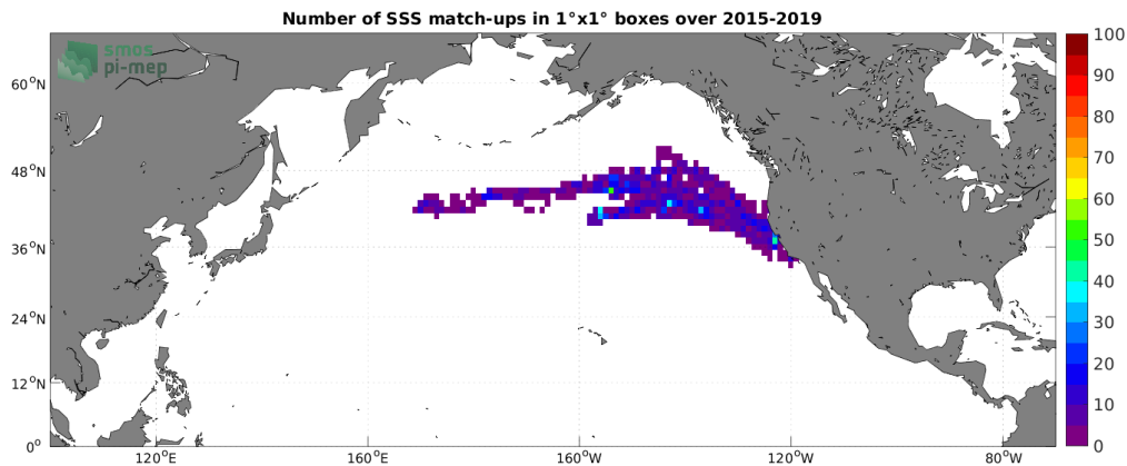
Figure 4: Number of SSS match-ups between Marine mammals SSS and the SMAP SSS L3 v5 - Monthly (RSS) SSS product for the North Pacific Ocean Pi-MEP region over 1^\circ \times 1^\circ boxes and for the full satellite product period.
