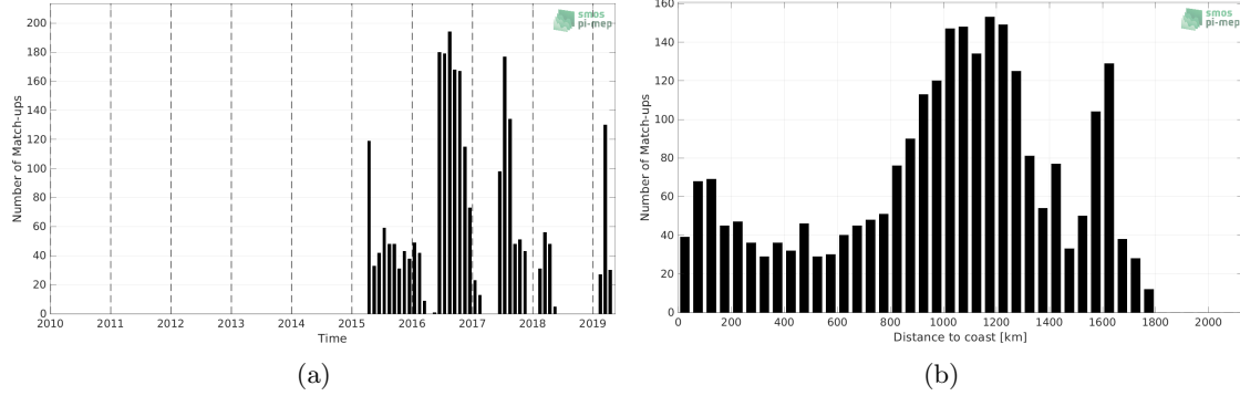
Figure 1: Number of match-ups between Marine mammals and SMAP SSS L3 v5 - Monthly (RSS) SSS as a function of time (a) and as function of the distance to coast (b) over the North Pacific Ocean Pi-MEP region and for the full satellite product period.
