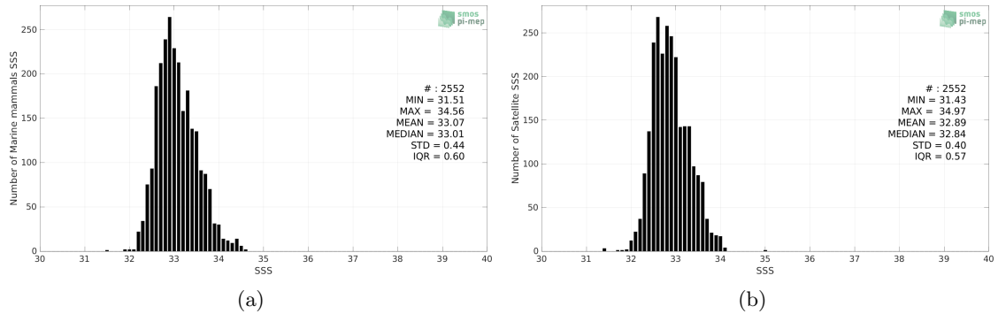
Figure 2: Histograms of SSS from Marine mammals (a) and SMAP SSS L3 v5 - Monthly (RSS) (b) considering all match-up pairs per bins of 0.1 over the North Pacific Ocean Pi-MEP region and for the full satellite product period.
