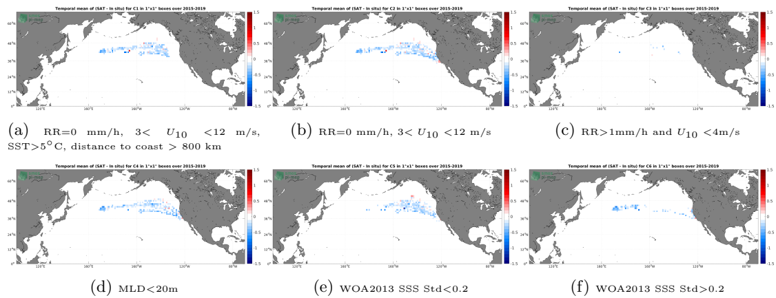
Figure 12: Temporal mean gridded over spatial boxes of size 1^\circ \times 1^\circ of \Delta SSS (SMAP SSS L3 v5 - Monthly (RSS) - Marine mammals) for 6 different subdatasets corresponding to:RR=0 mm/h, 3 < U_{10} < 12 m/s, SST >5^\circ\text{C} , distance to coast > 800 km (a), RR=0 mm/h, 3 < U_{10} < 12 m/s (b), RR >1 mm/h and U_{10} < 4 m/s (c),MLD <20 m (d),WOA2013 SSS Std <0.2 (e),WOA2013 SSS Std >0.2 (f).
