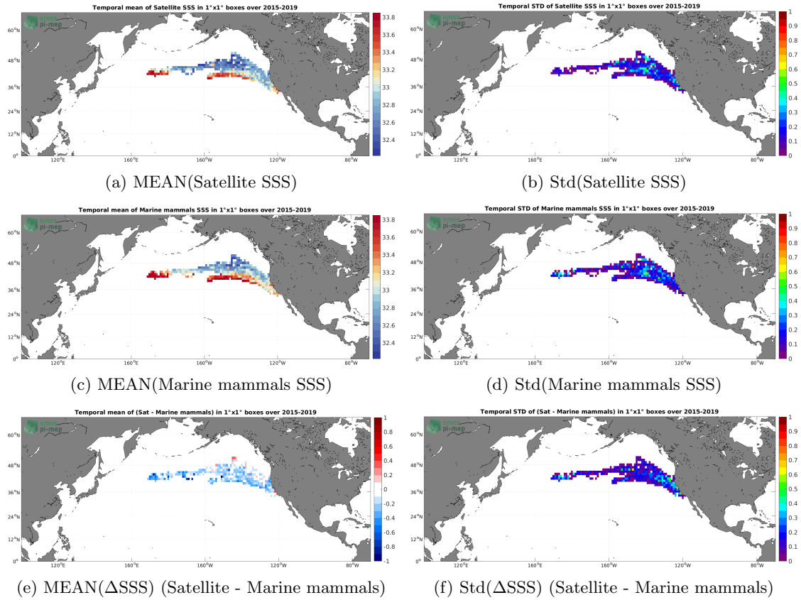
Figure 6: Temporal mean (left) and Std (right) of SSS from SMAP SSS L3 v5 - Monthly (RSS) (top), Marine mammals (middle), and of \Delta SSS (Satellite - Marine mammals). Only match-up pairs are used to generate these maps.
