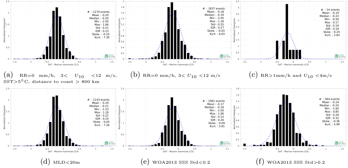
Figure 13: Normalized histogram of \Delta SSS (SMAP SSS L3 v5 - Monthly (RSS) - Marine mammals) for 6 different subdatasets corresponding to: RR=0 mm/h, 3 < U_{10} < 12 m/s, SST > 5°C, distance to coast > 800 km (a), RR=0 mm/h, 3 < U_{10} < 12 m/s (b), RR > 1mm/h and U_{10} < 4 m/s (c), MLD < 20m (d), WOA2013 SSS Std < 0.2 (e), WOA2013 SSS Std > 0.2 (f).
