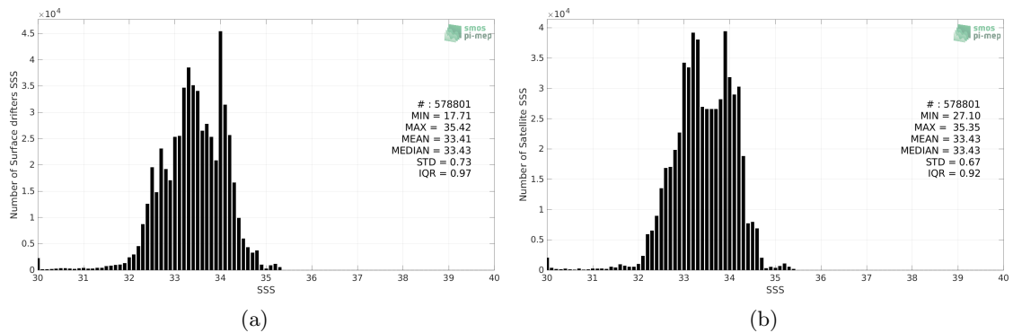
Figure 2: Histograms of SSS from Surface drifters (a) and SMAP SSS L3 v5 - Monthly (RSS) (b) considering all match-up pairs per bins of 0.1 over the North Pacific Ocean Pi-MEP region and for the full satellite product period.
