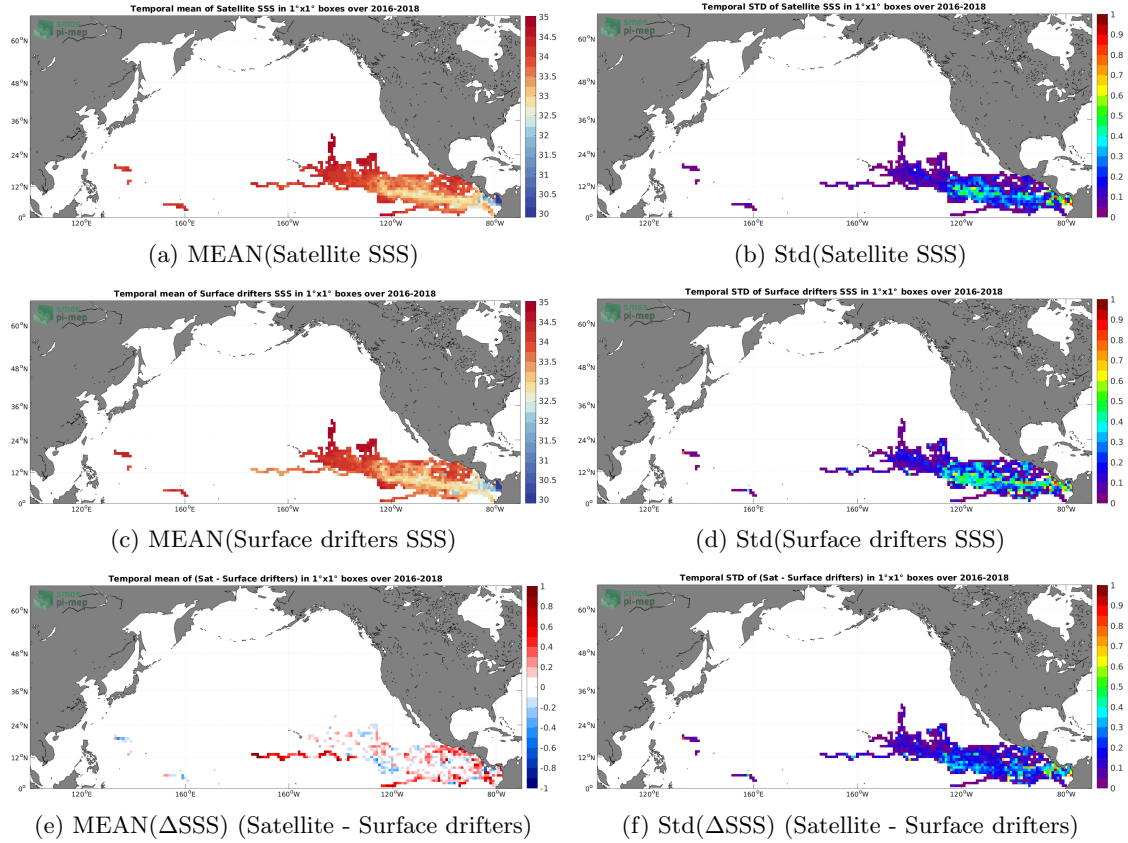
Figure 5: Temporal mean (left) and Std (right) of SSS from SMAP SSS L3 v5 - Monthly (RSS) (top), Surface drifters (middle), and of \Delta SSS (Satellite - Surface drifters). Only match-up pairs are used to generate these maps.
