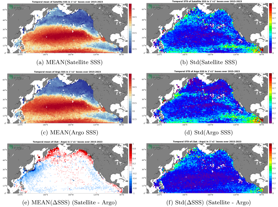
Figure 6: Temporal mean (left) and Std (right) of SSS from SMAP SSS L3 v5 - Monthly (RSS) (top), Argo (middle), and of \Delta\text{SSS} (Satellite - Argo). Only match-up pairs are used to generate these maps.
