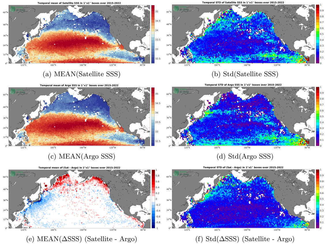
Figure 6: Temporal mean (left) and Std (right) of SSS from SMAP SSS L3 v5 - Monthly (RSS) (top), Argo (middle), and of \Delta SSS (Satellite - Argo). Only match-up pairs are used to generate these maps.
