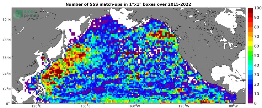
Figure 4: Number of SSS match-ups between Argo SSS and the SMAP SSS L3 v5 - Monthly (RSS) SSS product for the North Pacific Ocean Pi-MEP region over 1^\circ \times 1^\circ boxes and for the full satellite product period.
