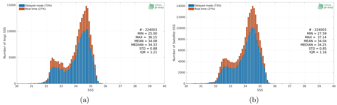
Figure 2: Histograms of SSS from Argo (a) and SMAP SSS L3 v5 - Monthly (RSS) (b) considering all match-up pairs per bins of 0.1 over the North Pacific Ocean Pi-MEP region and for the full satellite product period.
