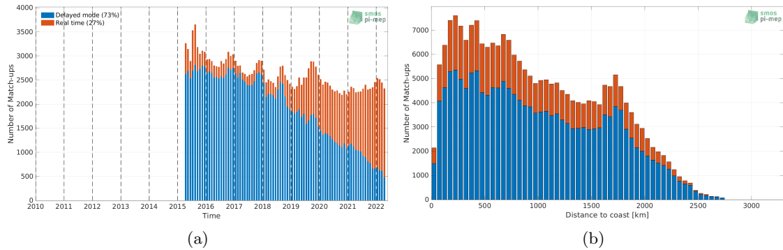
Figure 1: Number of match-ups between Argo and SMAP SSS L3 v5 - Monthly (RSS) SSS as a function of time (a) and as function of the distance to coast (b) over the North Pacific Ocean Pi-MEP region and for the full satellite product period.
