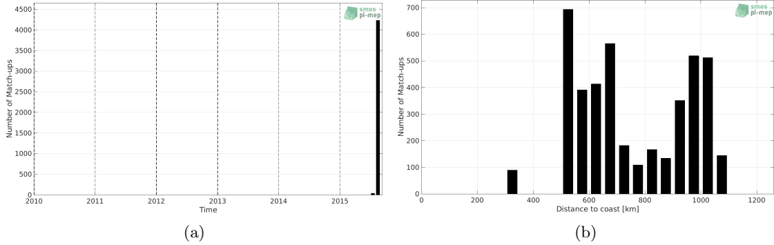
Figure 1: Number of match-ups between TSG (GOSUD-Research-vessel) and SMAP SSS L3 v4 - 8-Day running (RSS) SSS as a function of time (a) and as function of the distance to coast (b) over the North Pacific Ocean Pi-MEP region and for the full satellite product period.
