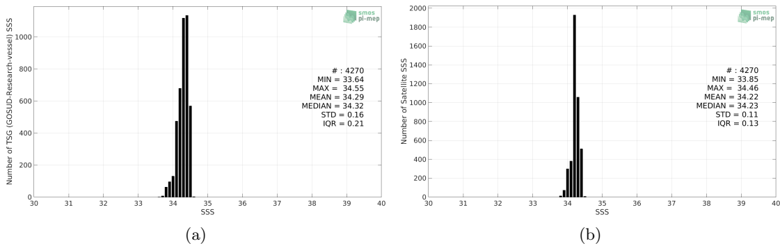
Figure 2: Histograms of SSS from TSG (GOSUD-Research-vessel) (a) and SMAP SSS L3 v4 - 8-Day running (RSS) (b) considering all match-up pairs per bins of 0.1 over the North Pacific Ocean Pi-MEP region and for the full satellite product period.
